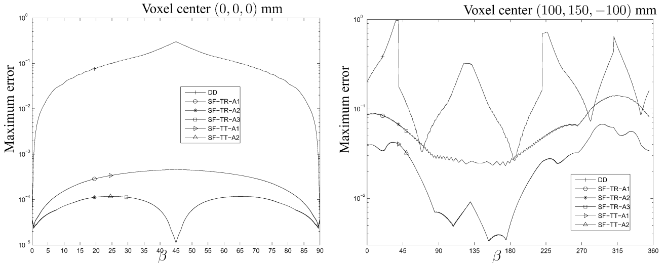
Fig. 3. Maximum error comparison between the forward DD, SF-TR, and SF-TT projector for a voxel centered at the origin (left) and a voxel centered at (100, 150, -100) mm (right).
