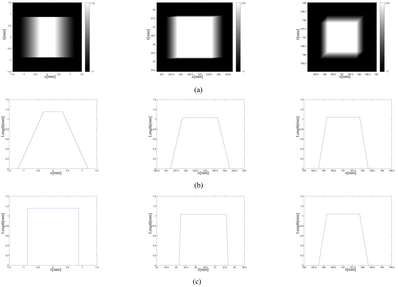
Fig. 2. Exact footprint functions q(s, t; \beta; \vec{n}) and their profiles for 1 \text{ mm}^3 voxels centered at the origin (left), (100, 150, 15) \text{ mm} (center), and (93, 93, 93) \text{ mm} (right). (a) True footprint. (b) Profile in s . (c) Profile in t .
