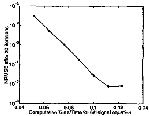
Fig. 5. NRMSE after 20 iterations vs. computation time for L = 4, \dots, 10 for the ideal min-max interpolator. Time is given as a percentage of the computation time to evaluate the full signal equation (1).
