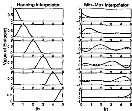
Fig. 3. Real (solid lines) and imaginary (dashed lines) parts of interpolators using L = 6 for the Hanning and min-max interpolators.
