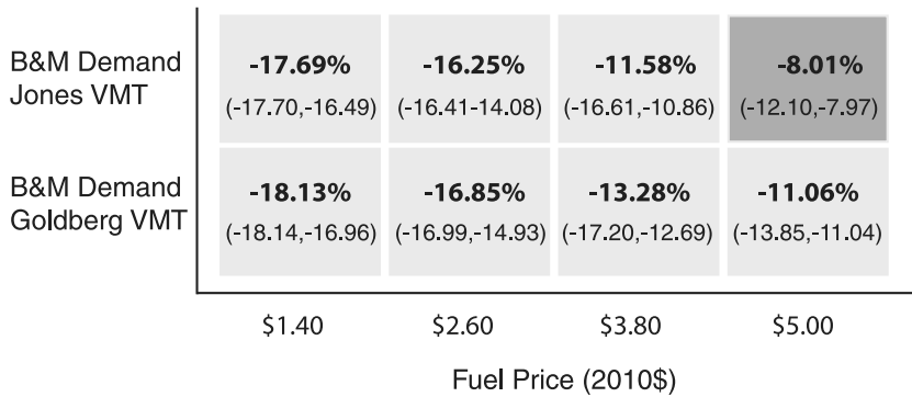
Figure 5 Greenhouse gas emission results evaluated over scenarios of fuel price parameter and vehicle miles travelled (VMT) model. The shade of the scenario indicates acceptance (light), rejection (dark; none shown in this figure), or neither (mid-shade) of the case-study hypothesis. Confidence intervals are shown in parentheses. B&M Demand = use of the demand model published by Boyd and Mellman in 1980.
