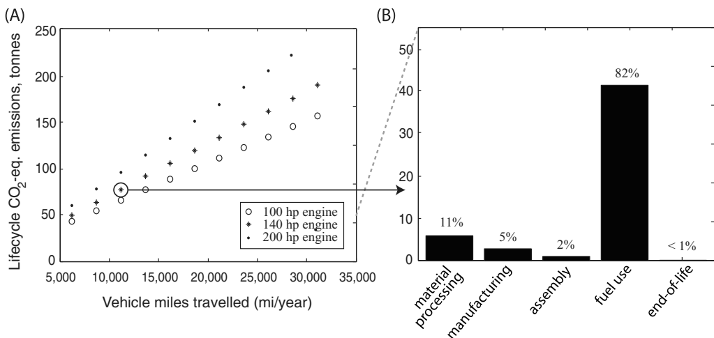
Figure 2 (A) Effect of varying vehicle miles travelled on life cycle equivalent carbon dioxide emissions (CO 2 -eq.) using an attributional life cycle assessment approach. (B) Emissions from the 140-horsepower (hp) vehicle with 11,200 vehicle miles travelled, broken down by life cycle stage. mi = miles.
