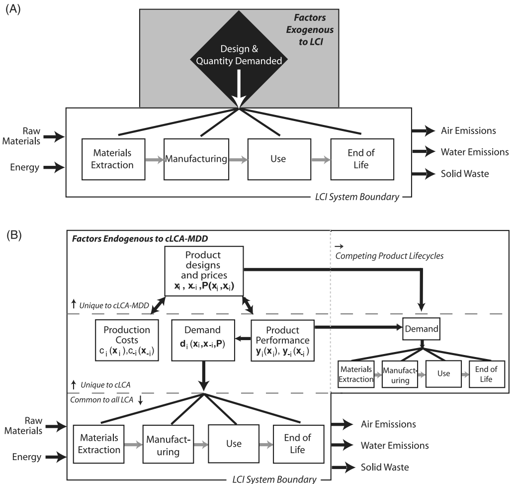
Figure 1 Life cycle inventory (LCI) system boundaries according to (A) an attributional life cycle assessment approach and (B) a consequential life cycle assessment with market-driven demand approach. x_i , protagonist design variables; x_{-i} , competitor design variables; P , prices of all products; c_i and c_{-i} , the production costs of the protagonist and competitor products, respectively; y_i and y_{-i} , product attributes that consumers care about of the protagonist and competitor products, respectively; d_i , demand for the protagonist products.
