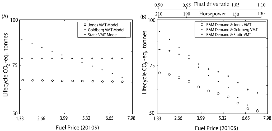
Figure 3 Life cycle greenhouse gas emissions as a function of fuel price according to (A) a consequential life cycle assessment approach, whereby vehicle design is fixed but vehicle miles travelled (VMT) is a function of fuel price, and (B) a consequential life cycle assessment with market-driven demand approach, whereby both vehicle miles travelled and equilibrium engine horsepower are dependent on fuel price. CO 2 -eq. = carbon dioxide equivalent; B&M Demand = use of the demand model published by Boyd and Mellman in 1980.
