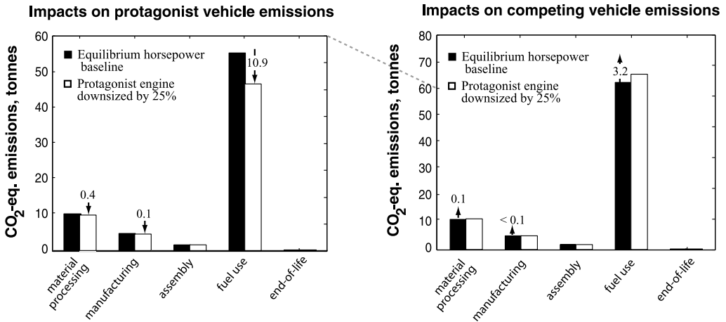
Figure 4 Changes in life cycle greenhouse gas emissions associated with a mid-size vehicle (the protagonist) as a result of the decision to downsize the vehicle’s engine. CO 2 -eq. = carbon dioxide equivalent.
