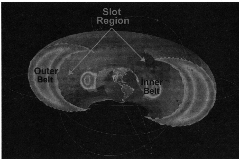
Fig. 1. Energetic electron flux, showing the inner and outer radiation belts. Warm colors indicate high flux intensity, while cool colors indicate low flux intensity values. Also shown are the orbits of three Global Positioning System (GPS) spacecraft and one geosynchronous spacecraft (the equatorial orbit). Image from AF-GEOSpace. Original color image appears at the back of this volume.
