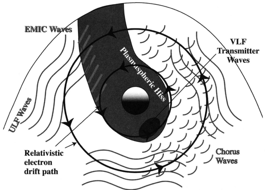
Fig. 3. A schematic of how relativistic electron paths pass through various plasma wave regions over the course of a drift period. The inner drift path will experience mostly loss processes, while the outer drift path encounters a mixture of acceleration and loss processes. Adapted from Summers et al. [1998]. Original color image appears at the back of this volume.
