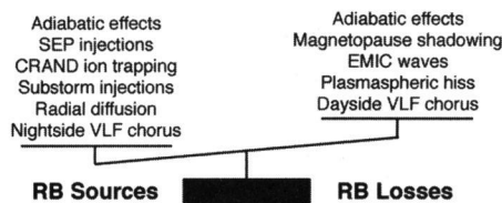
Fig. 2. Scale weighing the plasma source and loss mechanisms within the radiation belts. In this example, the scale is tipped, indicating a scenario where plasma is enhanced within the radiation belts. SEP stands for solar energetic particle; CRAND is cosmic ray albedo neutron decay; EMIC is electromagnetic ion cyclotron; and VLF is very low frequency.
