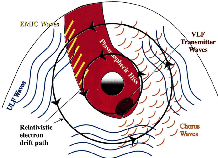
Fig. 3. A schematic of how relativistic electron paths pass through various plasma wave regions over the course of a drift period. The inner drift path will experience mostly loss processes, while the outer drift path encounters a mixture of acceleration and loss processes. Adapted from Summers et al. [1998].
