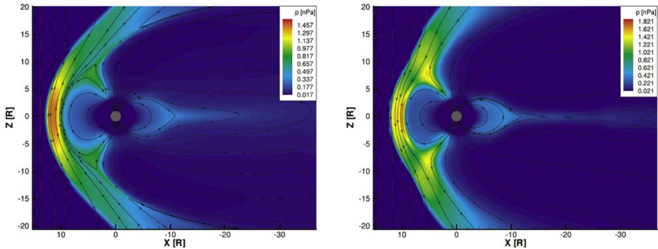
Figure 5. Pressure (color code) and the magnetic field lines in the north-south plane for (left) B_z = 5 nT, B_y = 1 nT and (right) B_z = -5 nT, B_y = 1 nT.
