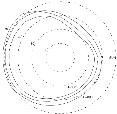
Figure 9. Open-closed field line boundary for B_y = 5 nT, B_z = 0 nT, n = 5 cm ^{-3} , and U = 300, 500, and 800 km/s.
