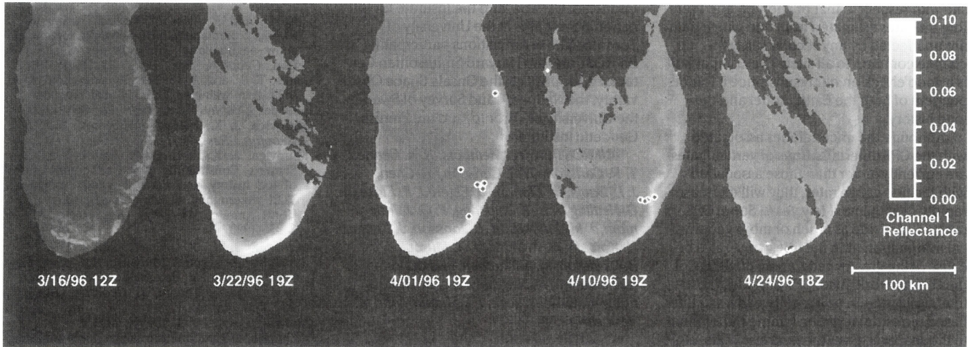
Fig. 1. Visible band satellite imagery of southern Lake Michigan. On March 16, the NOAA 12 (morning) AVHRR Channel 1 satellite image shows shore-fast ice along the eastern shore of the southern basin and large ice floes at the south end of the lake. After several days of warming temperatures and strong northerly winds, the March 22 NOAA 14 (afternoon) image shows the presence of a highly reflective plume that appears to originate along the southwestern shoreline and extend eastward along the southern shore. On April 1, a helicopter was used to collect five samples from the plume region and one sample and two conductivity-temperature-depth profiles were collected from ship further north. A subsequent set of four samples and conductivity-temperature-depth profiles were collected by small boat on April 10. Sampling locations are marked by crosses. By April 24, the plume extended along the entire eastern shore, but the intensity was considerably diminished. The majority of the western shoreline is composed of silty-clay bluffs [Jibson et al., 1994], while the southern shore is highly industrialized with extensive man-made features. The eastern shore is primarily sandy beaches backed by dunes. The pattern of sediment accumulation is highly asymmetric; the western and southern regions do not accumulate recent sediments, while the highest sediment accumulation in the lake is on the southeastern slope (coincident with the eddy features in the figure) and not in the deep central region. Clouds are masked out on the March 22, April 10, and April 24 images.
