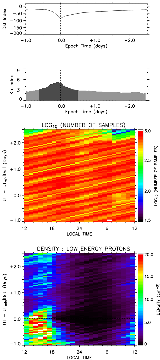
Figure 7. The averaged Dst and Kp indices, the sample statistics and the averaged LP density calculated as a function of storm epoch time, where the zero epoch occurs at minimum storm Dst .
