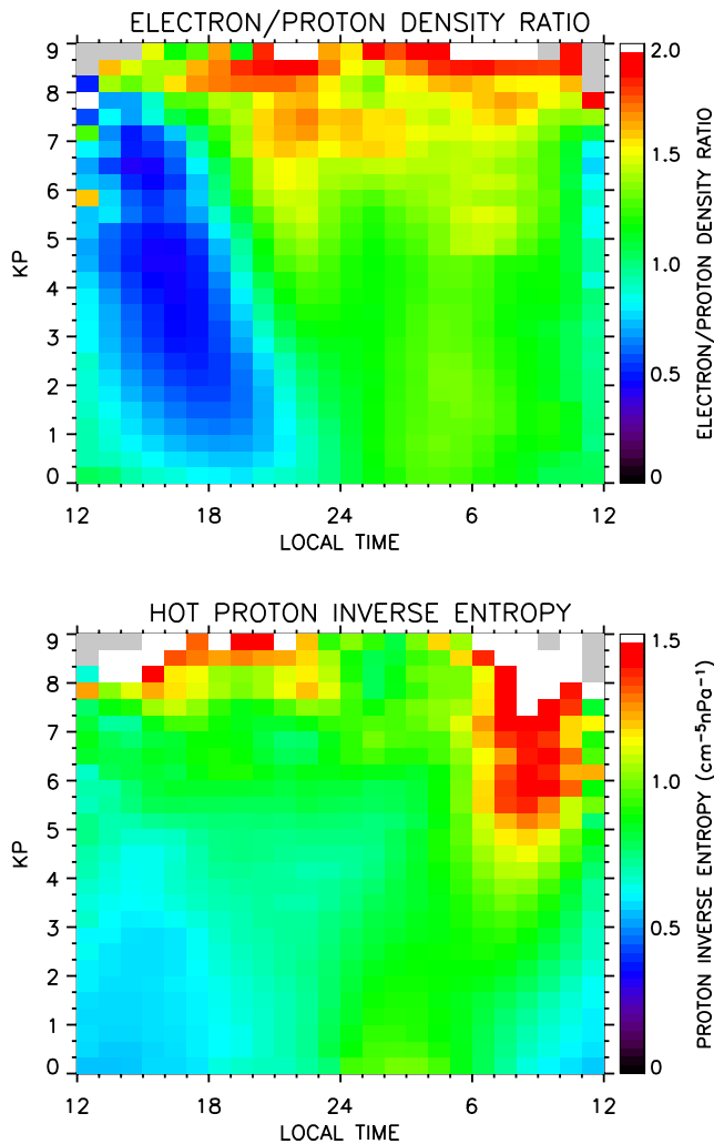
Figure 3. The averaged HE/HP density ratio and the HP inverse entropy calculated as a function of Kp index and local time for MPA data between 1990 and 2001, inclusive.
