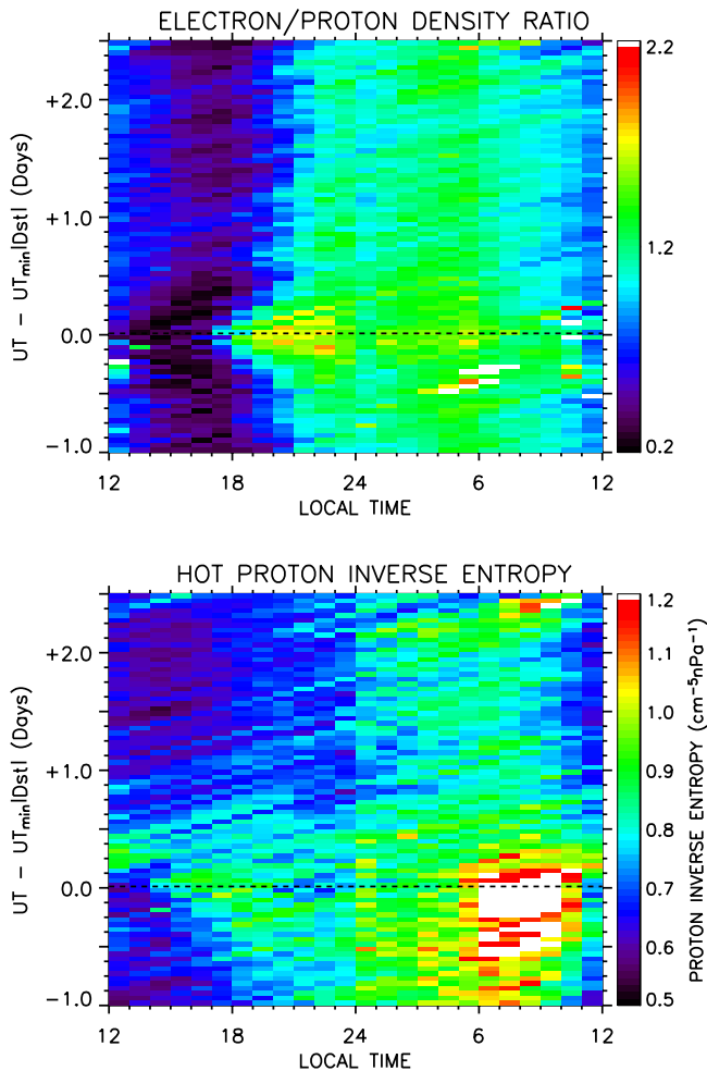
Figure 9. The averaged HE/HP density ratio and the HP inverse entropy calculated as a function of storm epoch time, where the zero epoch occurs at minimum storm Dst .
