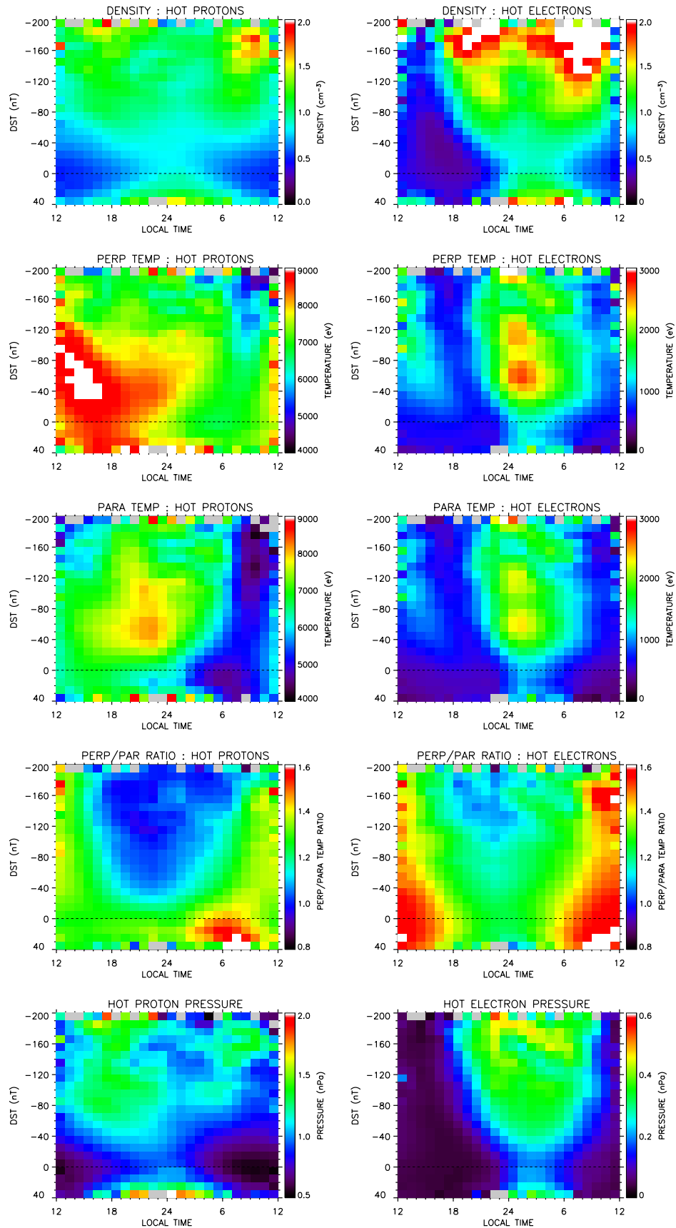
Figure 5. The averaged HP and HE density, parallel and perpendicular temperatures, the temperature anisotropies, and the pressures, calculated as a function of Dst index and local time for MPA data between 1990 and 2001, inclusive.
