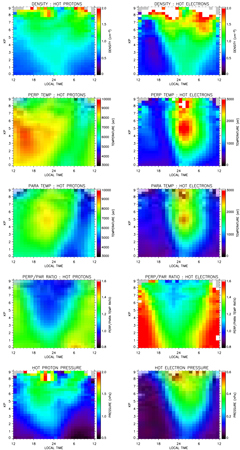
Figure 2. The averaged HP and HE density, parallel and perpendicular temperatures, the temperature anisotropies, and the pressures, calculated as a function of Kp index and local time for MPA data between 1990 and 2001, inclusive.
