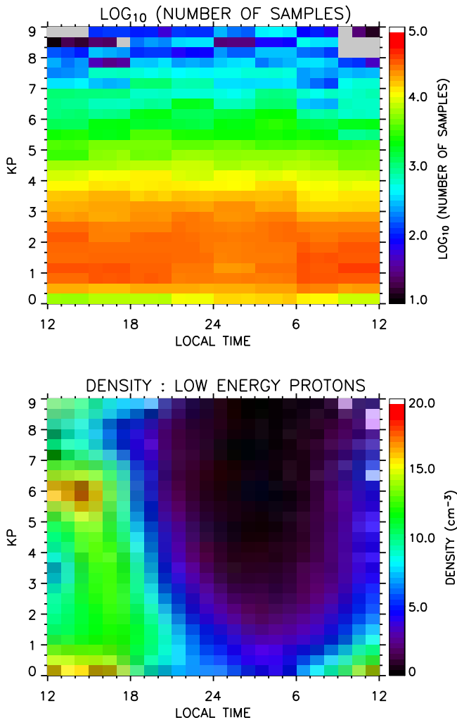
Figure 1. The sample statistics and the averaged LP density calculated as a function of Kp index and local time for MPA data between 1990 and 2001, inclusive.
