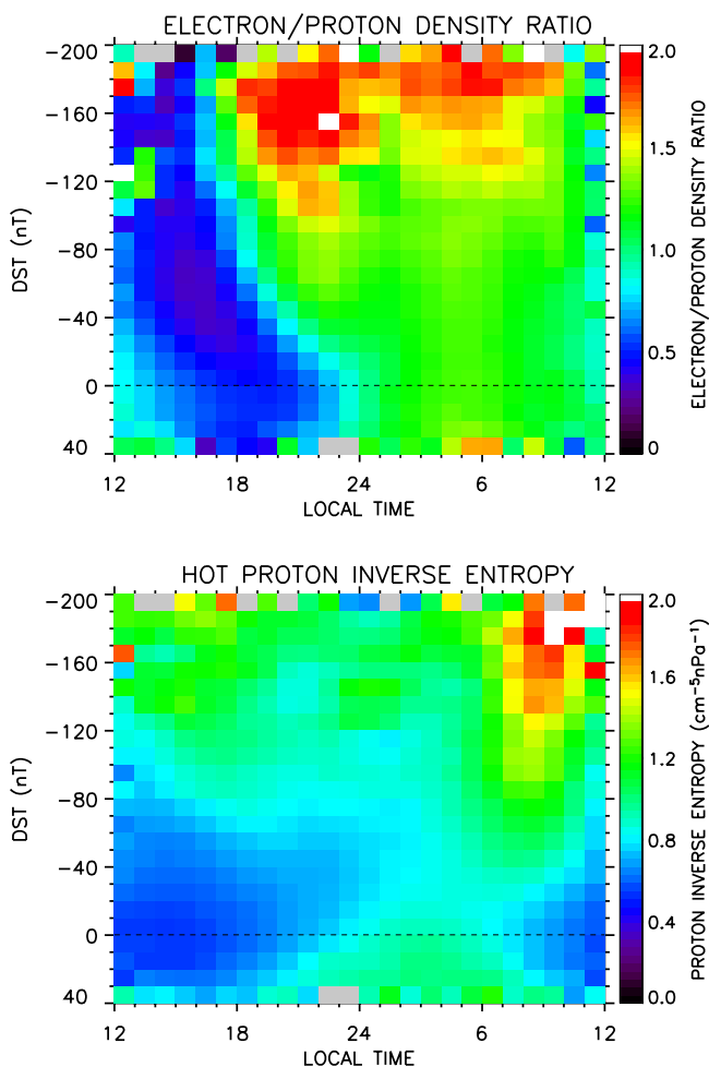
Figure 6. The averaged HE/HP density ratio and the HP inverse entropy calculated as a function of Dst index and local time for MPA data between 1990 and 2001, inclusive.
