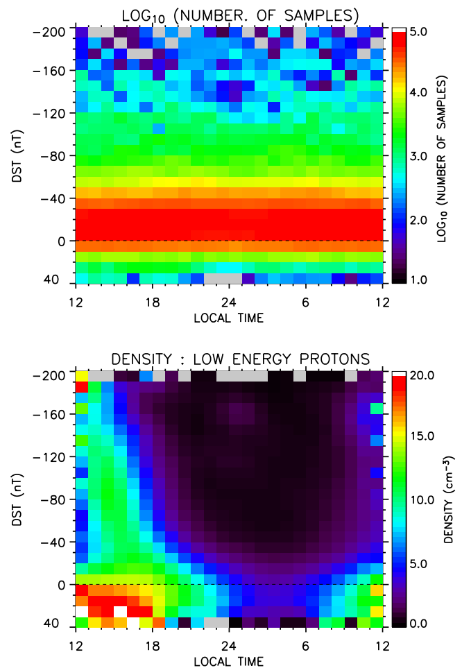
Figure 4. The sample statistics and the averaged LP density calculated as a function of Dst index and local time for MPA data between 1990 and 2001, inclusive.
