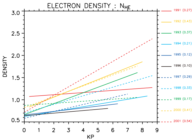
Figure 11. The averaged HE density at 0300 LT plotted as a function of the Kp index and year in the solar cycle between 1991 and 2001. Solar maximum is colored red and corresponds to 1991 and 2001. Solar minimum is colored black and corresponds to 1996.
