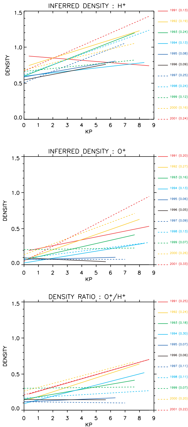
Figure 13. The inferred O^+ and H^+ density and the O^+/H^+ density ratio at 0300 LT plotted as a function of Kp and year in the solar cycle between 1990 and 2001. Solar maximum is colored red and corresponds to 1991 and 2001. Solar minimum is colored black and corresponds to 1996.
