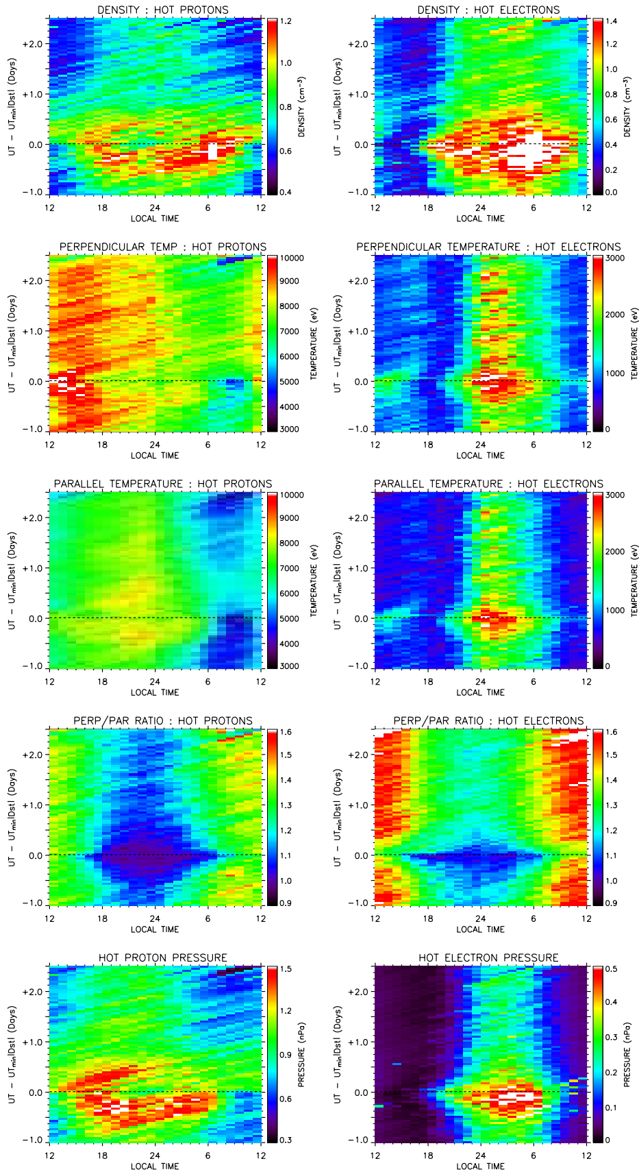
Figure 8. The averaged HP and HE density, parallel and perpendicular temperatures, the temperature anisotropies, and the pressures, calculated as a function storm epoch time, where the zero epoch occurs at minimum storm Dst .
