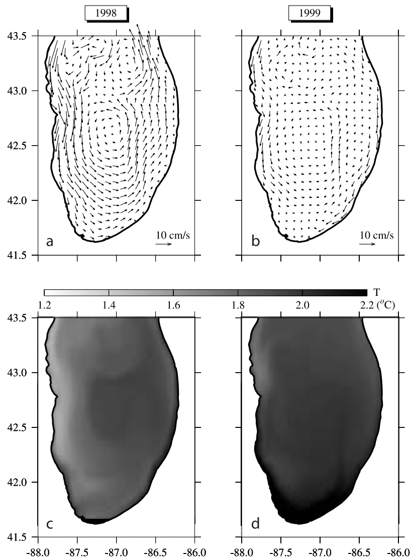
Figure 6. Distribution of monthly averaged surface water current vectors and temperature in southern Lake Michigan for March 1998 and 1999.
