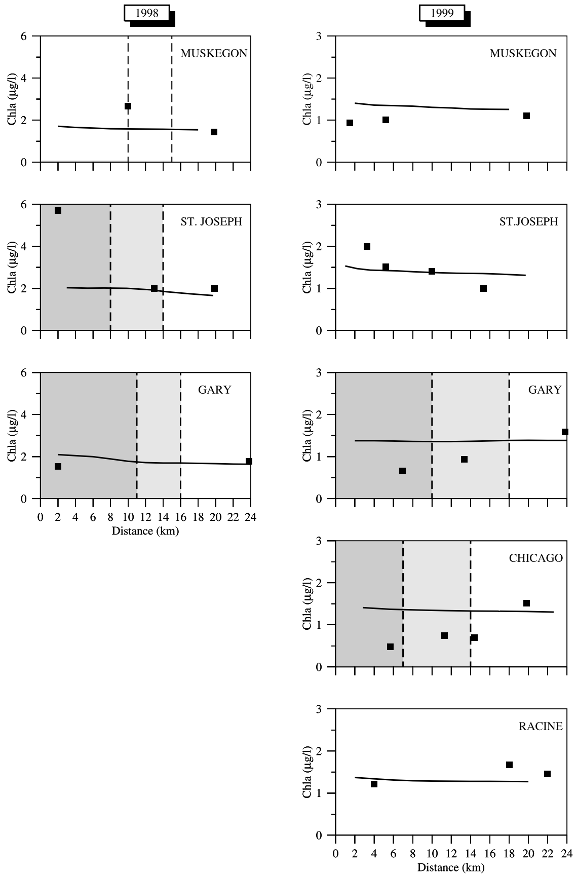
Figure 12. Comparison between model-computed and observed chlorophyll a concentrations on the Gary, St. Joseph, and Muskegon transects in March 1998 and on Gary, St. Joseph, Muskegon, Chicago, and Racine transects in March 1999. Solid squares are water samples, and curvature lines are model results.
