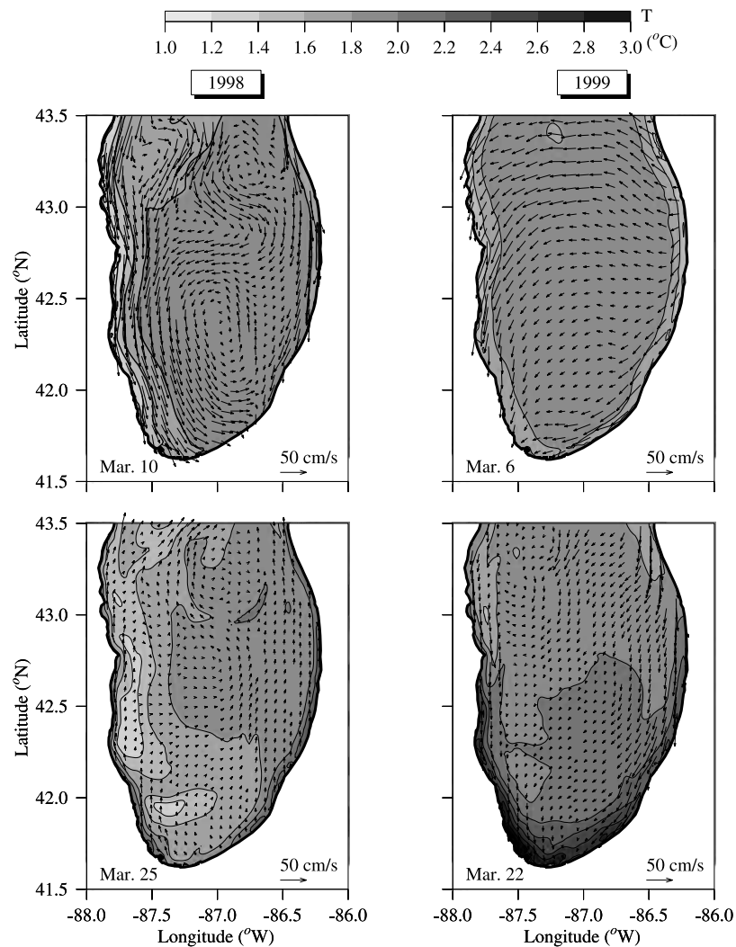
Figure 5. Distributions of surface water current vectors and temperature in southern Lake Michigan (left) on 10 and 25 March 1998 and (right) on 6 and 22 March 1999.
