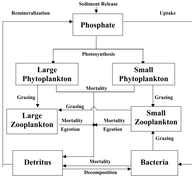
Figure 3. Schematic of the lower trophic level food web model for Lake Michigan.
