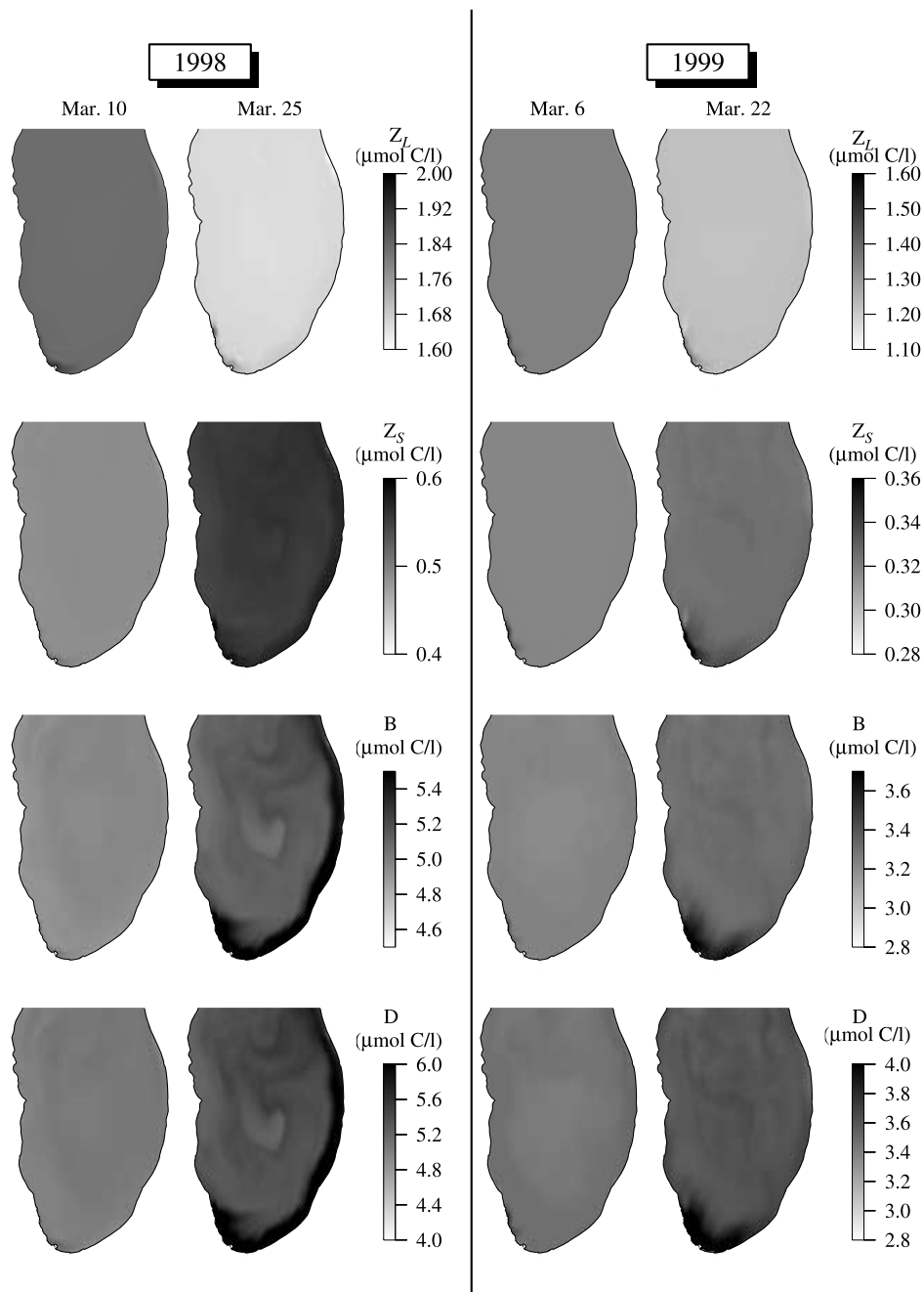
Figure 8. Distributions of large zooplankton, small zooplankton, bacteria, and detritus in southern Lake Michigan (left) on 10 and 25 March 1998 and (right) on 6 and 22 March 1999, respectively.
