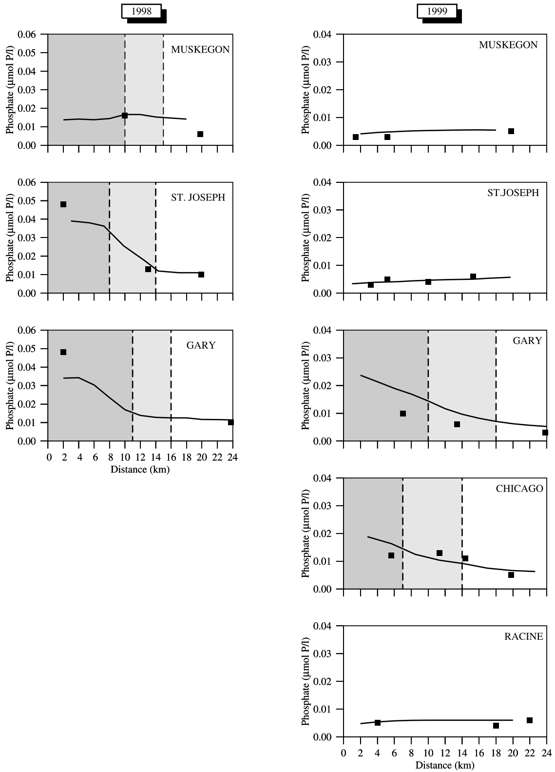
Figure 10. Comparison between model-computed and observed phosphorus concentrations on the Gary, St. Joseph, and Muskegon transects in March 1998 and on Gary, St. Joseph, Muskegon, Chicago, and Racine transects in March 1999. Solid squares are water samples, and curvature lines are model results.
