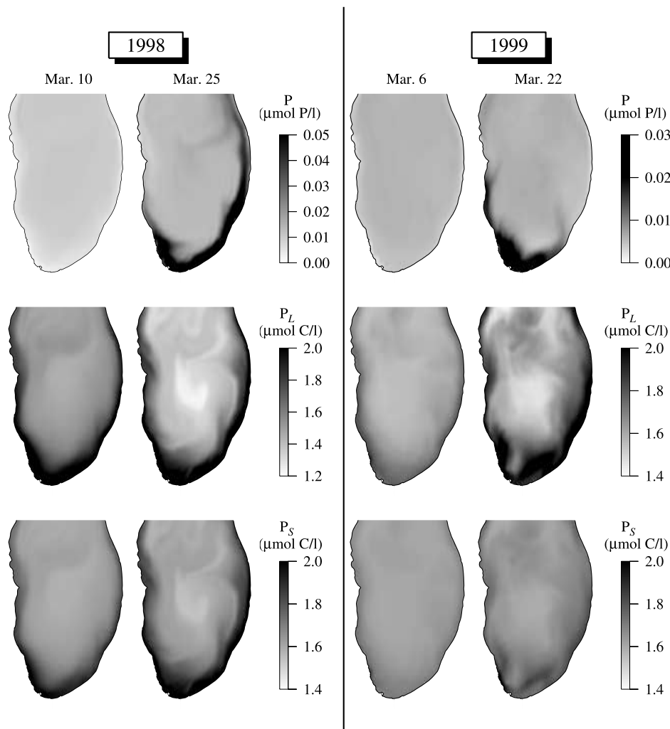
Figure 7. Distributions of phosphorus, large phytoplankton, and small phytoplankton in southern Lake Michigan (left) on 10 and 25 March 1998 and (right) on 6 and 22 March 1999, respectively.
