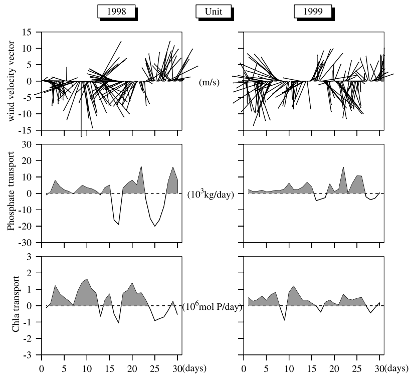
Figure 9. Time series of (top) surface wind velocity vectors and (middle) cross-plume fluxes of phosphate and chlorophyll a around the 20-m isobath during March (left) 1998 and (right) 1999. Positive: offshore flux, and negative: onshore flux.
