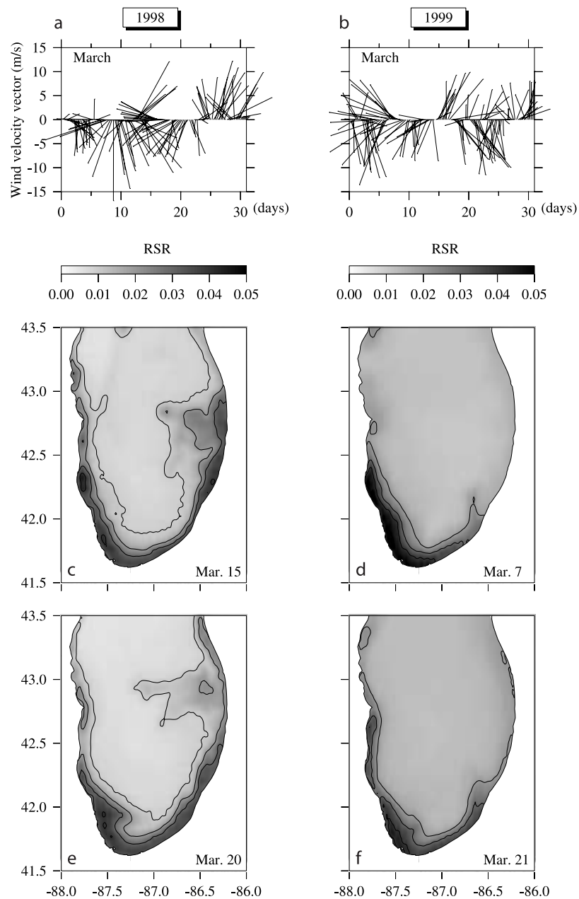
Figure 1. Time series of surface wind velocity vectors taken at center of lake basin during March of (a) 1998 and (b) 1999 and spatial distributions of remote sensing reflectance (RSR) taken on (c) 15 and (e) 20 March 1998 and (d) 7 and (f) 21 March 1999.
