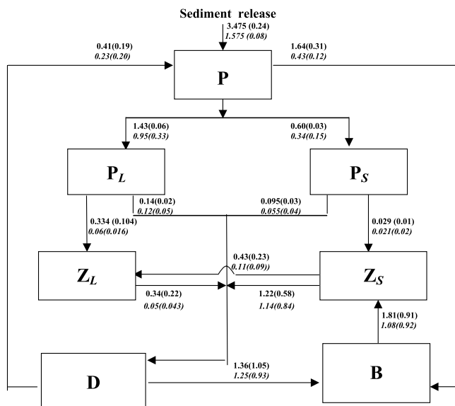
Figure 13. The model-predicted monthly averaged fluxes of biological variables among the food web inside and outside the plume for March of 1998 and 1999. The flux outside the plume was written within the brackets. The flux unit was \mu\text{mol C L}^{-1} \text{d}^{-1} .
