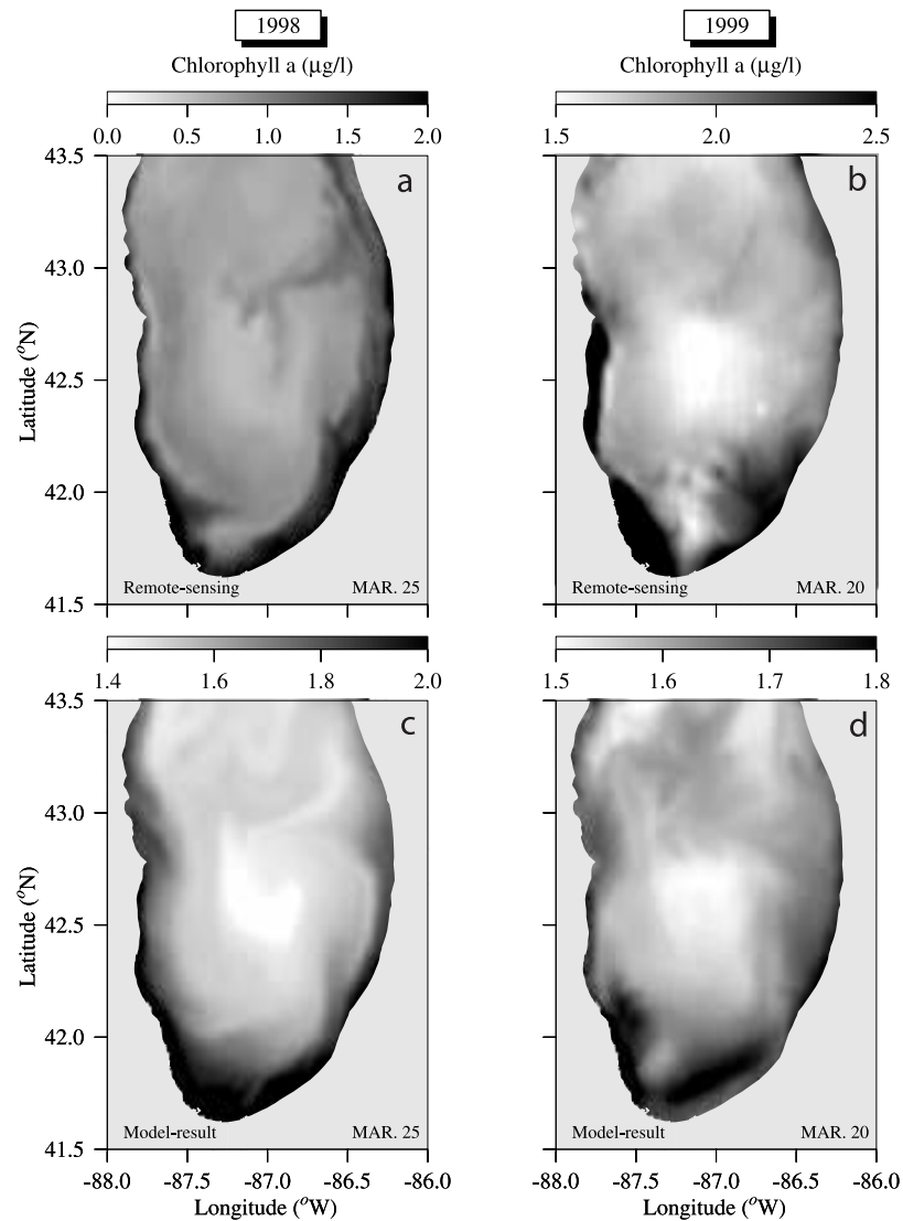
Figure 11. Comparison of the surface distributions of satellite-derived and model-computed chlorophyll a concentrations in southern Lake Michigan on 25 March 1998 and 20 March 1999.
