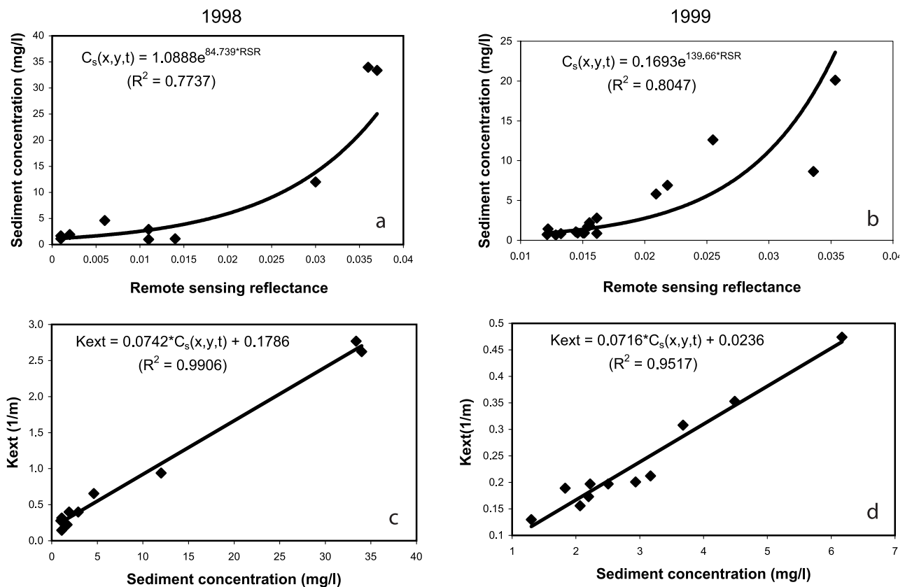
Figure 4. The regression fittings of sediment concentration with respect to remote sensing reflectance and light attenuation coefficient with respect to sediment concentration in March (left) 1998 and (right) 1999. Solid squares represent water samples collected on the transects shown in Figure 2 during the March 1998 and 1999 interdisciplinary plume cruises.
