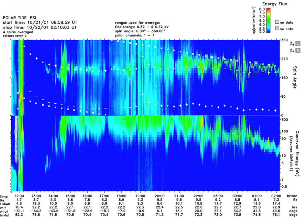
Figure 1. Polar/TIDE observations of the plasma sheet are plotted for an orbit on 21 October 2001, illustrating the following features: (a) lobal wind in both hemispheres, (b) bidirectional streaming in the plasma sheet boundary layer, (c) nearly isotropic warm plasma in the current sheet region, and (d) localized auroral acceleration and heating of the lobal wind outflows.
