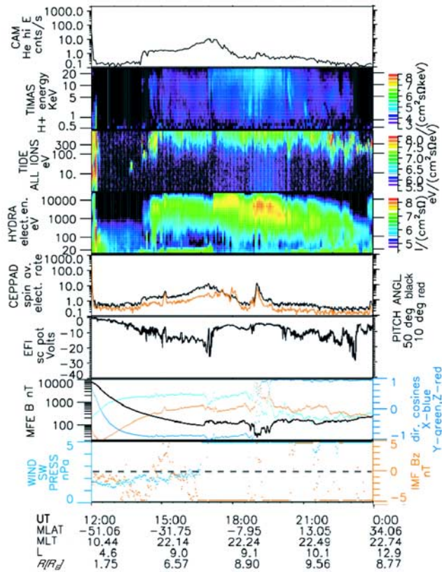
Figure 2. TIMAS and Hydra observations of hot plasmas ions and electrons illustrating the full thermal extent of the hot isotropic current sheet plasmas.
