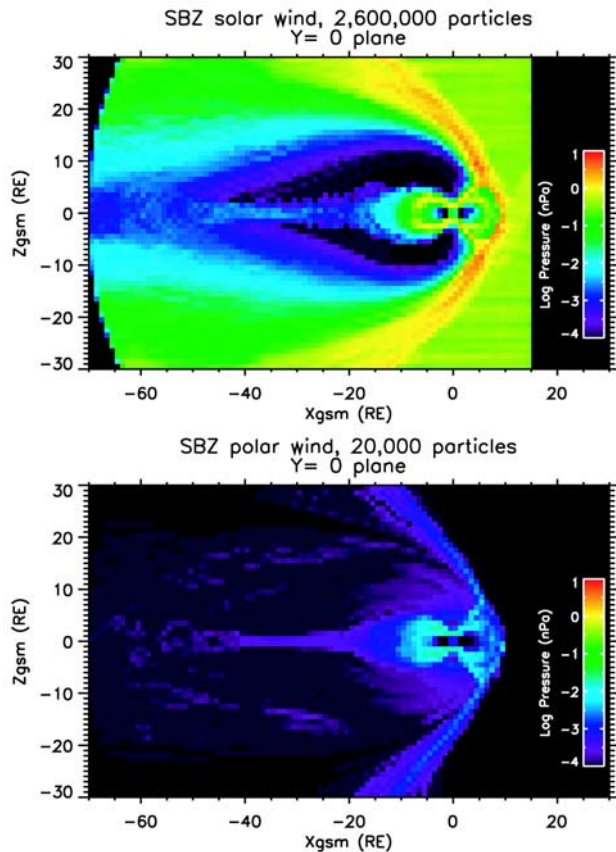
Figure 8. For the SB_Z case, the plasma pressure is color-contoured in the GSM- XZ or noon-midnight meridian plane. (top) Solar wind particle pressures and (bottom) polar wind particle pressures.
