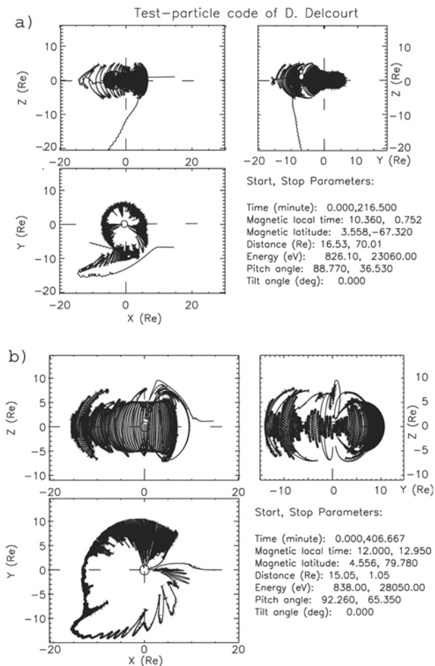
Figure 6. Example trajectories for solar wind entry in (a) the SB_Z case and (b) the NB_Z case. Insets in each panel show the YZ plane projection as seen from the Sun.
