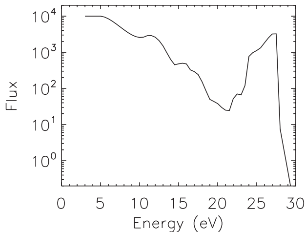
Figure 6. Scattered light photoelectron source cone distribution produced by the single flux tube model for use as a boundary condition in the bounce-averaged model. This spectrum is applied (without variation) at all local times and latitudes ( L shells) within the simulation domain.
