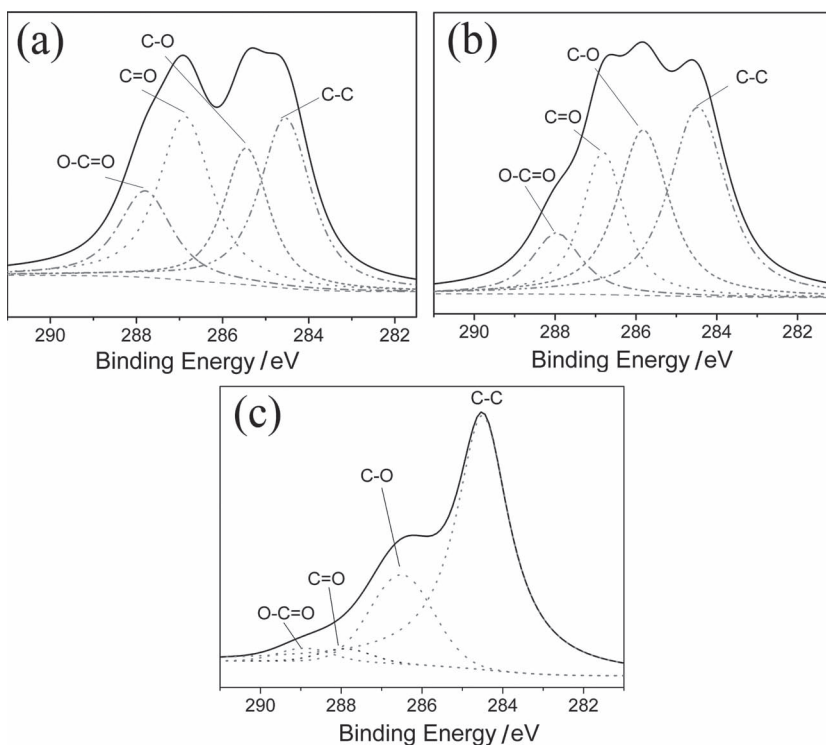
Figure 6. The C1s XPS spectra of GO (a), GNS/ \beta\text{-CD} (b), and GNS only (c) are obtained by means of a RBD upgraded PHI-5000C ESCA system with A1K \alpha radiation ( h\nu = 1486.6 \text{ eV} ).
