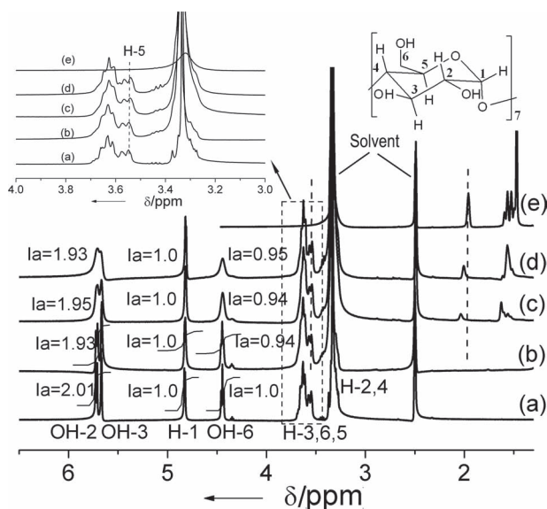
Figure 4. ^1\text{H} NMR spectra of \beta\text{-CD} (a), freeze-dried GNS/ \beta\text{-CD} (b), freeze-dried GNS/ \beta\text{-CD} /Ad-NH _2 with increasing loading ratio of Ad-NH _2 [(c) 3.88 wt%, (d) 5.71 wt%] and Ad-NH _2 (e). (DMSO- d_6 as solvent, “Ia” denotes integrated area)
