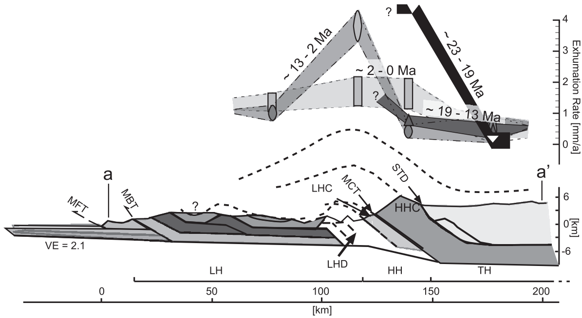
Figure 3. Temporal and spatial variations in exhumation across the NW Himalaya related to a schematic cross sections derived from previous studies [Robinson et al. , 2006; Srivastava and Mitra, 1994; Vannay et al. , 2004]. See Figure 2 for the location of the cross section. Regional distribution of exhumation rates was determined from the 1-D thermal model (see section 4.3 for further details). Dashed lines in the cross section indicate estimates of volume loss due to erosion since the early Miocene. HHC, High Himalayan Crystalline; LHC, Lesser Himalayan Crystalline; LHD, Lesser Himalayan Duplex; MCT, Main Central Thrust; STD, Southern Tibetan Detachment; MBT, Main Boundary Thrust; MFT, Main Frontal Thrust.
