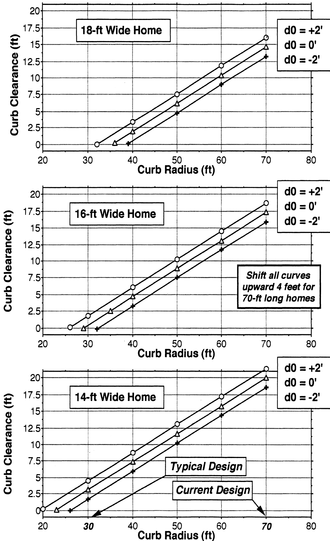
Figure 4-12. Curb Clearance vs. Curb Radius. Intersection Type 1. Three Home Widths & Three Initial Centerline Offsets (d0).
