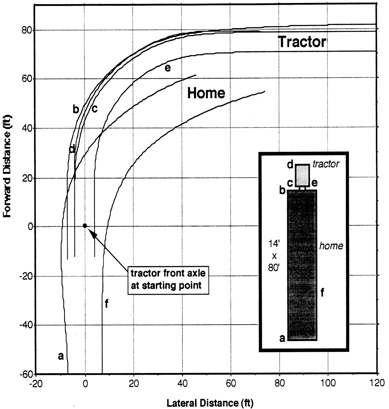
Figure 4-3. Trajectories of Various Points on a Tractor & Mobile Home Combination Vehicle as it Moves Along a 50-ft Radius Right-Hand Turn. (14-ft Wide)
