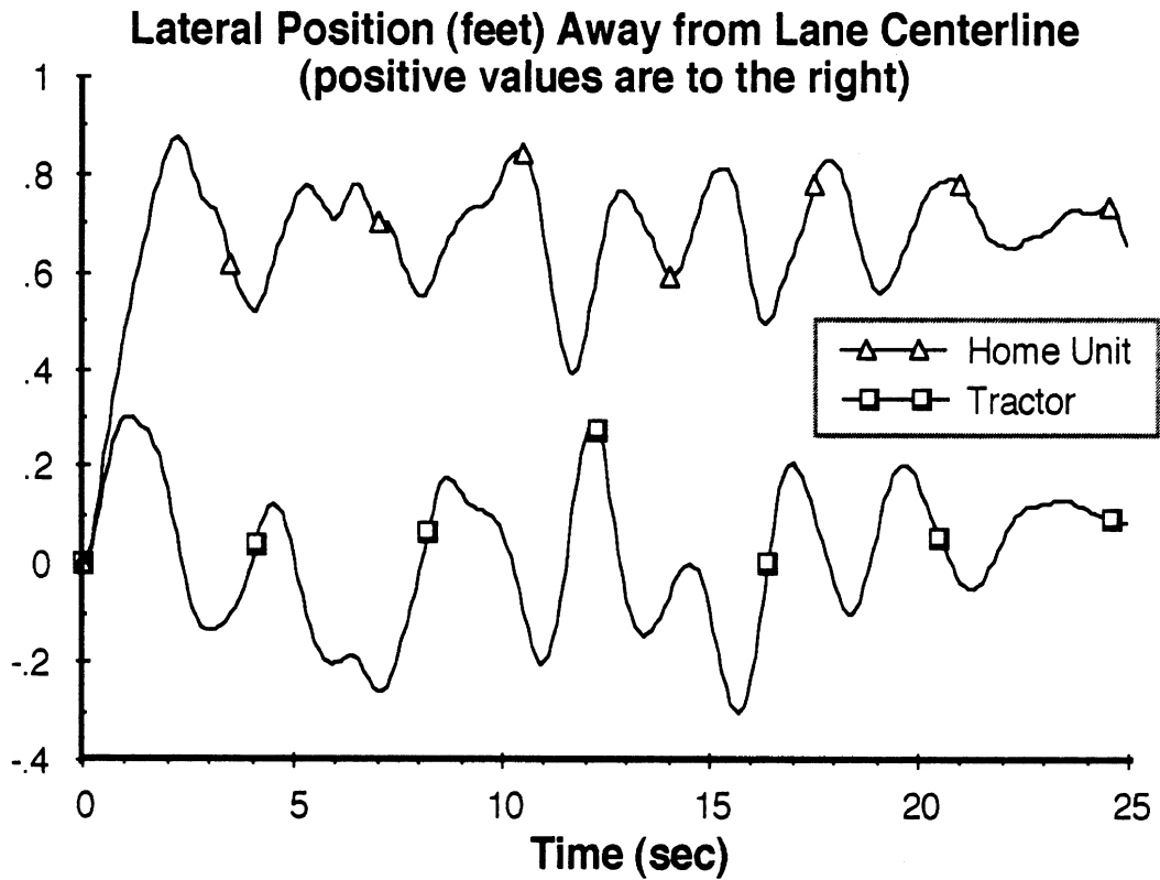
Figure 5-6. Tractor/Home Response to the 25 mph Random Crosswind. 16-ft Wide Baseline Home Unit. 45 mph Vehicle Speed.
