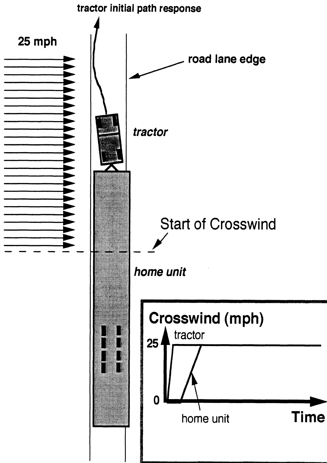
Figure 5-1. Simulated Crosswind Maneuver — Idealized Uniform Crosswind Profile.
