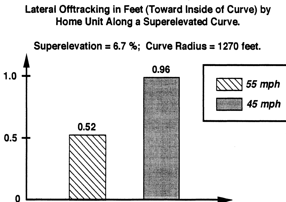
Figure 5-8. Offtracking by All Home Units Along a Superelevated Curve.
