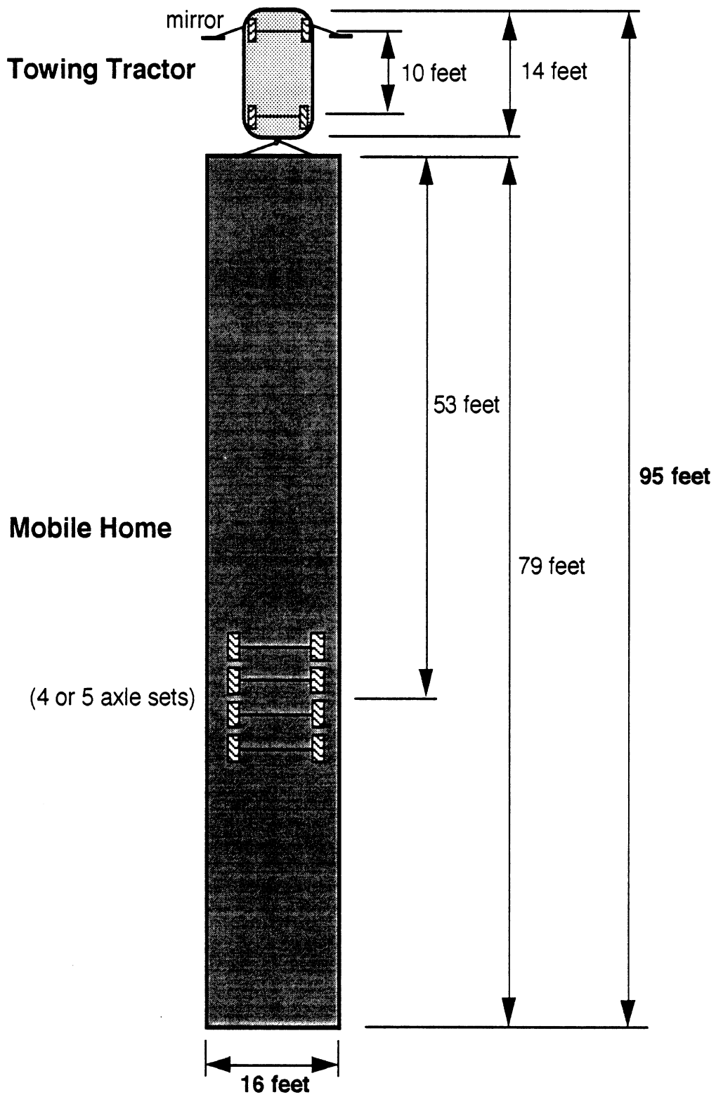
Figure 2-1. Description of an Example Mobile Home and Towing Tractor Combination as Measured by MDOT.
