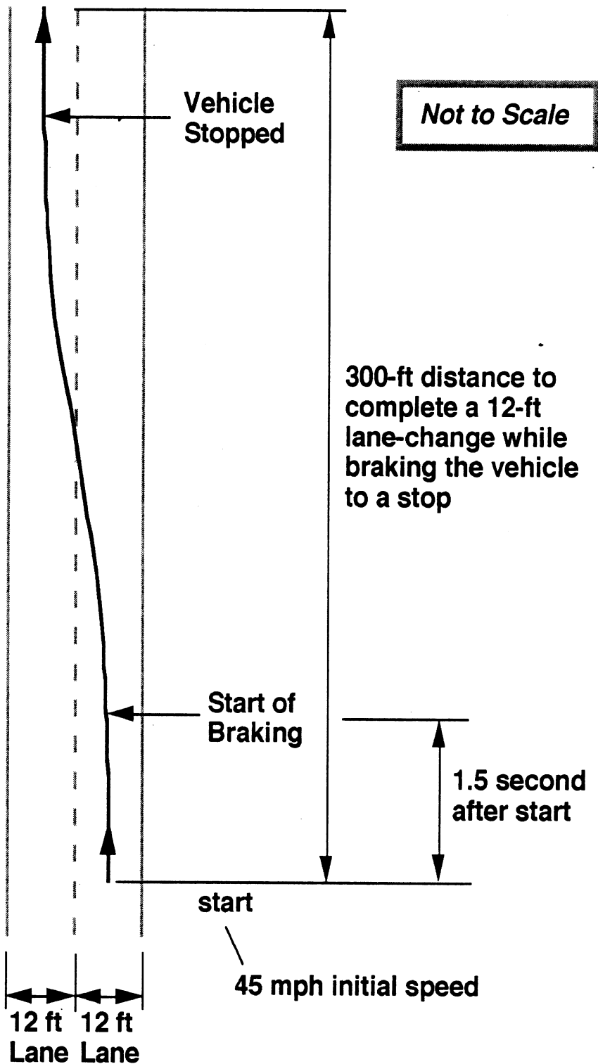
Figure 6-1. Braking Maneuver Used to Evaluate Tractor/Home Combination Braking Performance.
