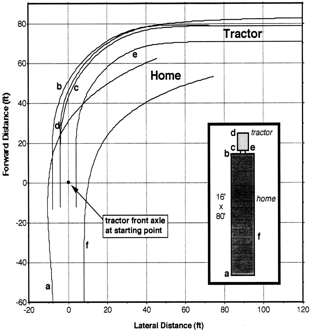
Figure 4-4. Trajectories of Various Points on a Tractor & Mobile Home Combination Vehicle as it Moves Along a 50-ft Radius Right-Hand Turn. (16-ft Wide)
