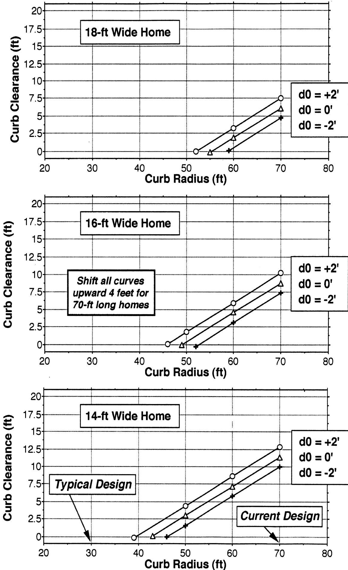
Figure 4-14. Curb Clearance vs. Curb Radius. Intersection Type 3. Three Home Widths & Three Initial Centerline Offsets (d0).
