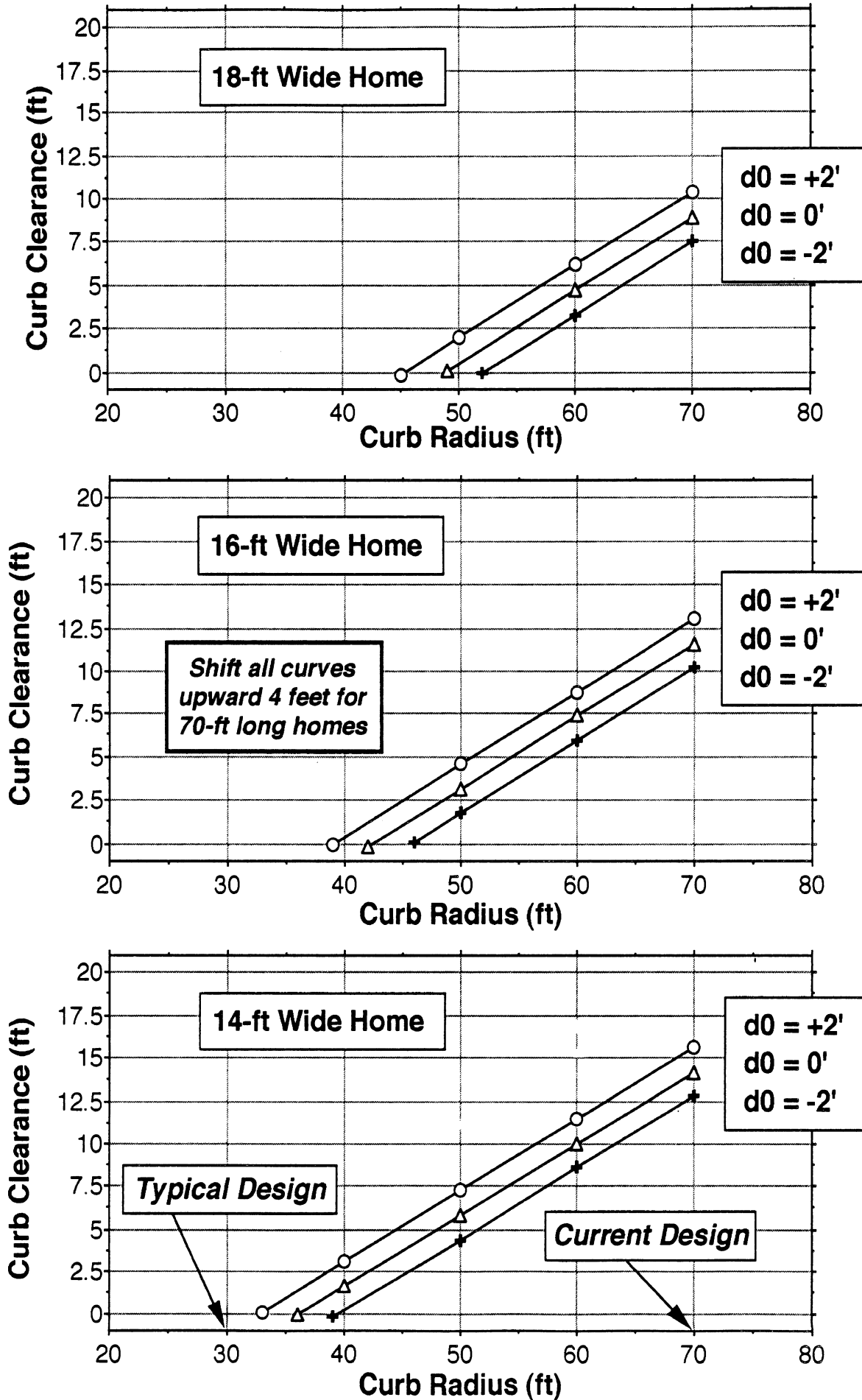
Figure 4-13. Curb Clearance vs. Curb Radius. Intersection Type 2. Three Home Widths & Three Initial Centerline Offsets (d0).
