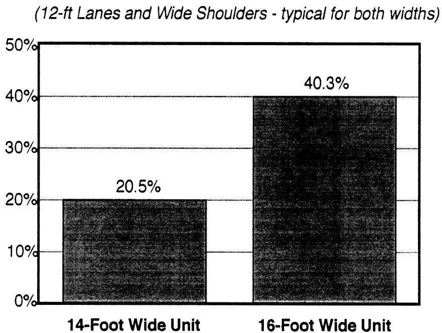
Figure 3-7. Tractor/Home Encroachment Proportion of Time Encroaching in Passing Lane (Multilane Divided Highways)
