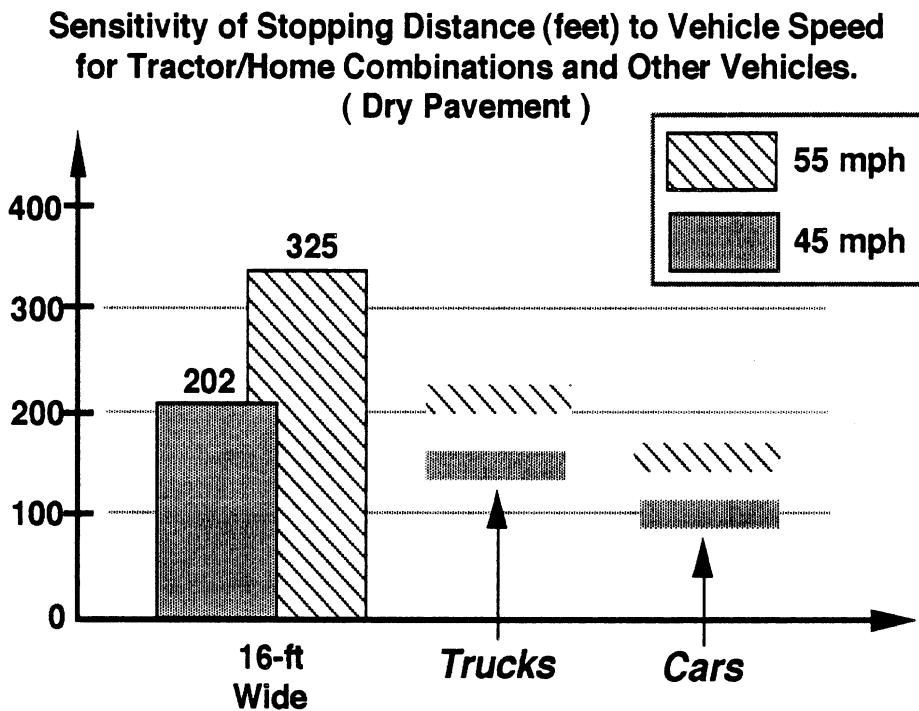
Figure 6-5. Stopping Distance Sensitivity to Vehicle Speed.
