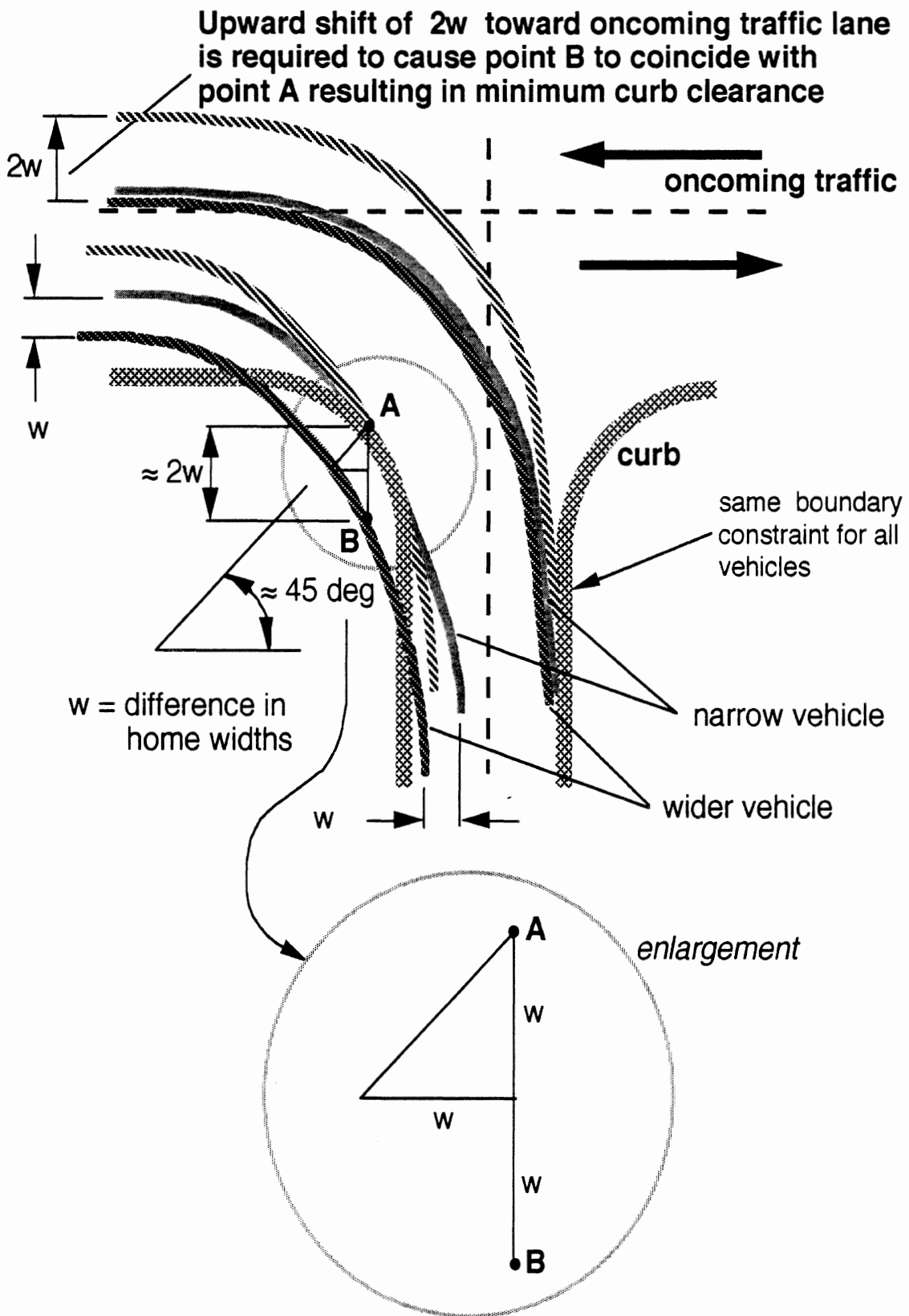
Figure 4-15. Magnified Encroachment Requirements at Intersections Due to Increased Home Width.
