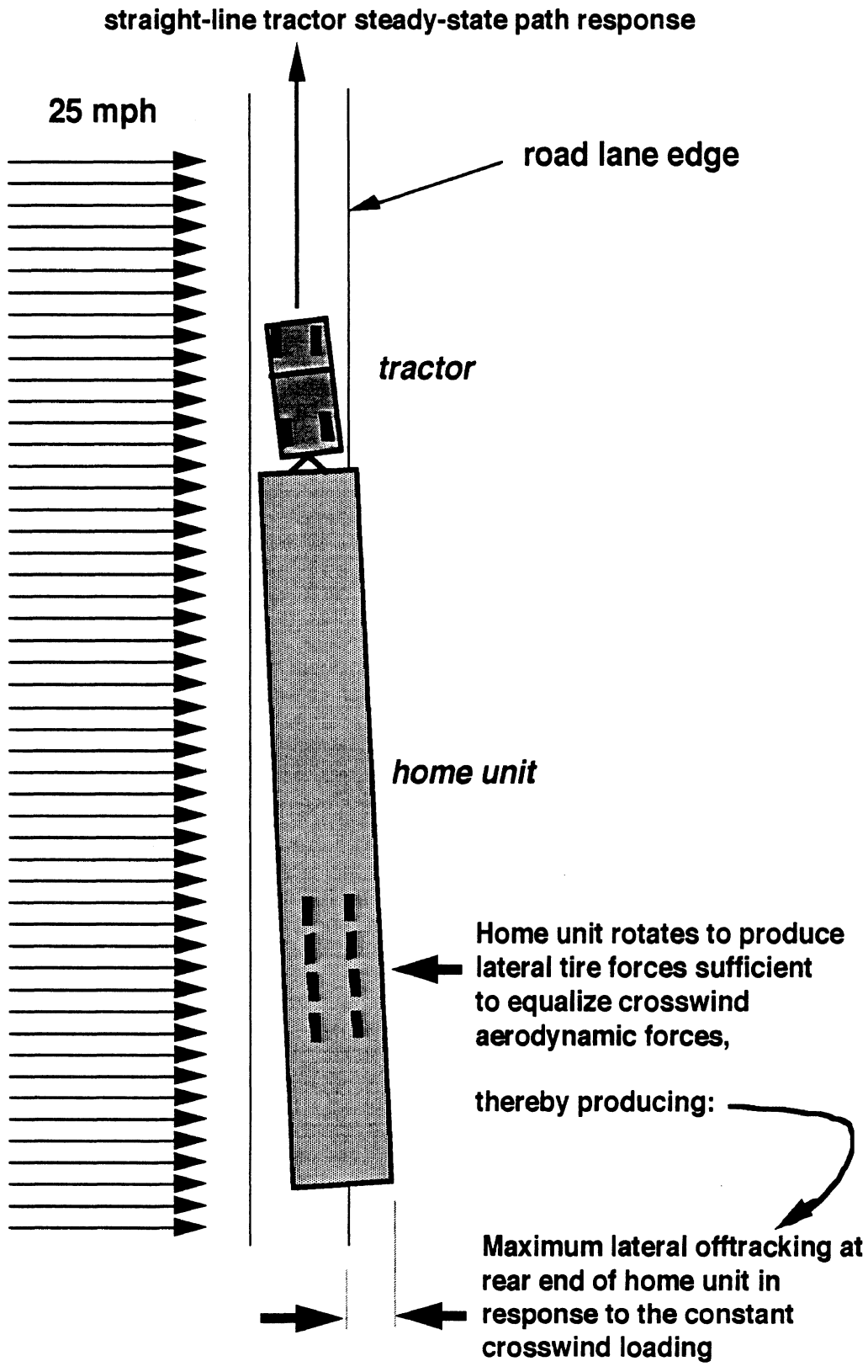
Figure 5-2. Simulated Crosswind Maneuver — Full Immersion into Crosswind and Steady-State Offtracking Response by Home Unit.
