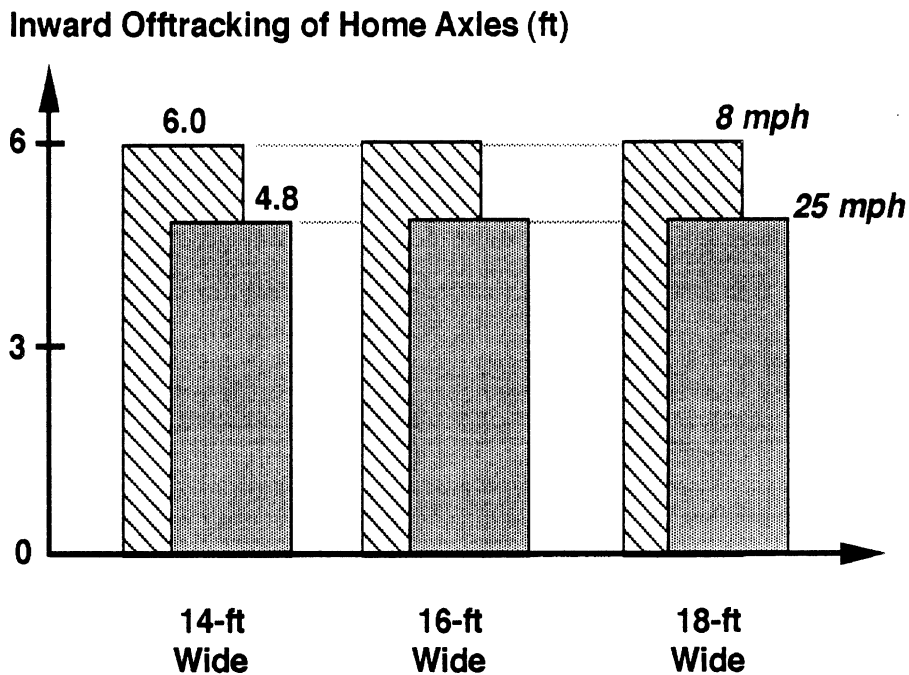
Figure 4-19. Tractor/Home Offtracking from Lane Centerline Along Freeway Exit Ramp @ 8 & 25 mph.
