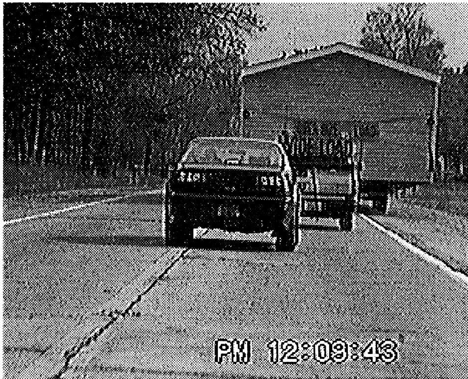
Figure A.16. Passenger vehicle behind a 16-foot wide home preparing to pass.
