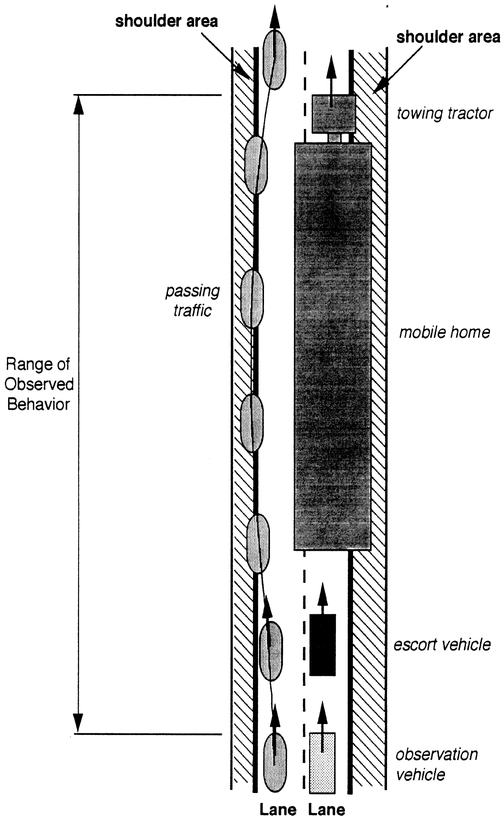
Figure 3-9. Shoulder Usage by Passing Traffic on Multilane Divided Highways.
