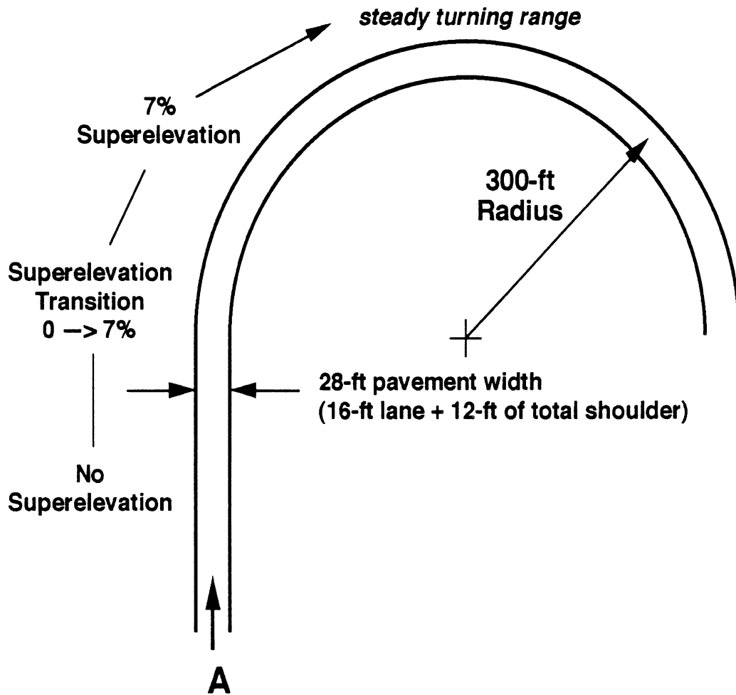
Figure 4-17. Exit Ramp Geometry Used in the Computer Analysis.
