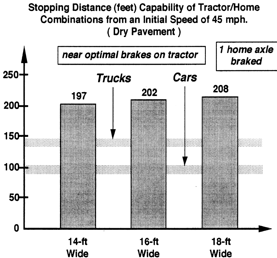
Figure 6-3. Stopping Distances for Tractor/Home Combinations and Other Highway Vehicles from 45 mph.
