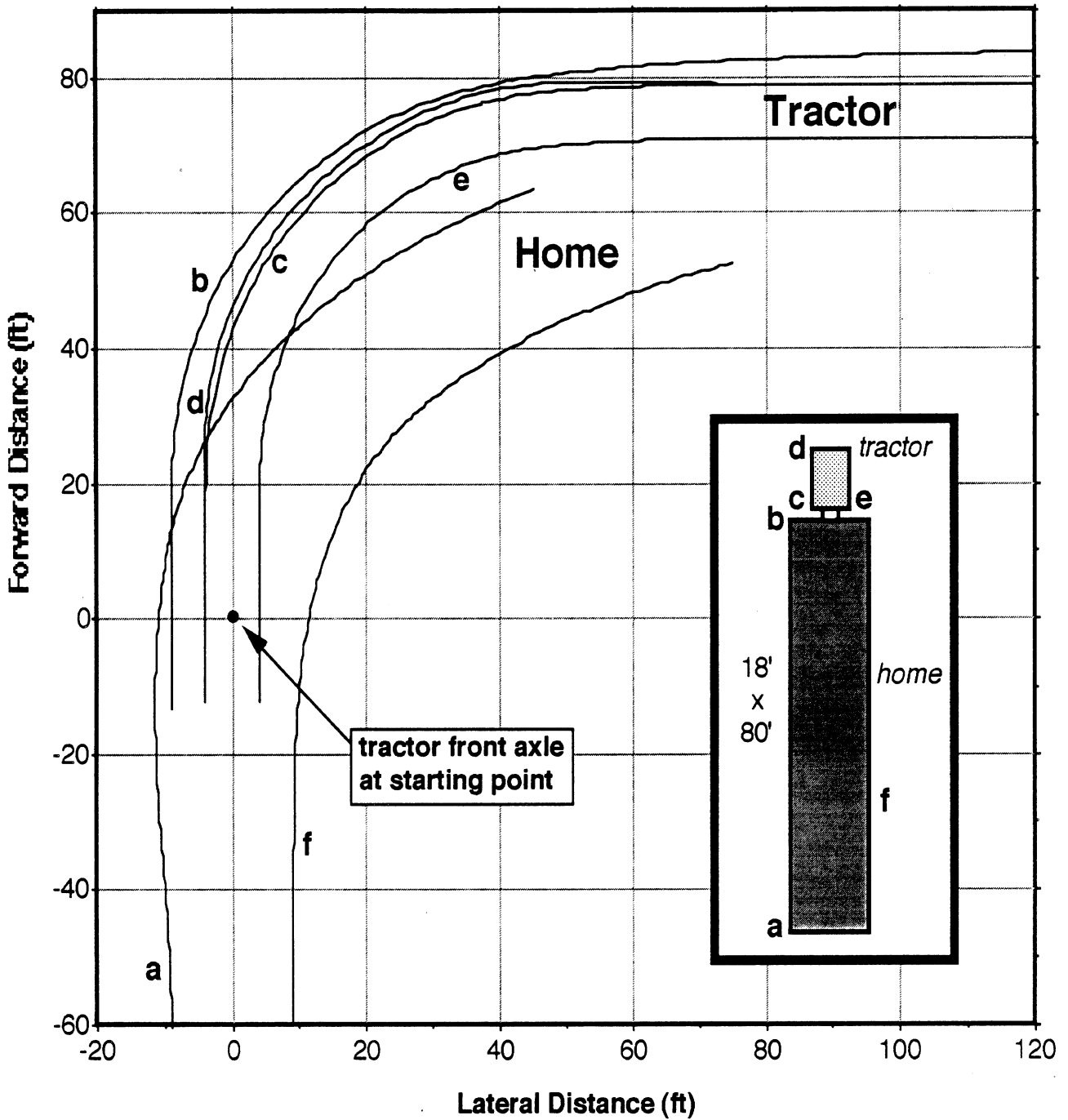
Figure 4-5. Trajectories of Various Points on a Tractor & Mobile Home Combination Vehicle as it Moves Along a 50-ft Radius Right-Hand Turn. (18-ft Wide)
