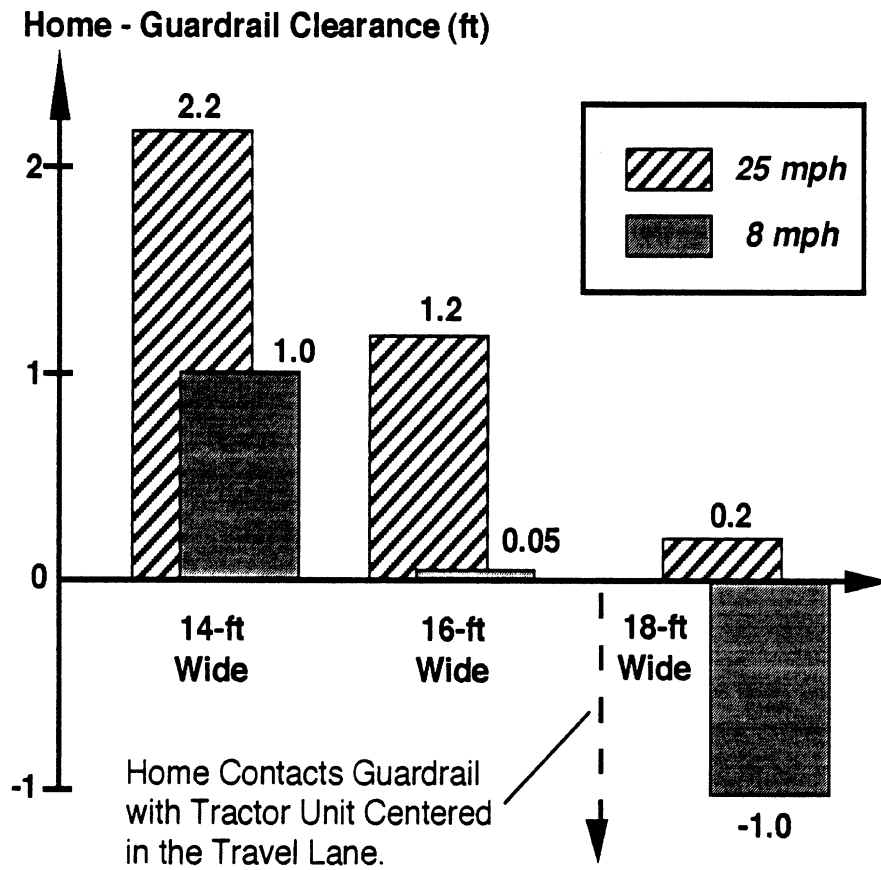
Figure 4-20. Home-to-Guard Rail Inside Clearance Along Exit Ramp for Different Home Widths. Tractor Unit Centered in Travel Lane.
