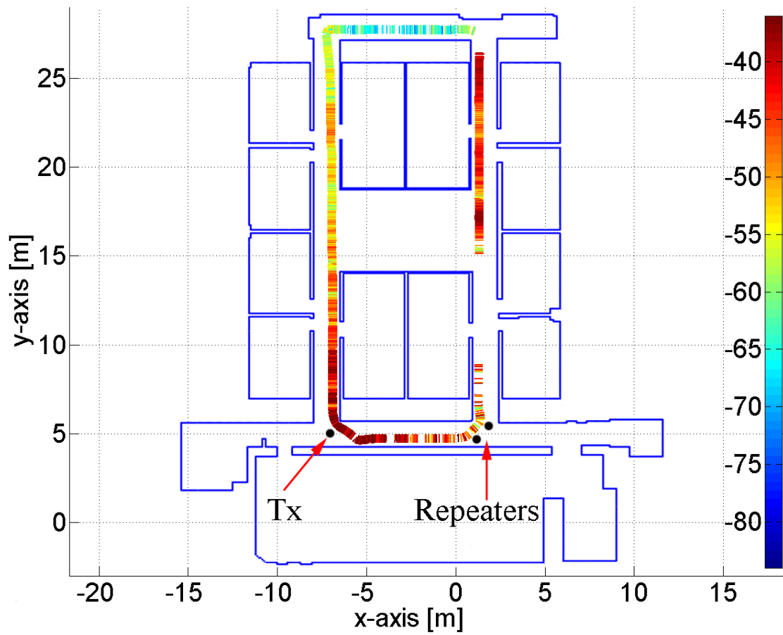
Measured fields intensity with a pair of repeaters at right-lower corner
