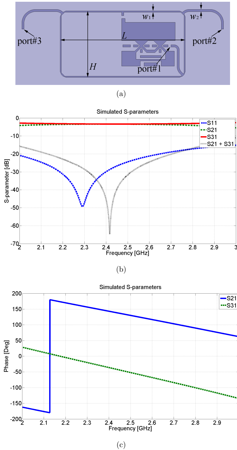
Figure 4.10: Modified hybrid ring coupler: (a) geometry of the modified hybrid ring coupler; (b) simulated S-parameters; (c) phase responses of two outputs.
