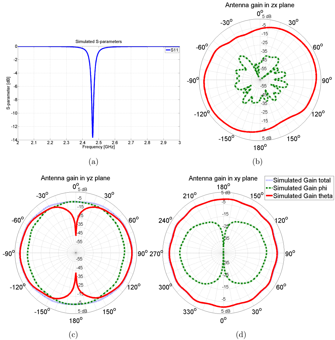
Figure 4.4: Simulated responses of the high-gain Tx antenna: (a) input reflection coefficient; (b) radiation pattern in E(zx) -plane; (c) radiation pattern in E(yz) -plane; (d) radiation pattern in H(xy) -plane.
