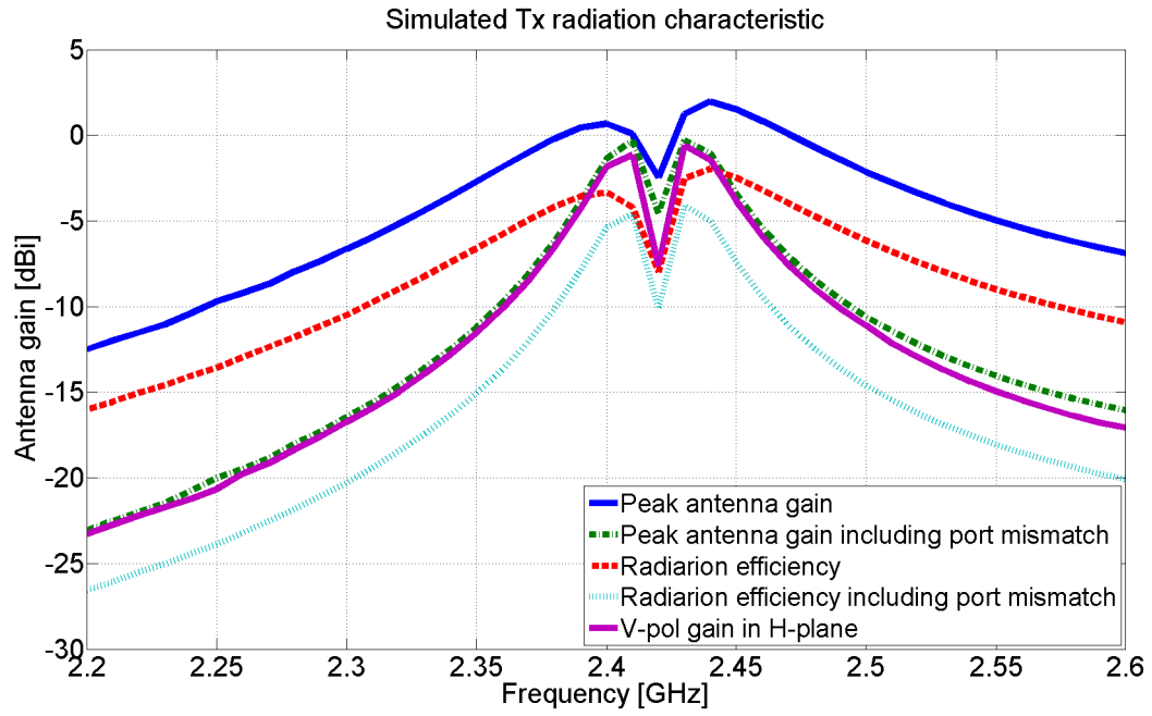
Figure 5.17: Radiation characteristic of the isolator-embedded repeater Tx antenna.
