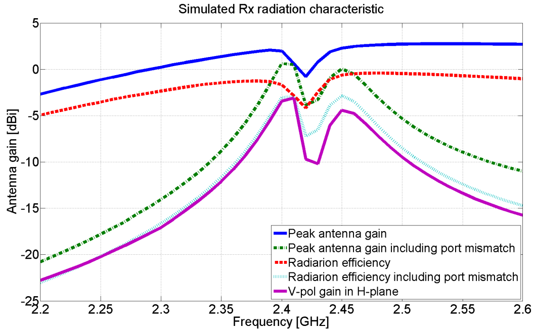
Figure 5.15: Radiation characteristic of the isolator-embedded repeater Rx antenna.
