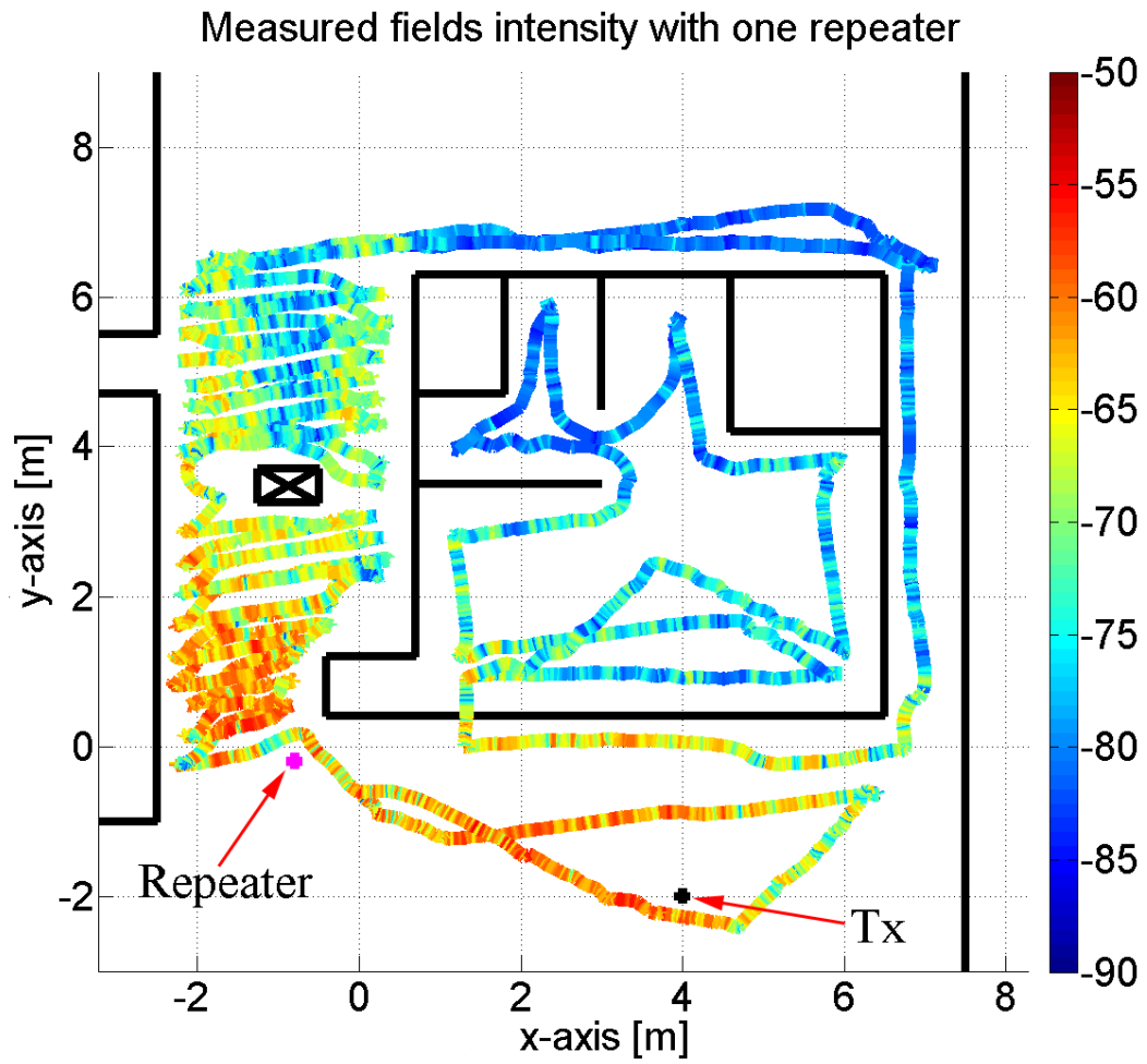
Figure A.2: Measured RSSI of a wooden building with one repeater.
