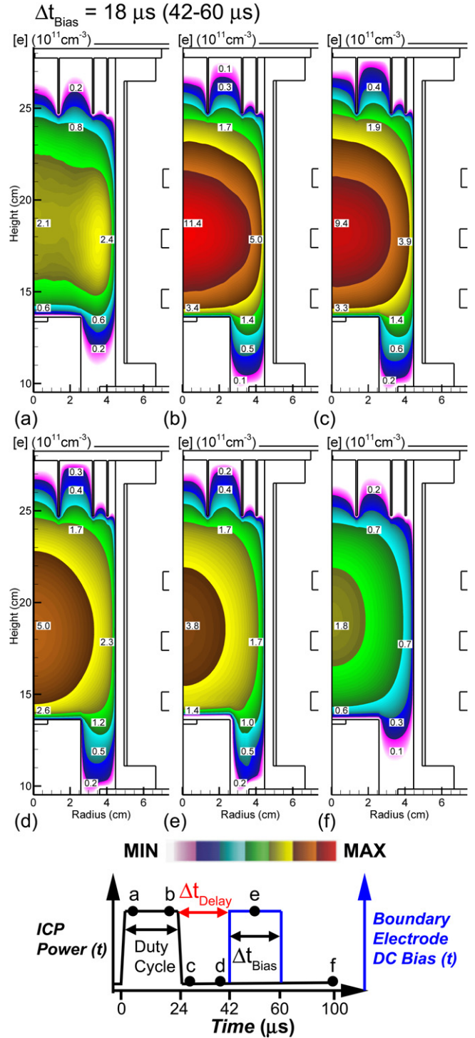
Figure 13. Electron density at different times during a single pulse for pulsed ICP and pulsed V_B = 24.4 V ( \Delta t_{Bias} = 18 \mu s (42–60 \mu s)). Plasma conditions are argon, 120 W pulsed-period-averaged power, 14 mTorr, 40 sccm, pulse repetition frequency = 10 kHz, duty cycle = 20%. (a) 2 \mu s after pulse starts. (b) 2 \mu s before pulse ends. (c) 2 \mu s after pulse ends. (d) 2 \mu s before start of applied bias. (e) Middle of applied bias time period. (f) End of pulse. The times of each frame are noted in the waveform. n_e peaks in the skin depth early during the pulse where the ionization sources are large, and become diffusion dominated later in the pulse and afterglow. Application of V_B does not significantly affect n_e .
