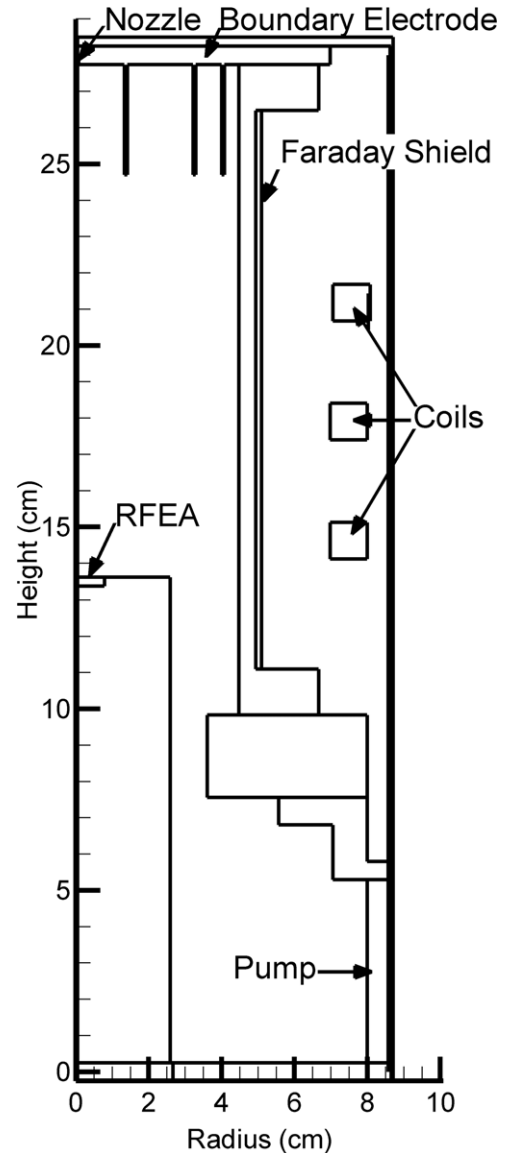
Figure 1. Schematic of the BE-ICP reactor when measuring IEDs using the RFEA. When comparing with experimental results obtained with the Langmuir probe, the RFEA was removed.
