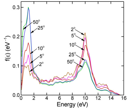
Figure 10. Simulated IEDs as a function of ion collection angle (in degrees from normal) from the surface of the RFEA, 2^\circ – 50^\circ (FWHM 4^\circ – 10^\circ about the normal). Plasma conditions are argon, 120 W pulsed-period-averaged power, 40 sccm, pulse repetition frequency = 10 kHz, duty cycle = 20% and V_B = 0 V. The efficiency of collecting low-energy ions decreases with decreasing collection angle.
