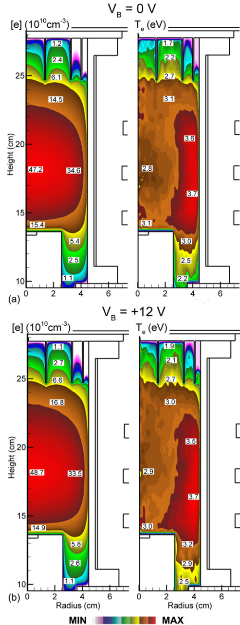
Figure 4. Electron density and temperature for two BE bias voltages. (a) V_B = 0 V. (b) V_B = +12 V. Plasma conditions are argon, 300 W (cw), 14 mTorr and 40 sccm.
