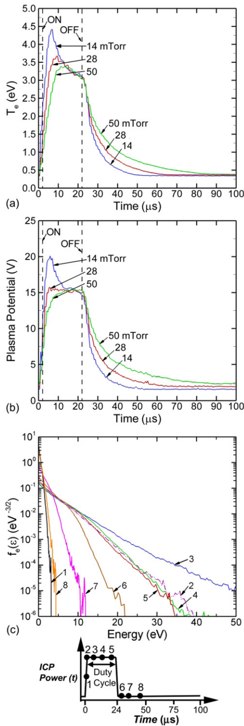
Figure 7. Plasma parameters as a function of time for a single pulse of the ICP power without the RFEA in place. The plasma conditions are argon, 120 W pulsed-period-averaged power, 40 sccm, pulse repetition frequency = 10 kHz and 20% duty cycle. (a) Reactor averaged electron temperature at different pressures. (b) Maximum plasma potential at different pressures. (c) Electron energy distribution taken at designated times (points 1–8 on the ICP power envelope) at a pressure of 14 mTorr.
