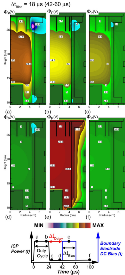
Figure 11. Plasma potential at different times during a single pulse for pulsed ICP and pulsed V_B = 24.4 V ( \Delta t_{\text{Bias}} = 18 \mu\text{s} ( 42 – 60 \mu\text{s} )). Plasma conditions are argon, 120 W pulsed-period-averaged power, 14 mTorr, 40 sccm, pulse repetition frequency = 10 kHz, duty cycle = 20%. (a) 2 \mu\text{s} after pulse starts. (b) 2 \mu\text{s} before pulse ends. (c) 2 \mu\text{s} after pulse ends. (d) 2 \mu\text{s} before start of applied bias. (e) Middle of applied bias time period. (f) End of pulse. The times of each frame are noted in the waveform. The plasma potential is nearly uniformly elevated by application of V_B .
