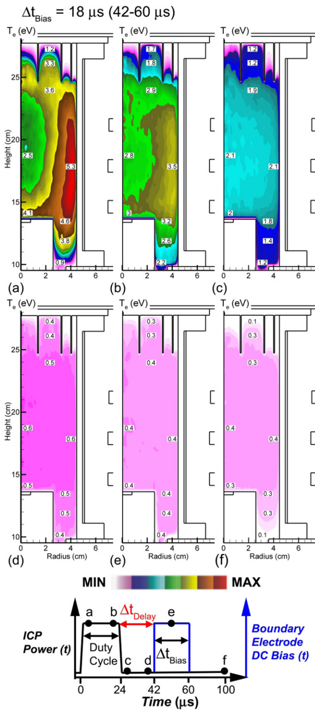
Figure 12. Electron temperature at different times during a single pulse for pulsed ICP and pulsed V_B = 24.4 V ( \Delta t_{Bias} = 18 \mu s (42–60 \mu s)). Plasma conditions are argon, 120 W pulsed-period-averaged power, 14 mTorr, 40 sccm, pulse repetition frequency = 10 kHz, duty cycle = 20%. (a) 2 \mu s after pulse starts. (b) 2 \mu s before pulse ends. (c) 2 \mu s after pulse ends. (d) 2 \mu s before start of applied bias. (e) Middle of applied bias time period. (f) End of pulse. The times of each frame are noted in the waveform. T_e peaks in the skin depth during the pulse and becomes more uniform in the afterglow. Application of V_B does not significantly affect T_e .
