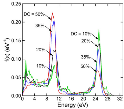
Figure 17. IEDs for a pulsed plasma for different duty cycles with V_B = 24.4 V applied on the BE in the afterglow of the ICP. Plasma conditions are argon, 120 W pulsed-period-averaged power, 14 mTorr, 40 sccm, pulse repetition frequency = 10 kHz. The bias was applied during a time period \Delta t_{\text{Bias}} = 28 \mu\text{s} (70–98 \mu\text{s} ) for all cases. With increasing duty cycle, a larger proportion of ions is collected with energies corresponding to the peak in plasma potential during the ICP pulse.
