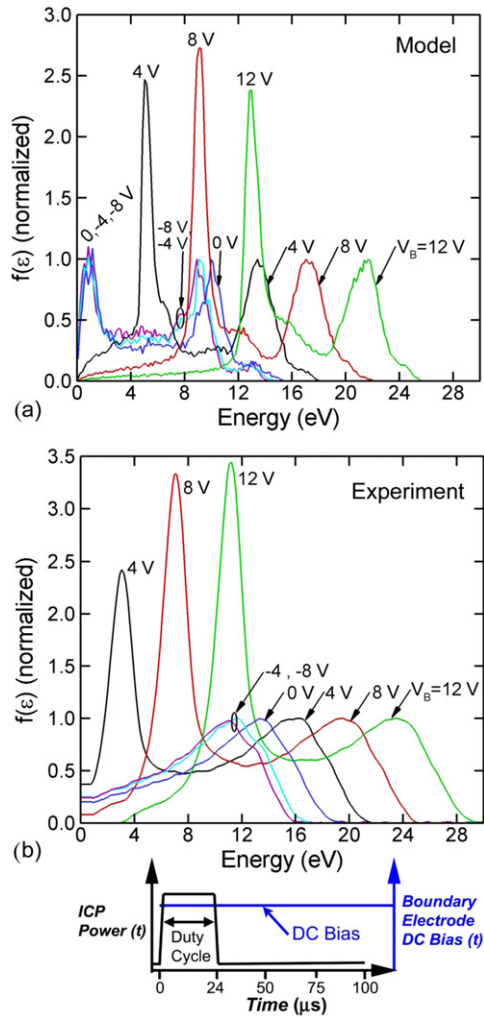
Figure 9. Normalized IEDs in pulsed plasma for different dc V_B applied on the BE. Each distribution is normalized with respect to its peak value during the pulse ON period. The plasma conditions are argon, 120 W pulsed-period-averaged power, 40 sccm, pulse repetition frequency = 10 kHz and 20% duty cycle. (a) Simulated and (b) experiments.
