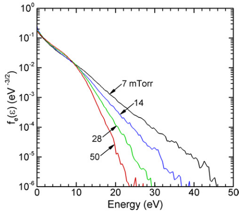
Figure 3. Simulated electron energy distributions, f_e(\epsilon) , at different pressures, near the skin depth of the electromagnetic wave without the RFEA ( r = 3.5 cm, z = 18 cm). Plasma conditions are 300 W (cw) and 40 sccm flow rate. The f_e(\epsilon) resemble two-temperature distributions.
