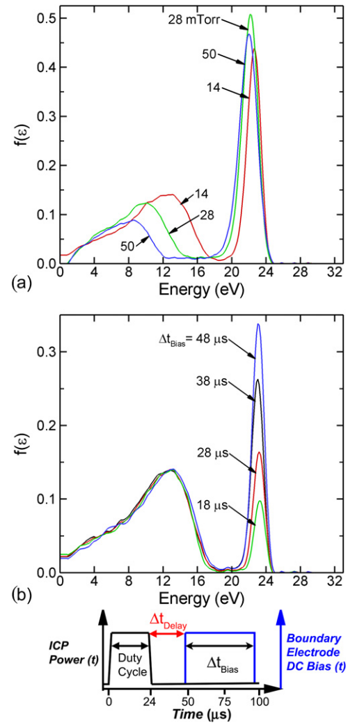
Figure 15. Experimental IEDs for pulsed plasma conditions with V_B = 24.4 V applied on the BE in the afterglow of the ICP at different pressures and bias pulse lengths. Plasma conditions are argon, 120 W pulsed-period-averaged power, 40 sccm, pulse repetition frequency = 10 kHz, duty cycle = 20%. (a) IEDs for a fixed delay time, \Delta t_{\text{Delay}} = 23 \mu\text{s} , and \Delta t_{\text{Bias}} = 50 \mu\text{s} (45–95 \mu\text{s} ) at different pressures. (b) IEDs at a fixed pressure of 14 mTorr and fixed dc bias end time of 98 \mu\text{s} . \Delta t_{\text{Delay}} is varied from 28 to 58 \mu\text{s} which produces \Delta t_{\text{Bias}} = 18 –48 \mu\text{s} .
