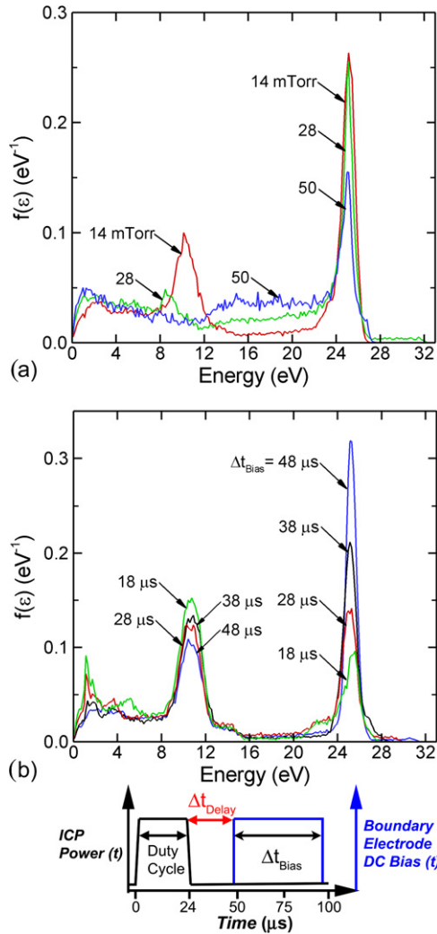
Figure 14. Simulated IEDs for pulsed plasma conditions with V_B = 24.4 V applied on the BE in the afterglow of the ICP at different pressures and bias pulse lengths. Plasma conditions are argon, 120 W pulsed-period-averaged power, 40 sccm, pulse repetition frequency = 10 kHz, duty cycle = 20%. (a) IEDs for a fixed delay time, \Delta t_{\text{Delay}} = 23 \mu\text{s} , and \Delta t_{\text{Bias}} = 50 \mu\text{s} (45–95 \mu\text{s} ) at different pressures. (b) IEDs at a fixed pressure of 14 mTorr and fixed dc bias end time of 98 \mu\text{s} . \Delta t_{\text{Delay}} is varied from 28 to 58 \mu\text{s} which produces \Delta t_{\text{Bias}} = 18 –48 \mu\text{s} . The high-energy peak of the IEDs scales with \Delta t_{\text{Bias}} .
