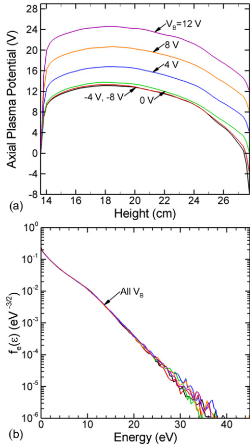
Figure 5. Parameters for a cw Ar plasma at 300 W, 14 mTorr and 40 sccm for different dc biases with the RFEA in place. (a) Plasma potential as a function of height on axis. (b) Electron energy distributions. f_e(\epsilon) are shown for V_B from -8 to 12 V, but are nearly indistinguishable.
