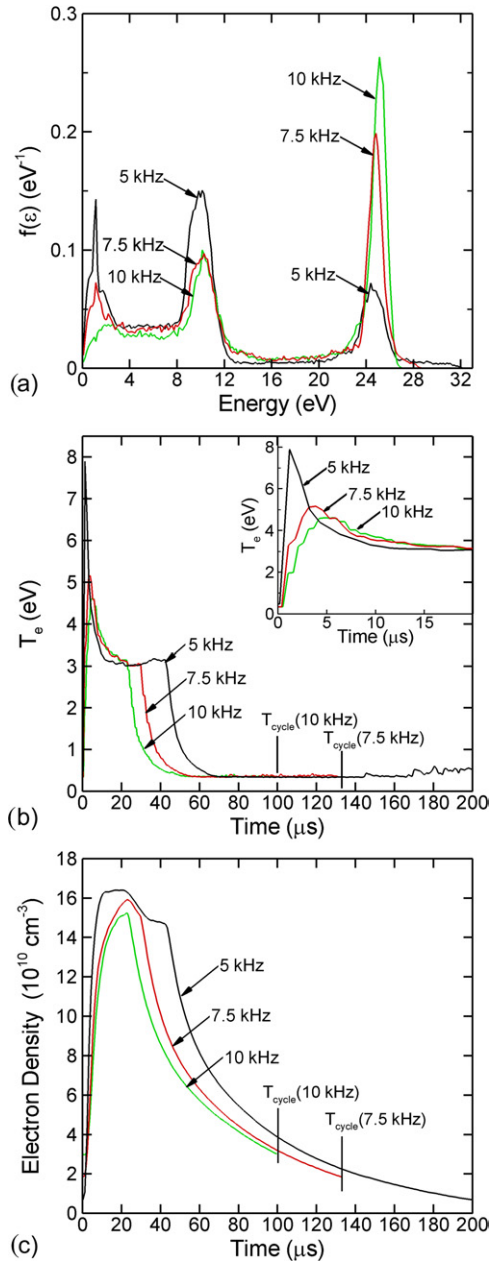
Figure 16. Properties for a pulsed plasma for different pulse repetition frequencies with V_B = 24.4 V applied on the BE in the afterglow of the ICP. Plasma conditions are argon, 120 W pulsed-period-averaged power, 14 mTorr, 40 sccm, duty cycle = 20%. (a) IEDs, (b) electron temperature (the inset shows early times during the pulse) and (c) electron density. V_B was applied for \Delta t_{\text{Bias}} = 50 \mu\text{s} for all cases, over times of 45–95 \mu\text{s} at 10 kHz, 75–125 \mu\text{s} at 7.5 kHz, and 145–195 \mu\text{s} for 5 kHz.
