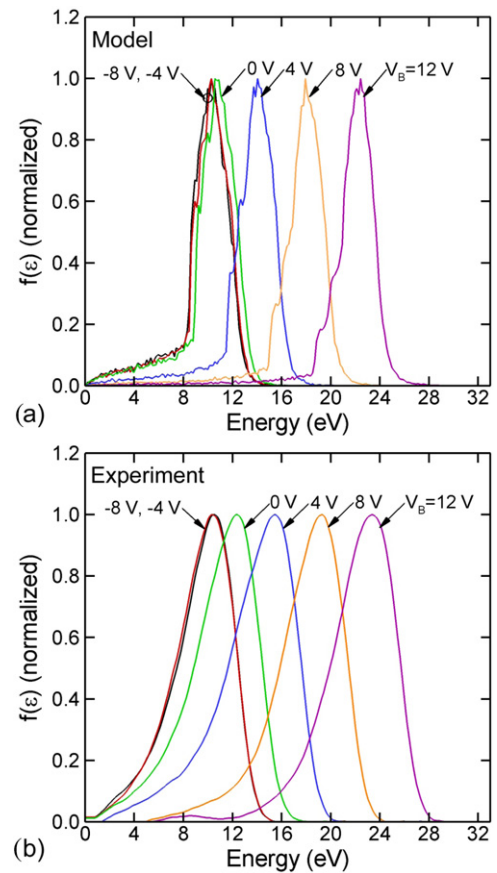
Figure 6. IEDs for different BE dc biases. (a) Simulated and (b) experimental. The IEDs have been normalized so their peak values are approximately equal. The plasma conditions are Ar, 300 W (cw), 14 mTorr and 40 sccm. The peak of the IED can be shifted to higher values by approximately the value of V_B .
