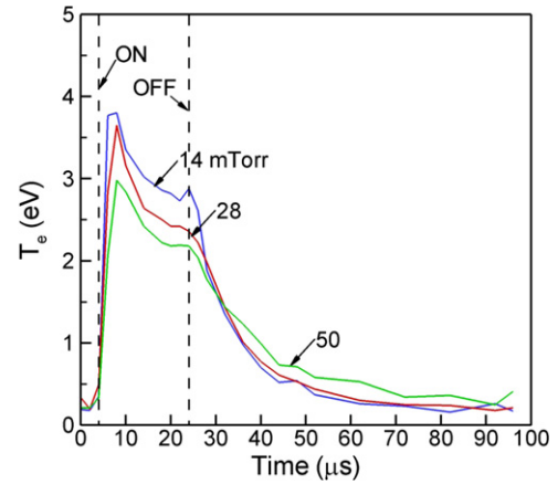
Figure 8. Experimental electron temperature as a function of time for a single pulse at different pressures without the RFEA in place. The plasma conditions are argon, 120 W pulsed-period-averaged power, 40 sccm, pulse repetition frequency = 10 kHz and 20% duty cycle.
