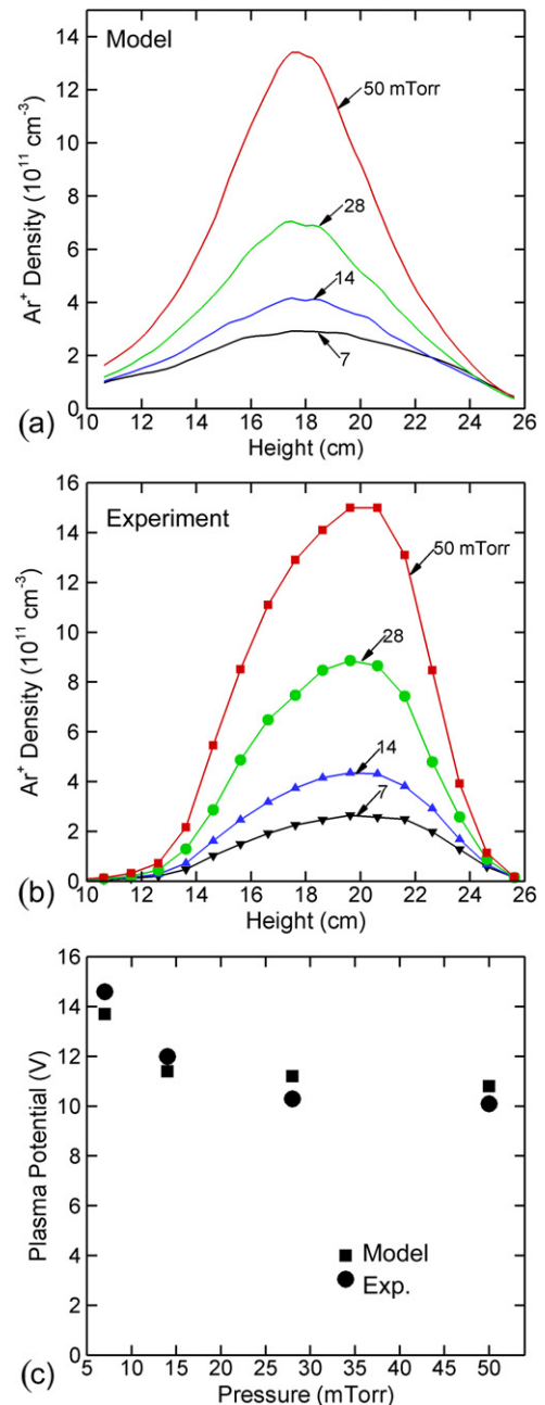
Figure 2. Plasma parameters at different pressures for a cw Ar plasma at 300 W and 40 sccm without RFEA. (a) Simulated ion density as a function of height near the axis of symmetry. (b) Experimental ion density as a function of height. (c) Experimental and simulated plasma potential taken on axis at a height of 13.6 cm (height of the RFEA).
