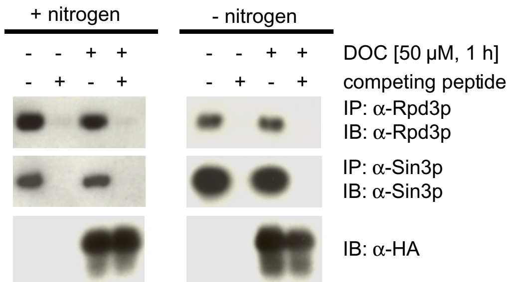
Fig. 2S. Expression levels of Rpd3p and Sin3p are unchanged in cells expressing Hac1 ip . Immunoprecipitation of Rpd3p and Sin3p from exponentially growing cells (+ nitrogen, left) and cells shifted to nitrogen-free medium for 1 h (- nitrogen, right). Expression of HA-Hac1 ip was induced with 50 \mu M DOC for 1 h.
