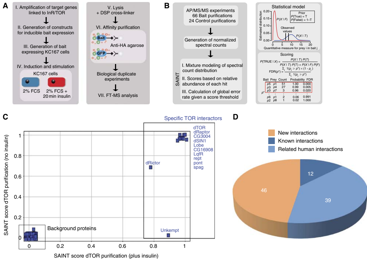
Figure 1 Overview on the experimental workflow and data processing. (A) Experimental workflow. In all, 16 genes linked to dInR/TOR pathway were PCR amplified from cDNA pools. By recombinatorial cloning, the Drosophila ORFs were transferred into an in-house designed expression vector for inducible expression of epitope-tagged bait proteins. Bait expression was induced and cells were starved overnight in 2% FBS. Half of the cell population was exposed to 100 nM insulin for 20 min. The cells were lysed in the presence of DSP cross-linker and bait proteins were purified by anti-HA AP. All AP-MS/MS experiments were performed as two independent replicates. (B) Data processing of the AP-MS/MS data set for detection of specific PPIs using the SAINT algorithm. Following database search, spectrum counts for each identified protein were extracted from the LC-MS/MS data. Based on normalized spectrum counts, SAINT models the spectrum count distribution of each bait-prey interaction and calculates scores based on the relative abundance of each hit. In all, 24 independently control AP-MS experiments (using GFP as a bait protein) were performed in parallel to model false interaction distribution. (C) SAINT scores (data from two biological replicates) were plotted from dTOR purified in the absence (x axis) or the presence (y axis) of insulin to illustrate the specificity increase by the SAINT filtering approach. (D) Overlap with orthologous PPI data and known Drosophila PPIs. The PPI data obtained in this study were compared with available literature and database information covering known D. melanogaster and related Homo sapiens interactions (see also Materials and methods).
