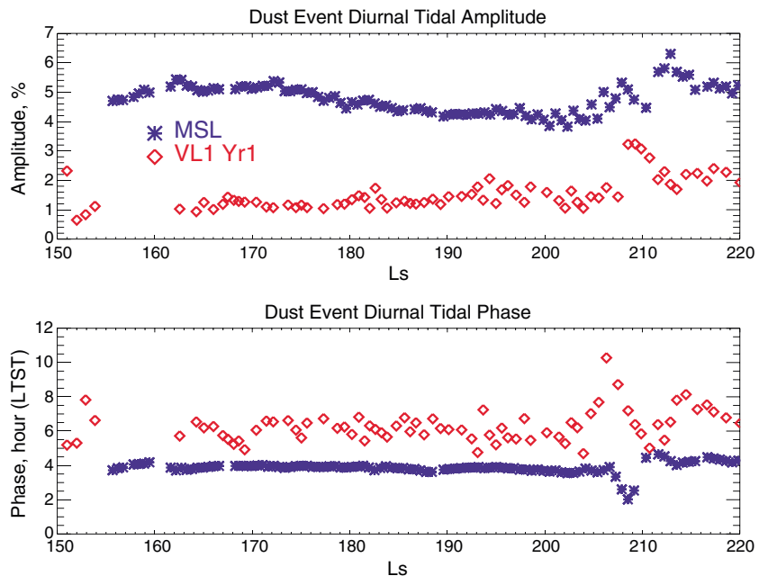
Figure 15. Diurnal amplitude and phase at MSL (blue asterisks) and VL1 Year 1 (red diamonds) for the season corresponding to the first 100 sols of MSL operations.
