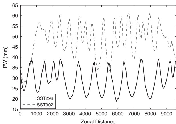
Figure 1. Mean meridional, time-mean zonal PW at equilibrium. SST298 is shown by the solid line and SST302 by the dashed one. Means are taken during the final 10 days.
