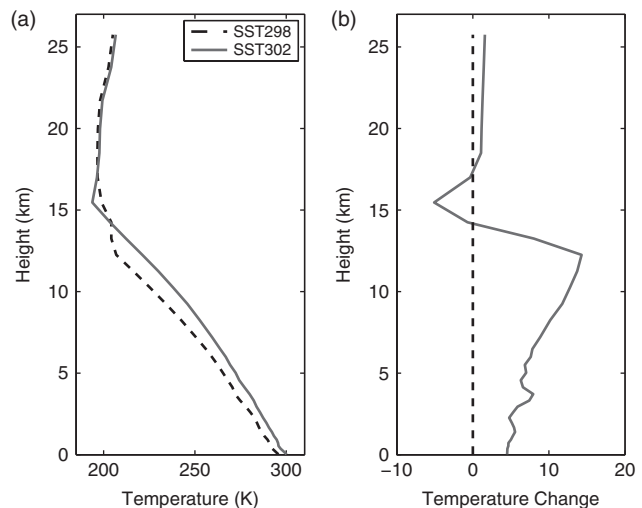
Figure 2. (a) Vertical profiles of domain- and time-averaged temperature from SST298 (dashed) and SST302 (solid). (b) Vertical profile of the averaged temperature differences (SST302–SST298). Positive numbers indicate heights at which the simulation is warmer in SST302.
