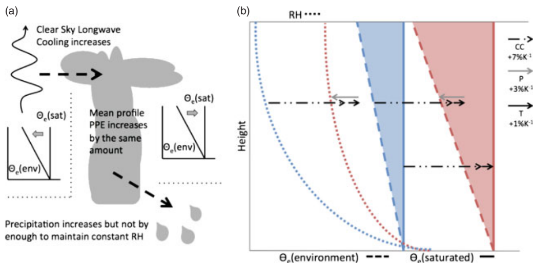
Figure 4. (a) Physical processes related to RH increase and mean PPE. Long-wave cooling increases with SST and serves to destabilize the mean atmosphere. Convection increases to eliminate mean PPE and stabilizes the mean atmosphere. Rain results from PPE release and increases with SST, but too slowly to maintain constant RH (see text). (b) Representative mean quantities for a cooler state in blue and a warmer state in red. Solid lines show the theoretical profile of saturated \theta_e and the dashed lines show the actual environmental \theta_e . The shaded area between the lines is the domain-mean PPE. Horizontal arrows show physical trends between the simulations, with dashed-double dot indicating the contribution from the CC rate, grey that from the precipitation increase and black that from temperature. Trends are shown with respect to surface temperature increases. The dotted lines illustrate the resultant environmental humidity. The figure is illustrative and is not meant to be precisely quantitative.
