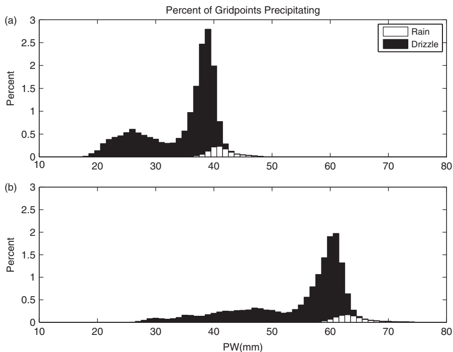
Figure 7. The percentage of surface grid points exhibiting rain (white) or drizzle (black). The upper panel, (a), is for SST298 and the lower, (b), for SST302.
