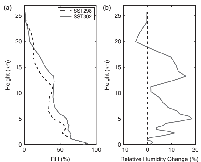
Figure 3. (a) Vertical profiles of relative humidity for SST298 (dashed) and SST302 (solid). (b) Vertical profile of the change in RH with SST.
