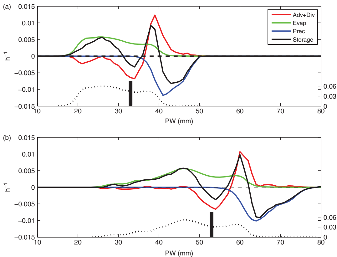
Figure 5. Summed WV flux in \text{h}^{-1} binned by PW. The upper panel is SST298 and the lower SST302. The red line shows contributions from atmospheric motions. Positive (negative) values mean net gains (losses). The green line shows contributions due to evaporation (always positive). The blue line shows evacuation of WV through precipitation (always negative). The black line shows the sum of the previous three. The black bar is the PW value of PW_{\text{thresh}} for each experiment. The black dotted line shows the fraction of the domain occupied by each 1 mm bin of PW read off of the right axis.
