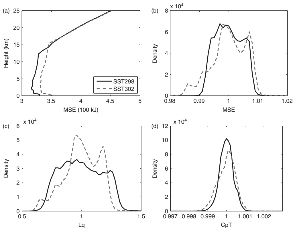
Figure 8. (a) Mean profiles of MSE for SST298 (solid) and SST302 (dashed). (b) PDFs of total column integrated MSE in SST298 and SST302, normalized by their respective means. (c) PDFs of the L_q (moisture) term to the total MSE, again normalized by the model run respective mean. (d) PDFs of the c_p T (temperature) term to the total MSE.
