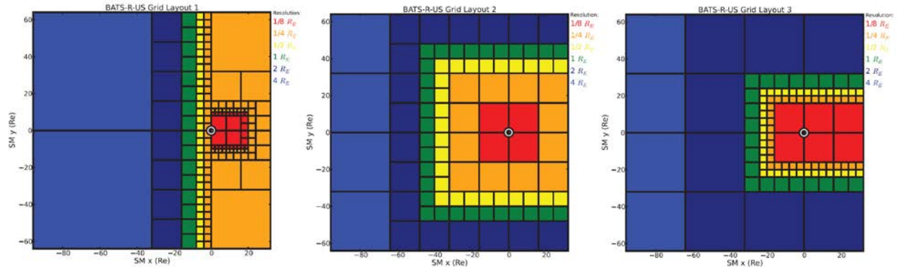
Figure 1 – From left to right, SM xy plane grid resolution is indicated using color for three different grids.
