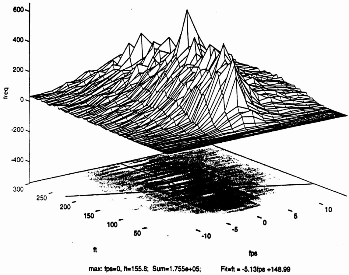
Figure 28. CC loop, CC and N modes, Rdot vs. R
