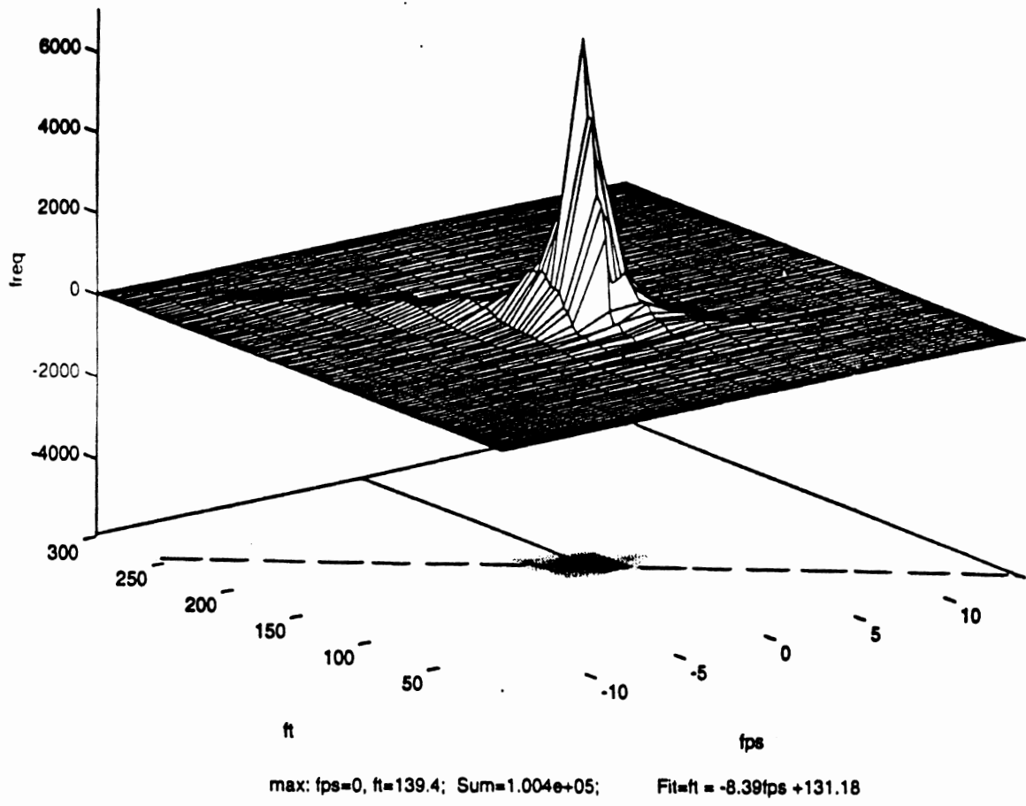
Figure 25. ACC loop, headway control only, Rdot vs. R
