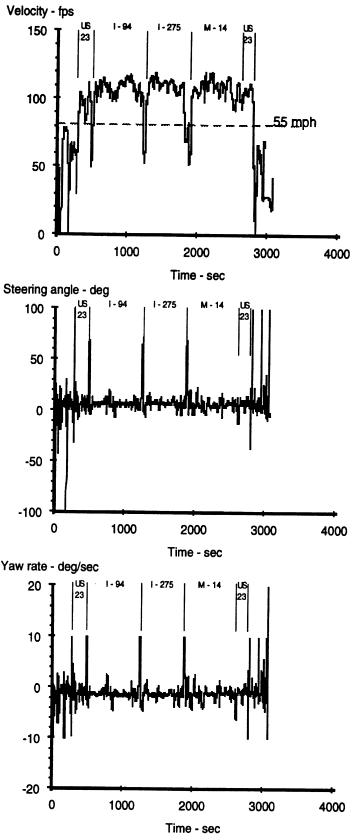
Figure 20. Time histories showing ramp locations
