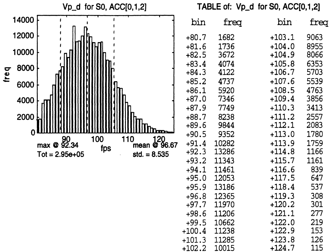
Figure 23. Density of the velocity of the preceding vehicle
