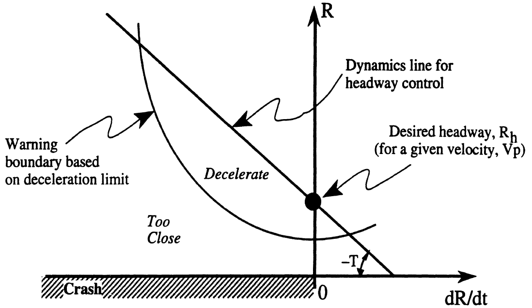
Figure 4. Range-rate versus range diagram.
