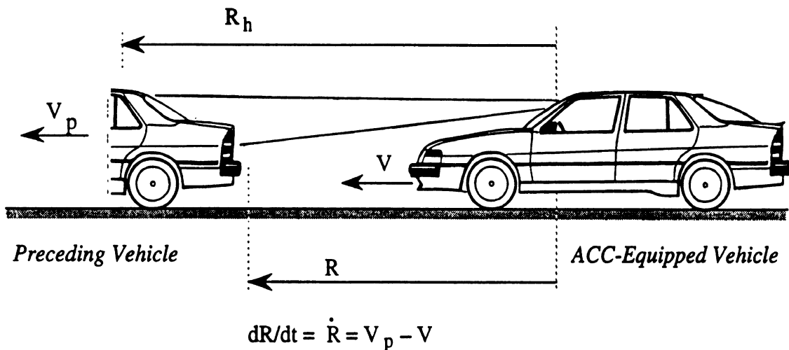
Figure 2. Headway Control
