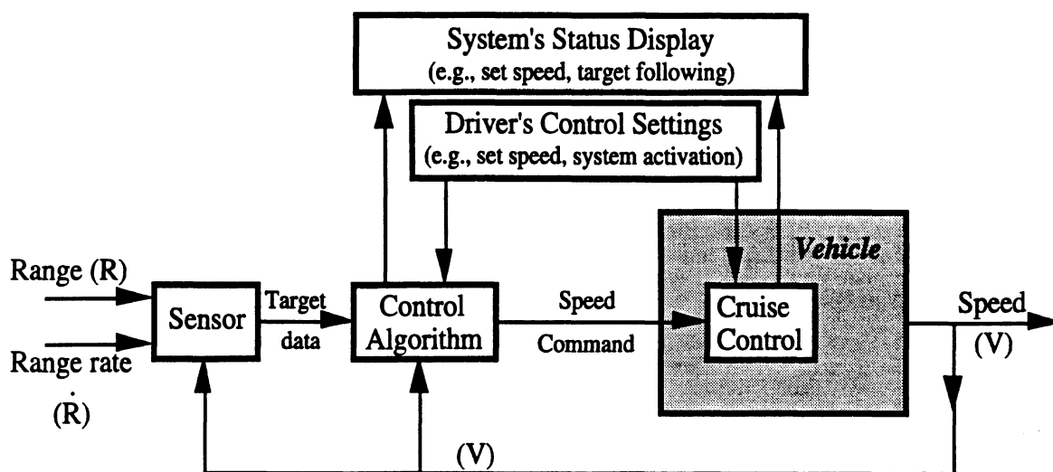
Figure 5. Baseline ACC system structure
