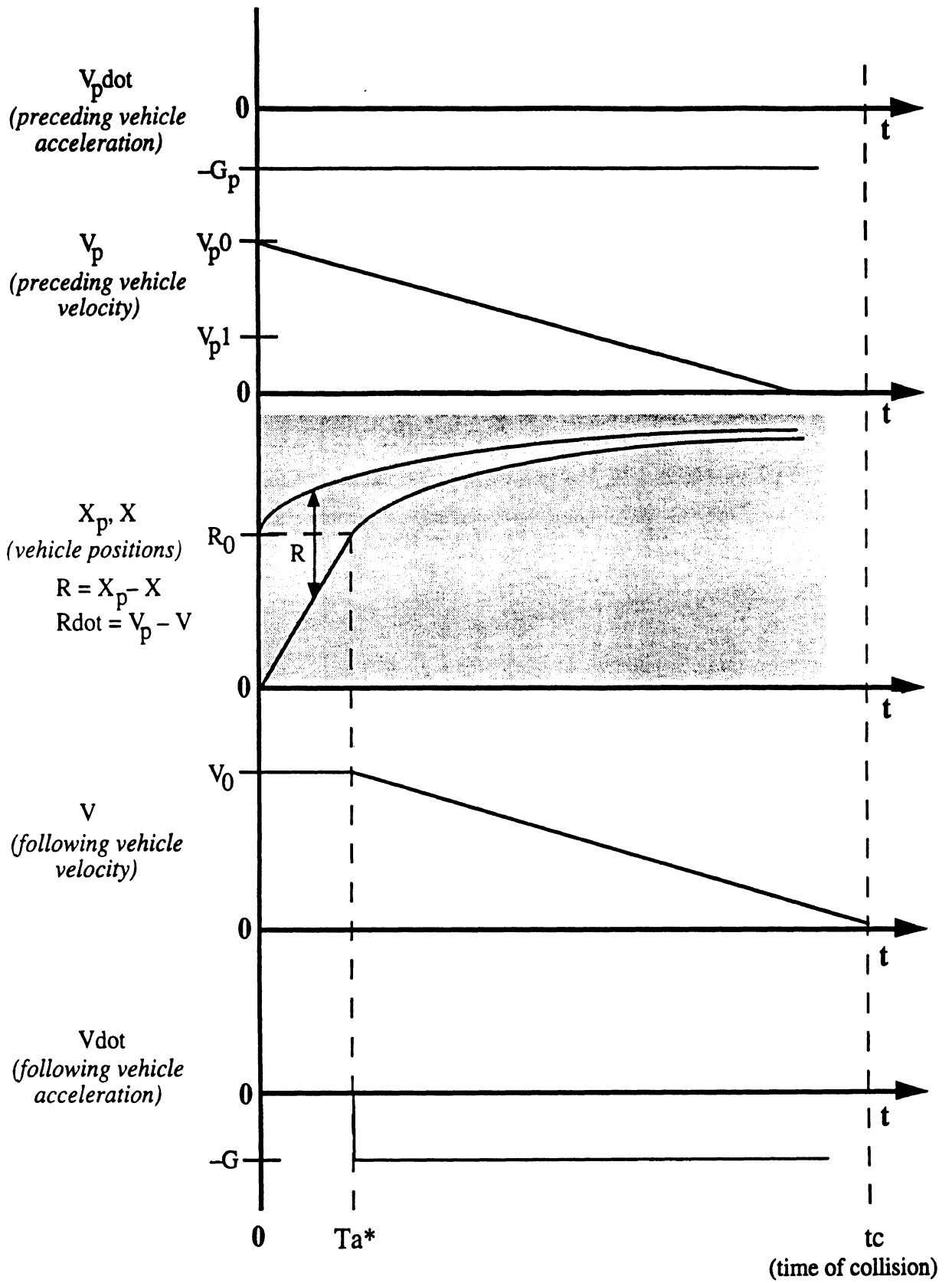
Figure 3. Kinematics of available reaction time and Ta^* .
