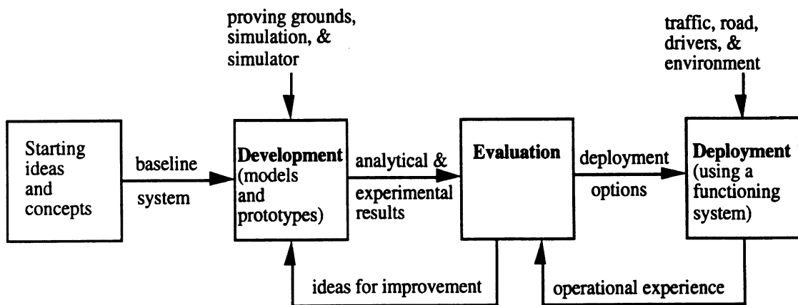
Figure 1. Evolutionary process for fostering forward crash-avoidance systems (FOCAS)
