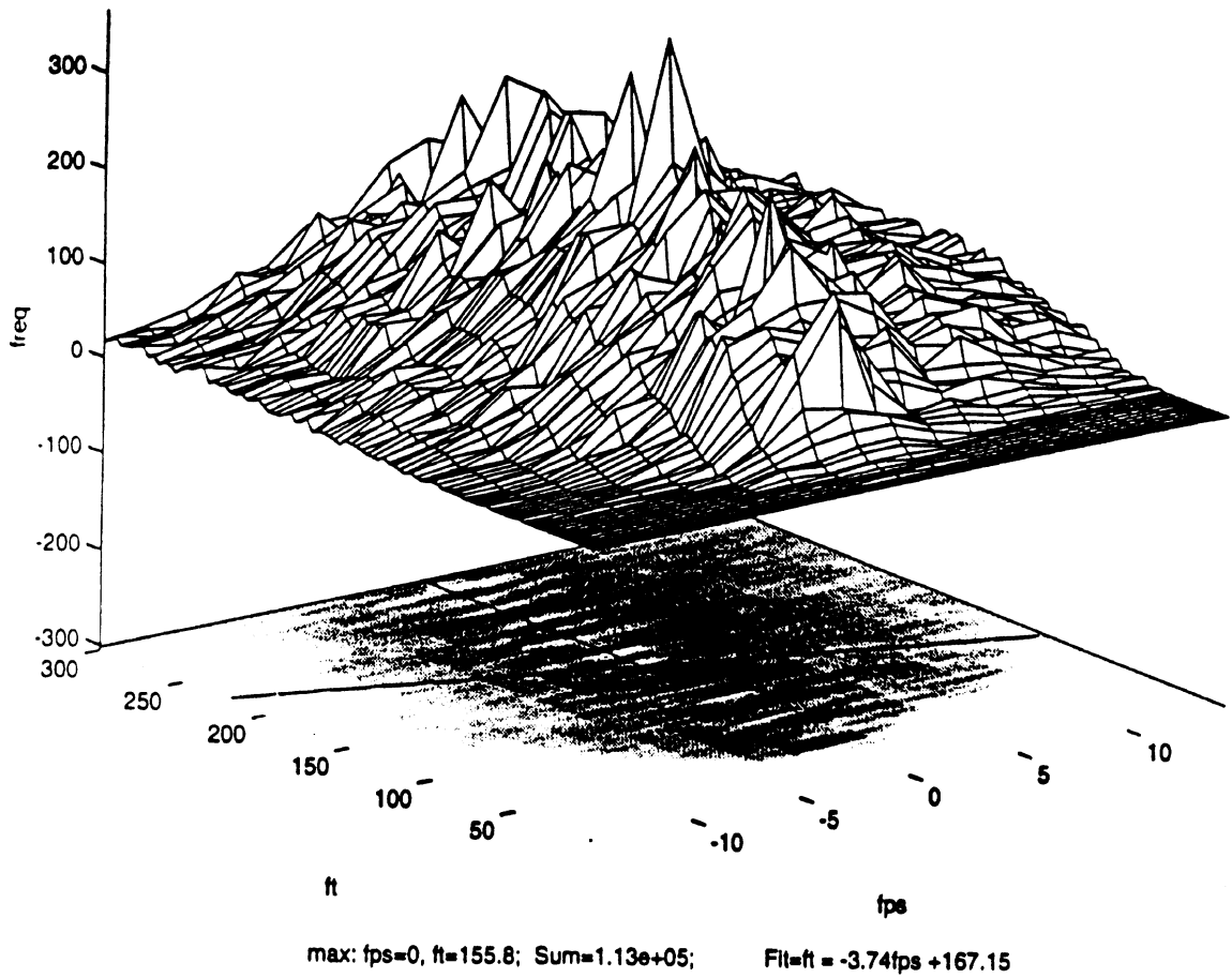
Figure 27 CC loop, CC only, Rdot vs. R
