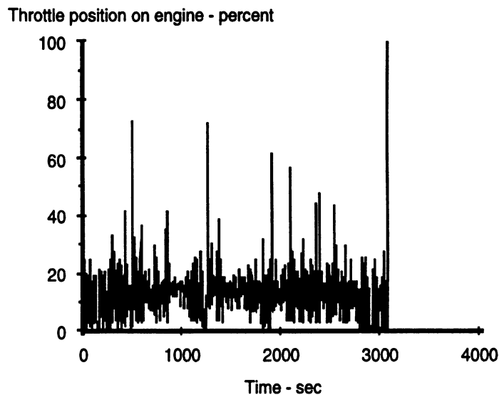
Figure 16. Accelerator pedal position time histories
