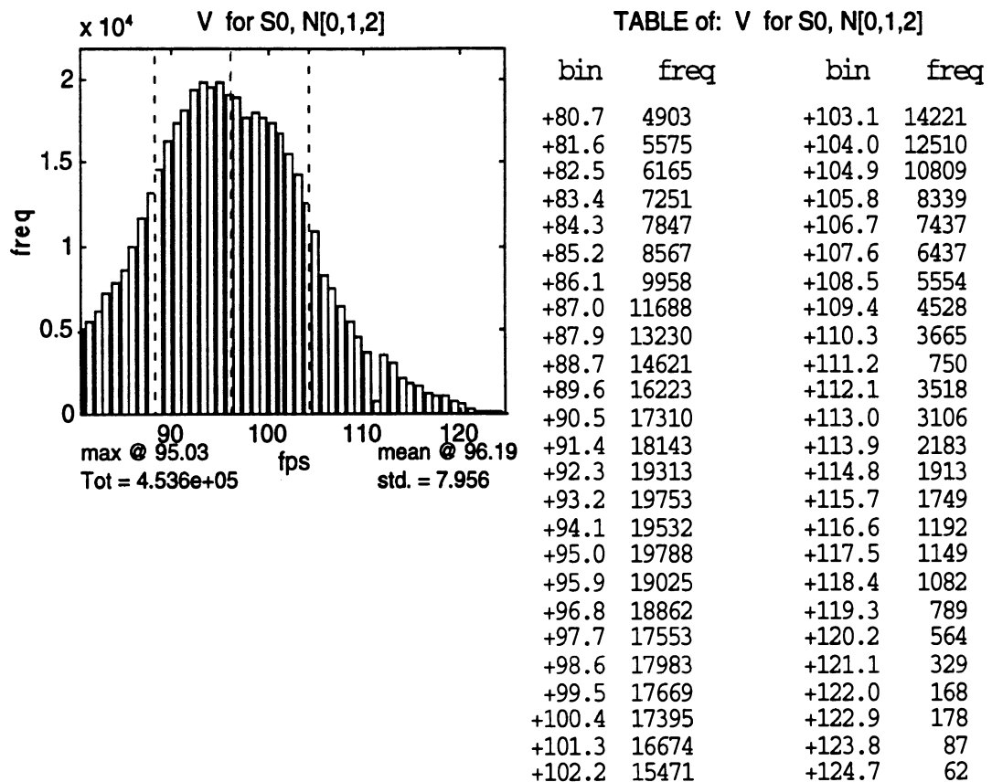
Figure 21. Velocity density histogram
