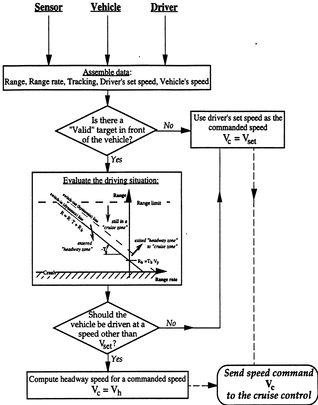
Figure 12. Autonomous Cruise Control algorithm
