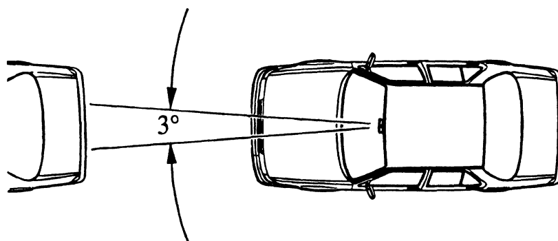
Figure 10. Sensor's field of view
