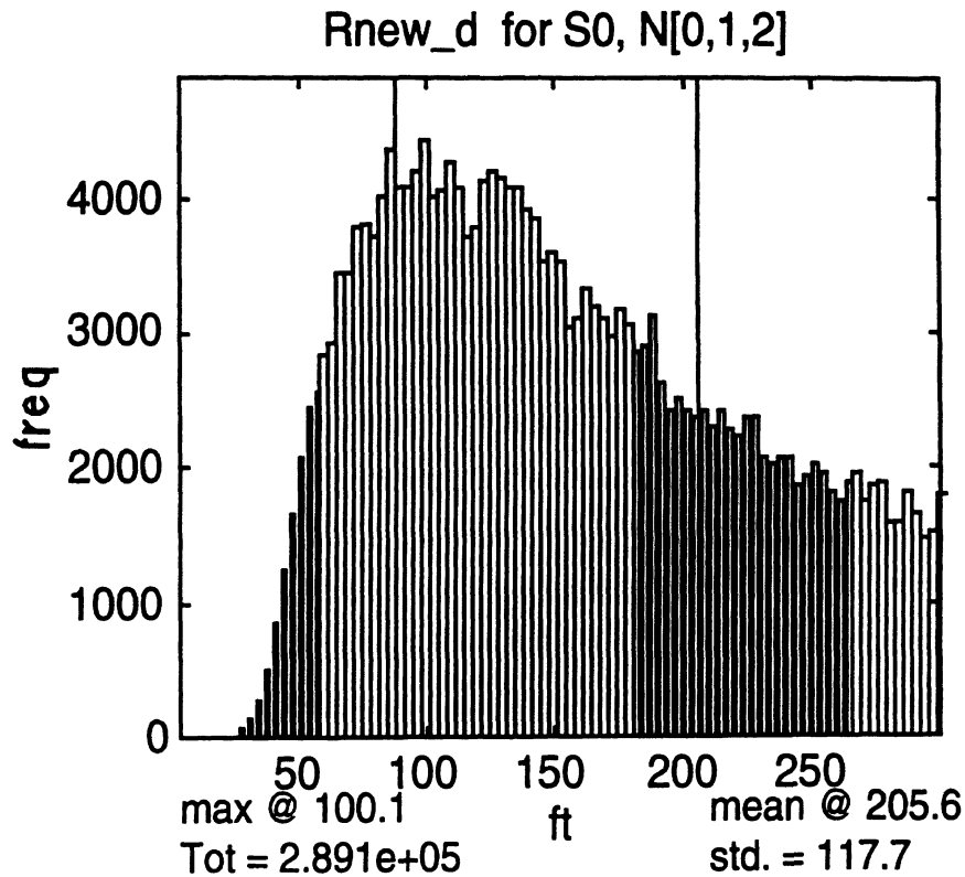
Figure 22. Range density histogram
