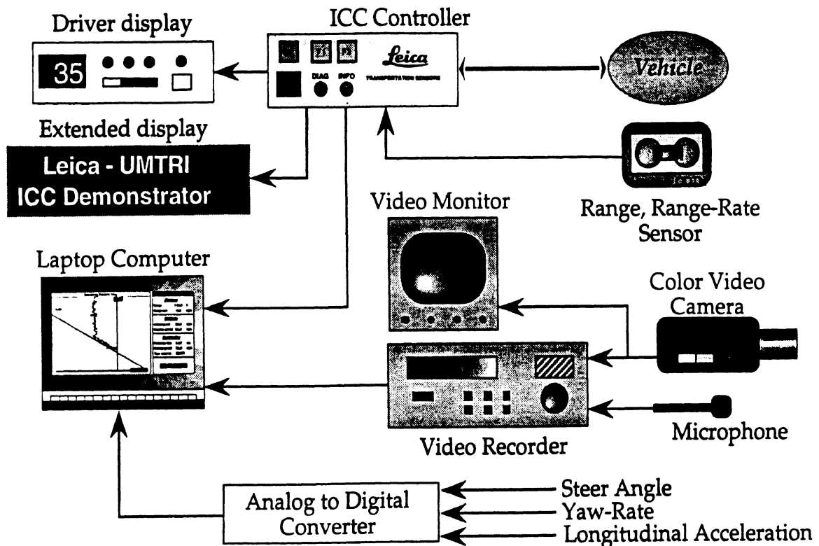
Figure 18. ACC Instrumentation system
