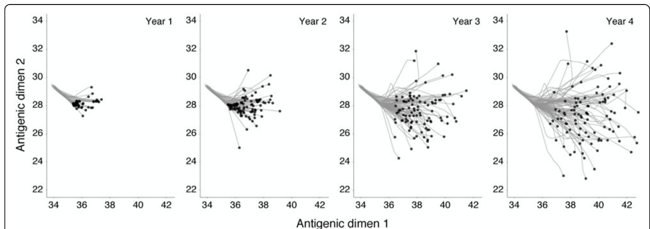
Figure 7 Antigenic phenotypes over the course of 4 years of evolution across 100 replicate simulations starting from identical initial conditions. Replicate simulations were initialized with the end state of the 40-year simulation shown in Figure 2. Each panel shows an additional year of evolution, with black points representing the mean antigenic phenotypes of the 100 replicate simulations and gray lines representing the history of each mean antigenic phenotype.
