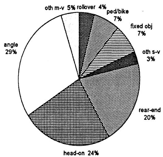
Figure 10 Collision Type Distribution Trucks with Trip Distance > 50 Miles Only 1991-1993 TIFA
