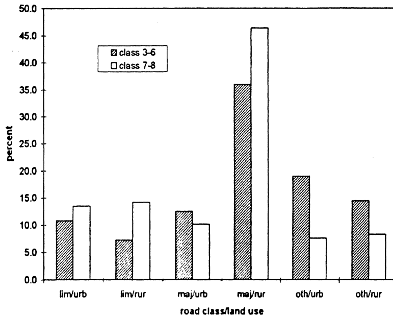
Figure 4 Road Class/Land Use Distribution of Fatal Involvements According to GVWR Class 1991-1993 TIFA
