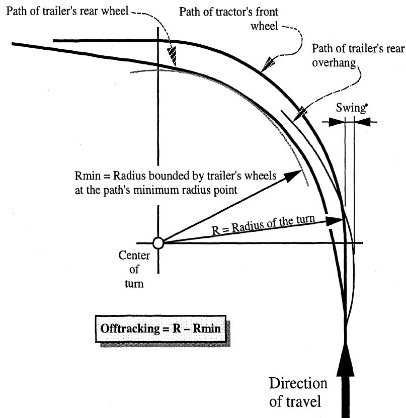
Figure 1. Low-speed offtracking terminology
