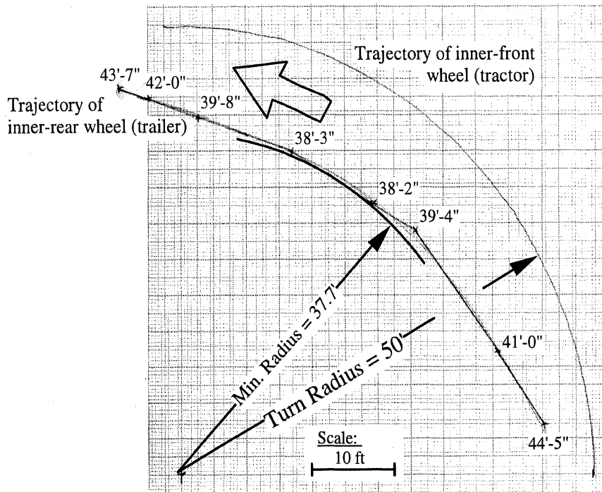
Figure 4. Offtracking experiment — 50 ft turning radius
