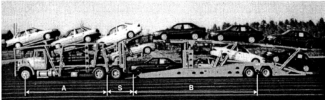
Figure 2. Offtracking and sum-of-squares dimensions
