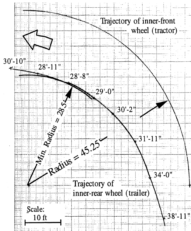
Figure 5. Determining minimum turning radius
