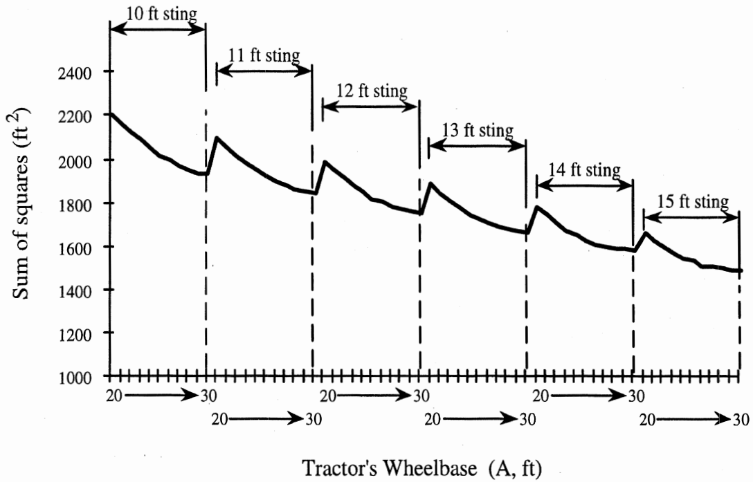
Figure 8. Optimization by sum of squares
