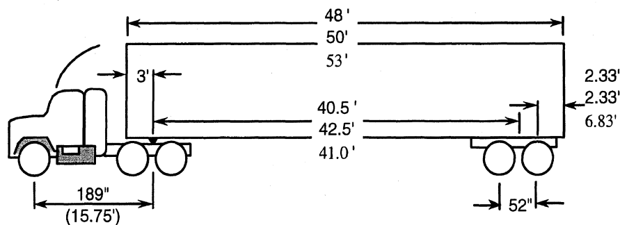
Figure 3. baseline tractor-semitrailer configurations
