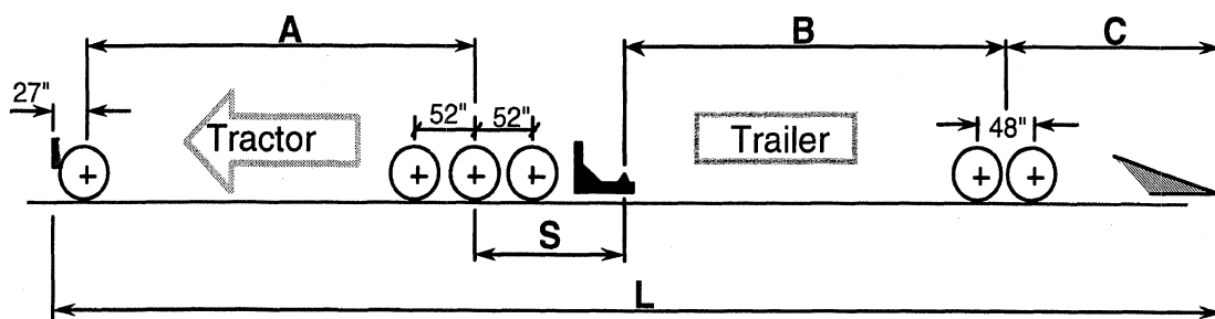
Figure 7. Tridem tractor configuration
