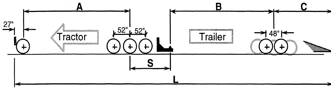
Figure 10. Tridem tractor with a tridem/tandem trailer
