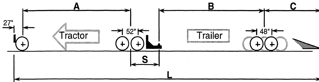
Figure 11. Tandem tractor with a tridem/tandem trailer
