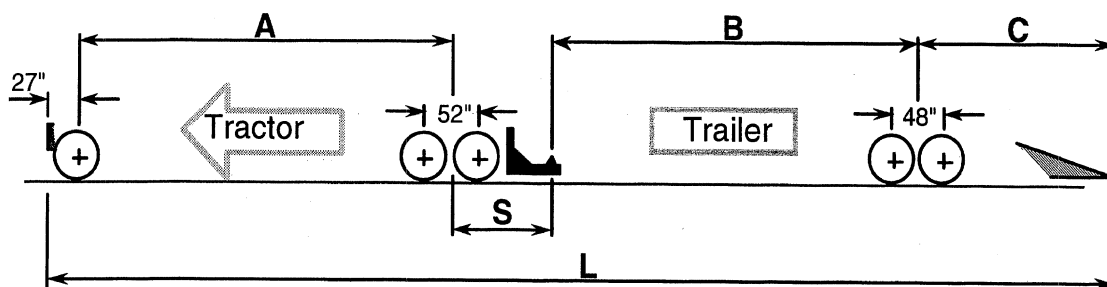
Figure 6. Dimensions template of an automobile transporter
