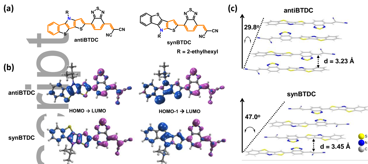
Figure 1. a) Molecular structural formulae of antiBTDC and synBTDC. b) Charge densities of the lowest energy singlet excitations ( S_1 \rightarrow S_0 ) with the given molecular orbital (MO) transitions, where blue denotes occupied, and purple symbolizes unoccupied MOs. c) Crystal packing configurations of antiBTDC and synBTDC. Side chains are omitted for clarity.
