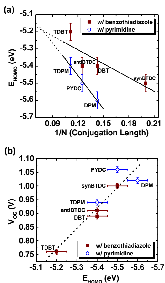
Figure 4. a) Highest occupied molecular orbital energy ( E_{HOMO} ) vs. reciprocal of the backbone conjugation length ( 1/N ) of a series of DTP- and heterotetracene-based d-a-a' donor molecules. b) Open circuit voltage ( V_{OC} ) vs. donor E_{HOMO} for d-a-a':C 70 heterojunctions.
