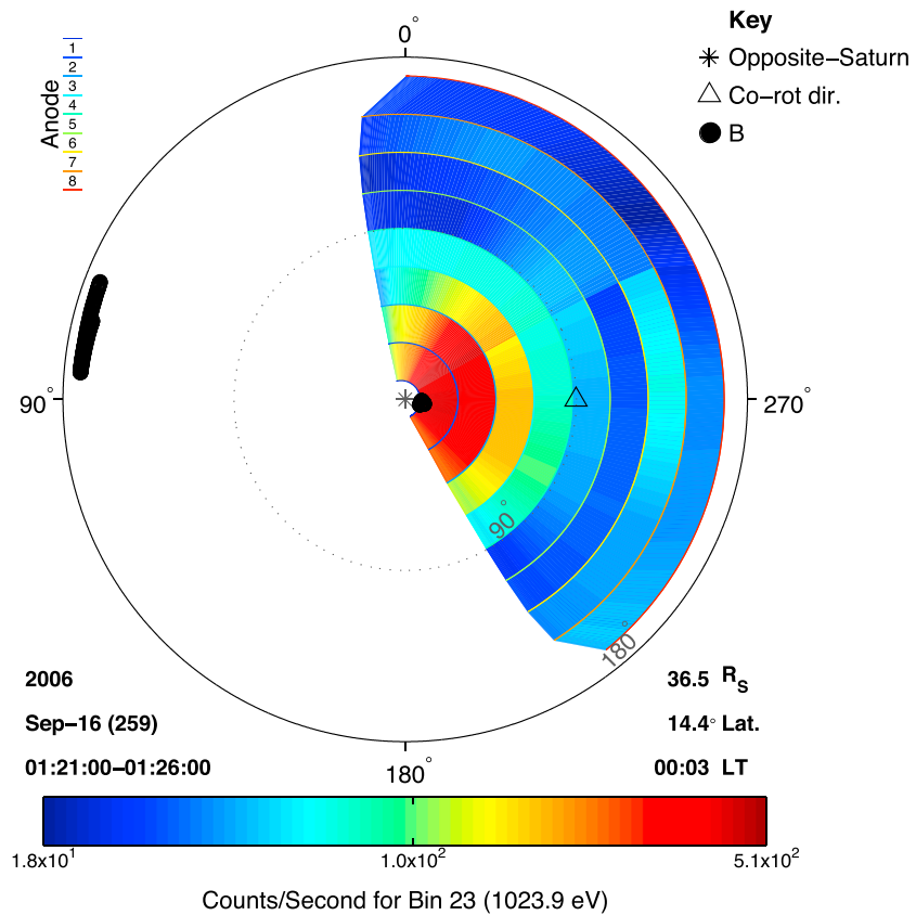
Figure 2. All-sky angular distribution of ions observed by CAPS/IMS between 01:21 and 01:26 UT on day 259, taken at the energy of peak ion counts (1024 eV). The center of the angular distributions corresponds to the look direction away from Saturn, and the open triangle halfway to the outer circle on the right of center corresponds to the look direction into corotation. The counts are sharply peaked in the look direction away from Saturn, corresponding to strong Saturnward flow. The solid black dots show the direction of the magnetic field, and for this interval the flow is nearly field-aligned.
