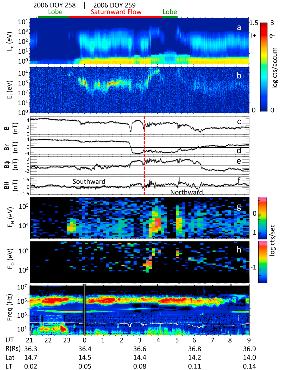
Figure 1. Sunward flowing ion beam event observed by Cassini on 15–16 September 2006 (days 258 and 259) near local midnight at \sim 37 R_s , downtail: (a) Electron count rate (proportional to energy flux) from CAPS/ELS; (b) ion count rate (proportional to energy flux) from the singles (SNG) measurement of CAPS/IMS; (c–f) total strength and KRTP components of the magnetic field observed by MAG, where B_R is positive above the current sheet, B_\theta is positive southward, and B_\phi is positive in the corotation direction; (g) H+ and (h) O+ count rate spectrograms from MIMI/CHEMS; and (i) electric field power spectrum from RPWS. The bright emissions above \sim 10^4 Hz in Figure 1i are identified as SKR. The colored bars above Figure 1a show the lobe intervals and the interval in which a Saturnward ion flow was observed. The vertical red dashed line in Figures 1c–1f marks the transition to higher beam energies and a return to significant water-group composition.
