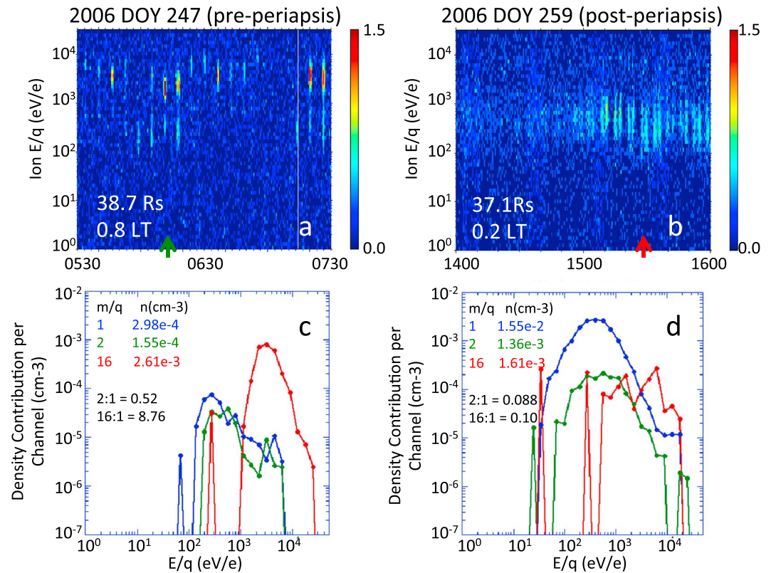
Figure 7. (a) Ion energy-time spectrogram for a preperiapsis crossing of the current sheet, showing the clear presence of two separate ion species ( W^+ at higher energies and light ions at lower energies). (b) Similar spectrogram for a postperiapsis crossing of the current sheet. Only a light-ion peak is visible. (c) Contribution to the total density of each species from each of the IMS energy channels, based on TOF measurements averaged over the interval covered in Figure 7a. Total densities are the sum of the plotted contributions. Water-group ions are the dominant population, consistent with typical magnetospheric plasma observations. Ions with m/q = 2 also have typical abundance for the outer magnetosphere. (d) Same as Figure 7c but for the interval in Figure 7b. Water-group ions are extremely tenuous, and ions with m/q = 2 have abundance much more similar to the solar wind than to typical magnetospheric plasma.
