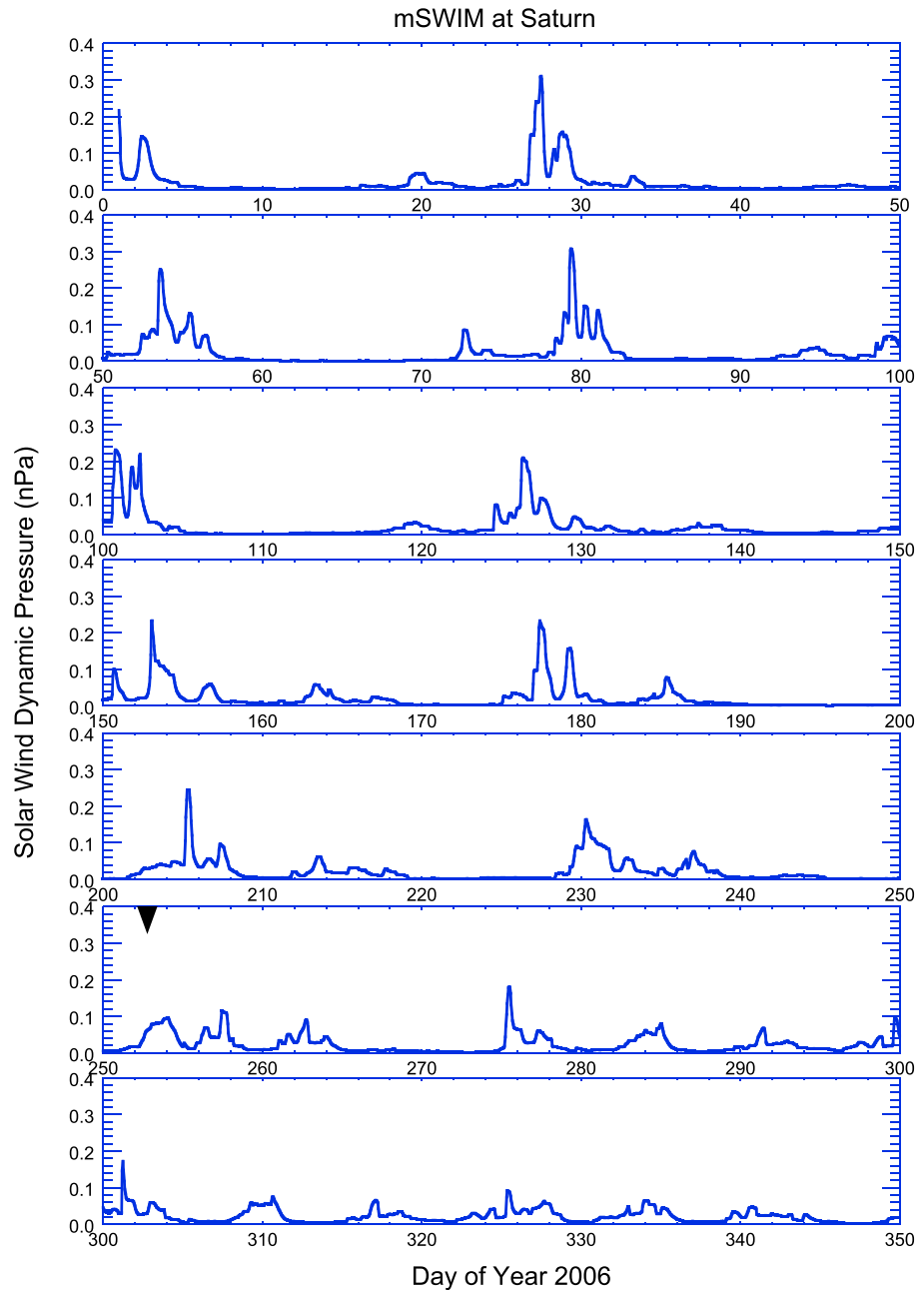
Figure 9. Stack of 50 day plots of the solar wind dynamic pressure at Saturn predicted by mSWIM for the year 2006. For most of the year there was one prominent high-pressure stream during each solar rotation (~25 days). Near the end of the year, this recurrent stream structure evolved into three somewhat weaker streams. The arrow in the second panel from the bottom marks the Cassini periapsis immediately preceding the ion flow interval on days 258 and 259.
