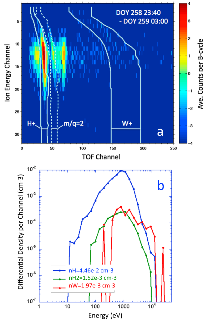
Figure 3. (a) Ion counts observed by CAPS/IMS, sorted according to their energy and time of flight (TOF) in the instrument. Pairs of curves labeled H+, (m/q = 2), and W+ indicate the range of TOF at each energy level that is populated by these species. The prominent peak below TOF ~ 30 is an instrumental artifact, and the population near TOF ~ 70 results from incident ions that strike the LEF MCP (see Thomsen et al. [2010] for a more complete discussion). The plot includes all the TOF data obtained during the ion beam event of Figure 1, from 23:40 UT on day 258 to 03:00 UT on day 259. (b) Contribution to the total density of each species from each of the IMS energy channels averaged over the interval covered in Figure 3a. Total densities are just the sum of the plotted contributions.
