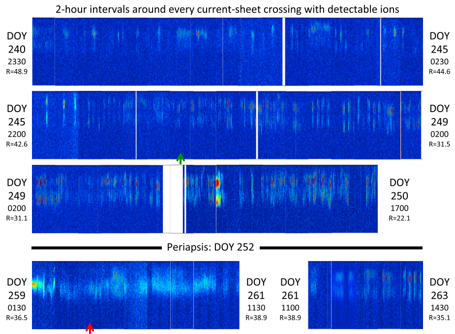
Figure 8. Concatenated 2 h ion energy-time spectrograms for all the current-sheet crossings between the end of day 240 and the middle of day 263, and for which detectable ions were present in CAPS. The green and red arrows indicate the intervals highlighted in Figure 7. Prior to periapsis (above the black horizontal bar), the ion distribution was characterized by two clear peaks in energy. After periapsis (below the bar), most of the distributions up until the middle of day 261 showed dominantly light ions, with little evidence for W+. After midday on day 261, the distribution returned to its preperiapsis character.
