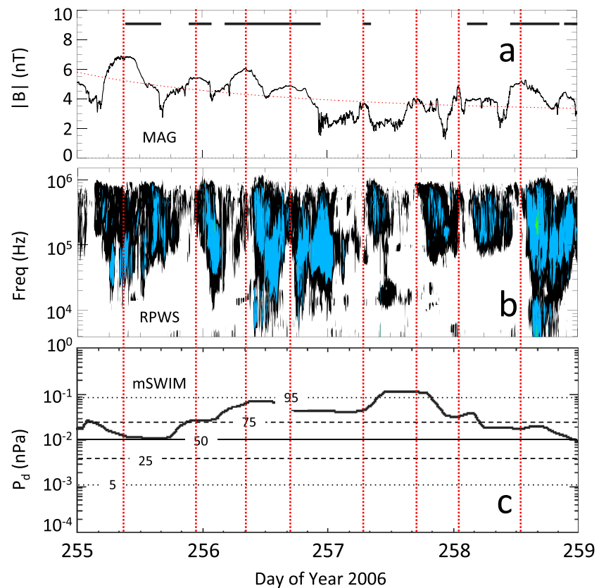
Figure 6. Same as Figure 5, for day 255 to day 259. SKR enhancements occur shortly after peaks in the magnetic field intensity, which are indicated by the vertical red dashed lines.
