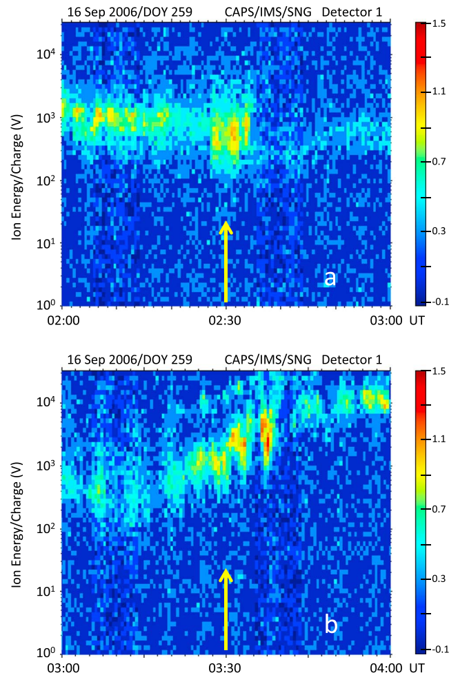
Figure 4. (a) Energy-time spectrogram of non-mass-resolved ions (SNG) observed by CAPS/IMS for 1 h centered on the current sheet crossing at ~02:30 UT on day 259. There is a clear peak at ~600 eV corresponding to flowing H + , but no similar peak at ~10 keV, where one might expect co-flowing W + to appear. (b) Similar SNG spectrogram for the hour encompassing the strong energization (both inferred flow speed and temperature increased) after ~03:20 UT on day 259. Plasma during this energization event had a clear contribution from co-moving W + , ~10–20 times the H + peak energy.
