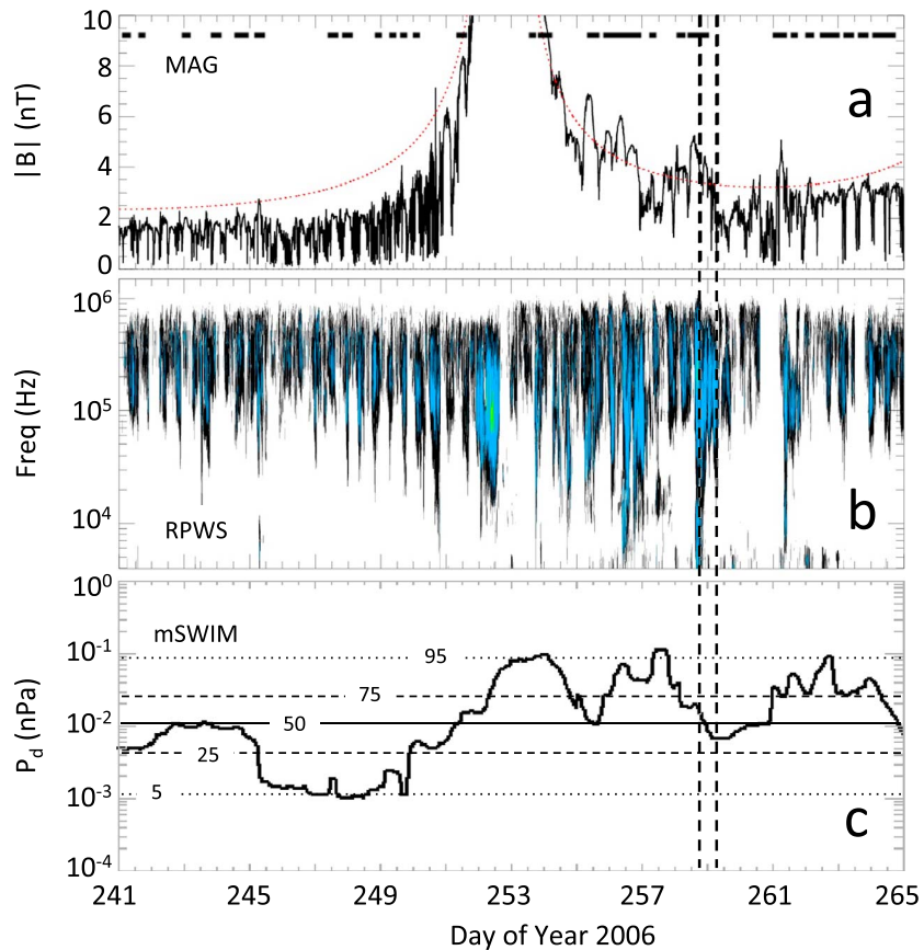
Figure 5. (a) Magnetic field magnitude and (b) electric field power spectrum observed by Cassini over a 24 day interval containing the ion beam event of Figure 1 (marked by vertical dashed lines). The red dashed curve in Figure 5a is the average lobe magnetic field magnitude determined by Jackman and Arridge [2011a], and the black bars at the top of that panel show times when Cassini was actually in or very near the lobe, based on CAPS/ELS electron observations. (c) Solar wind dynamic pressure predicted at Saturn for the same interval based on calculations of the mSWIM MHD model [ Zieger and Hansen, 2008 ]. Horizontal lines indicate the various percentile values of the dynamic pressure calculated with this model for the entire year of 2006.
