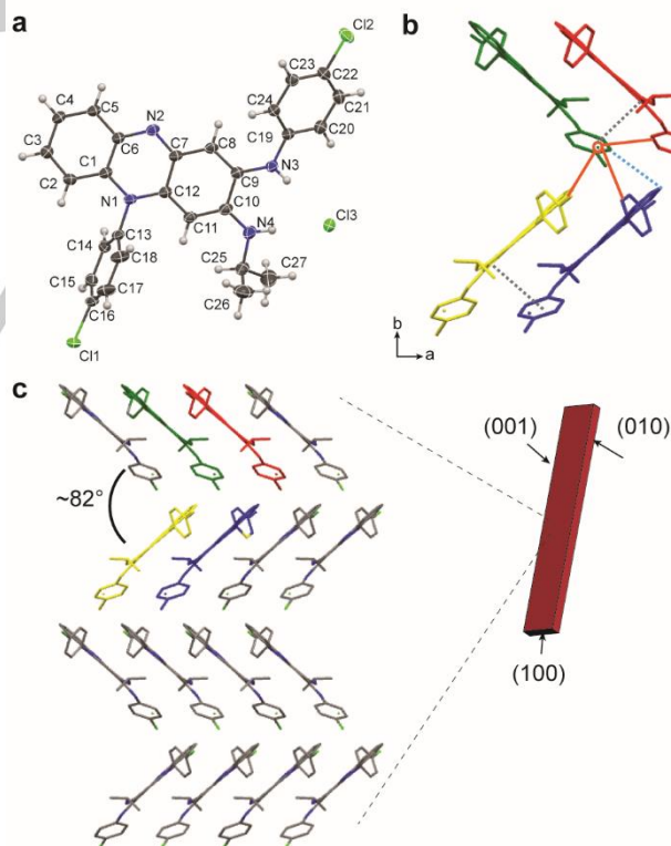
Figure 3. a) Asymmetric unit of CFZ-HCl displayed as an ellipsoid plot with 50% probability. The atomic positions for all non-hydrogen atoms are labeled. b) One section of the corrugated packing with solid orange lines indicating C-H...Cl interactions, C-H... \pi indicated with a light blue dotted line and \pi ... \pi interactions indicated with light grey dotted lines (unit cell looking along the c-axis). The molecules are displayed as capped sticks with the hydrogen atoms removed for better visualization of the crystals packing. c) Crystallographic projections of packing along the (001) face showing the corrugated packing. The projection is made up of 2 \times 2 \times 0.5 ( a \times b \times c ) unit cells.
