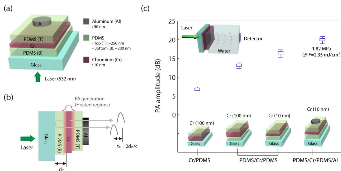
Figure 1. a) Metal film-based photoacoustic (PA) transmitter structure consisting of a Cr layer (10 nm) sandwiched by two thin PDMS layers. The Al layer (50 nm) serves as an optical reflector constituting an optical resonance cavity. Light is illuminated from the glass side. b) Illustration of detailed PA generation. Two oppositely-propagating PA pulses are produced in the heated regions. The two PA pulses have a delay time corresponding to twice the acoustic transit time across the bottom PDMS layer. c) PA signal amplitudes for different structures, normalized to the bare Cr (100 nm) on a glass substrate. The PA amplitude of the optimized structure is 1.82 MPa at a laser fluence of 2.35 mJ/cm 2 .
