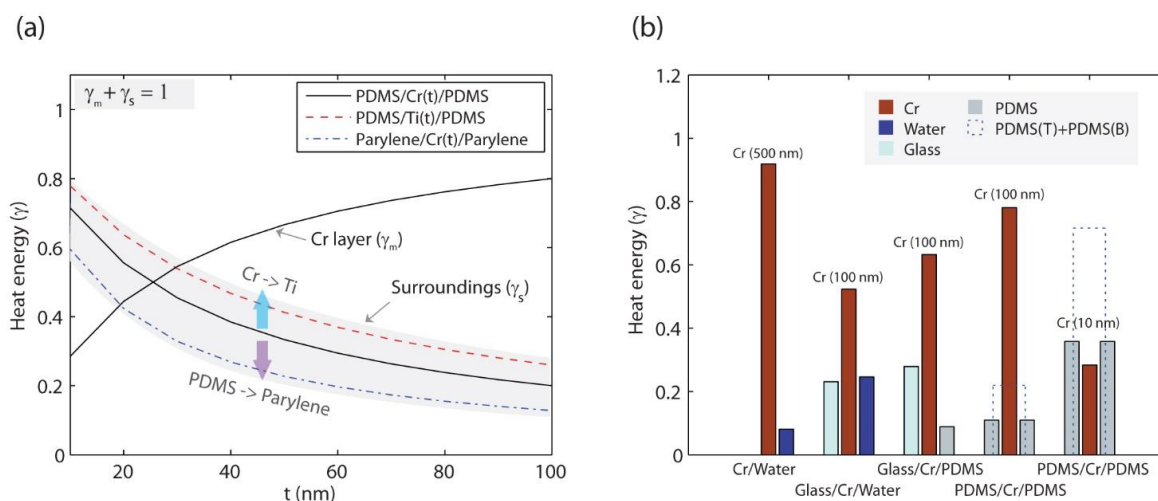
Figure 4. The calculated heat energy in each layer during laser excitation (pulse duration: 5 ns). a) The heat energy as a function of the metal thickness for the structure (PDMS/Cr/PDMS, solid line). The heat energy in Cr increase, while the combined heat energy in the PDMS layers decreases. The heat energy in the surrounding layers increases by replacing Cr with Ti (red dashed line), but decreases by replacing PDMS with parylene. b) The heat energy for different structures.
