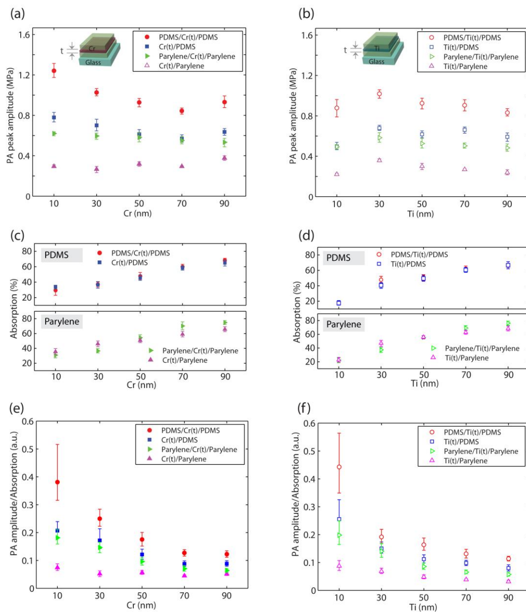
Figure 3. The measured photoacoustic (PA) amplitude as a function of metal layer thickness for Cr (a) and Ti (b). The light absorption for Cr (c) and Ti (d). The light absorption increases with the metal absorber thickness. The PA amplitude normalized to the light absorption for Cr (e) and Ti (f). The normalized PA amplitude decreases with the metal absorber thickness.
