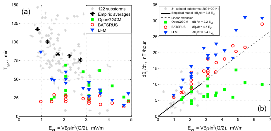
Figure 3. Analysis of the (a) growth phase duration and (b) lobe magnetic field loading rate as a function of the merging electric field E_{KL} in three GMHD models compared with the empirical data. Grey points show the spread of individual events, black stars indicate the derived average values, black lines in Figure 3b correspond to the average linear slope in the observation-based relationships.
