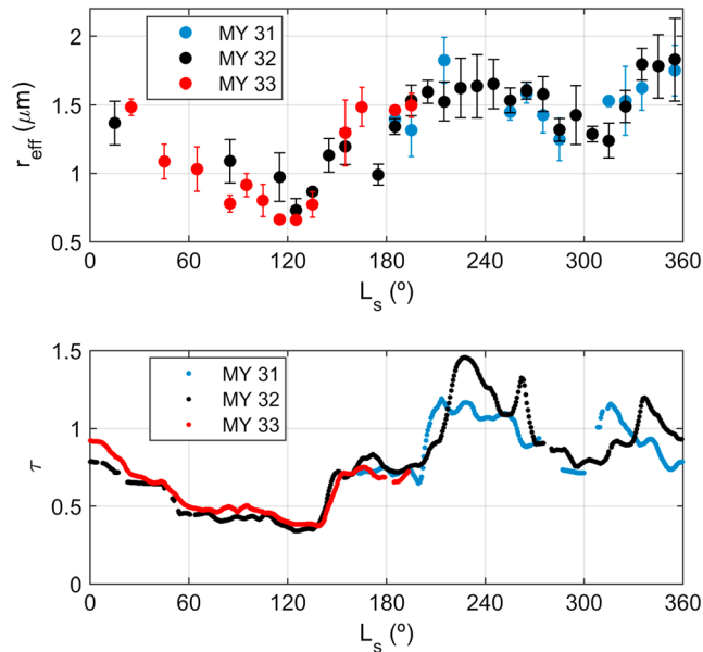
Figure 2. (top) Seasonal variability of dust aerosol particle effective radii for MY 31 (blue), 32 (black), and 33 (red). (bottom) Seasonal variability of averaged Mastcam atmospheric opacity for MY 31 (blue), 32 (black), and 33 (red).
