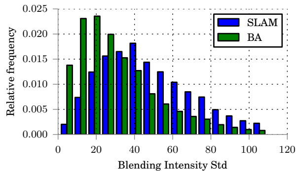
Figure 15: Histogram of intensity deviation for the results shown in Fig. 14. The y-axis displays normalized frequency counts across the whole model. Note the greater quantitative consistency of the the proposed approach (titled BA). There are many more occurrences of great pixel deviation in the authors' previous work (titled SLAM) which does not have global bundle adjustment applied.
