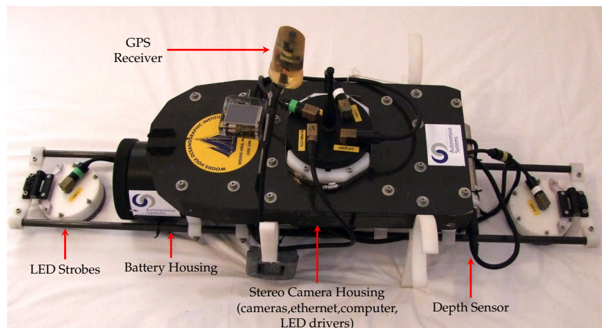
Figure 1: The stereo-vision diver-rig and list of components
