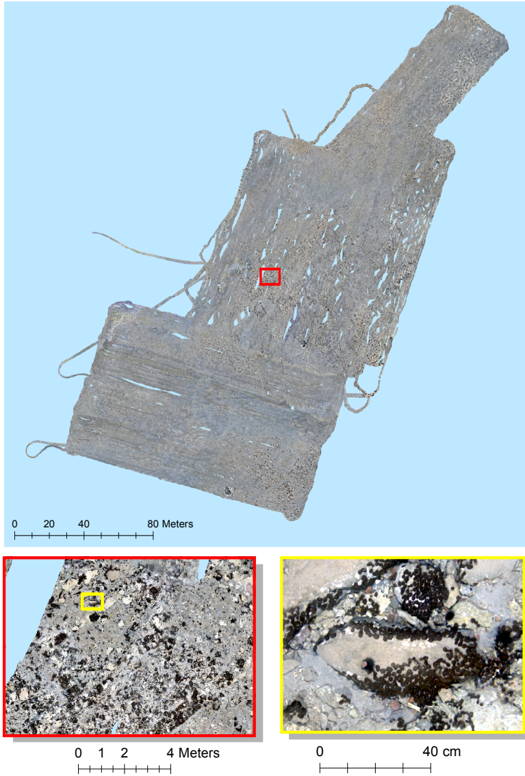
Figure 17: 3D model from the 2011 field season. This model is the result of a bundle adjustment of approximately 400,000 Iver2 gathered images into a large scale 3D model in which individual stones can be seen and mapped across the entire site.
