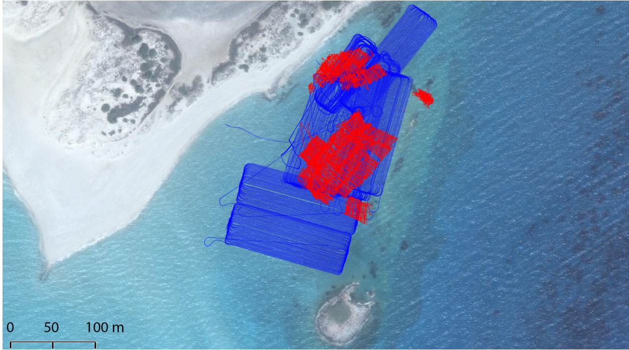
Figure 9: Vehicle trajectories: the blue line denotes the path of the Iver2 while the red line denotes the path of the diver-rig missions. The vast majority of the site was fully covered using the two technologies by the end of the 2011 field season.
