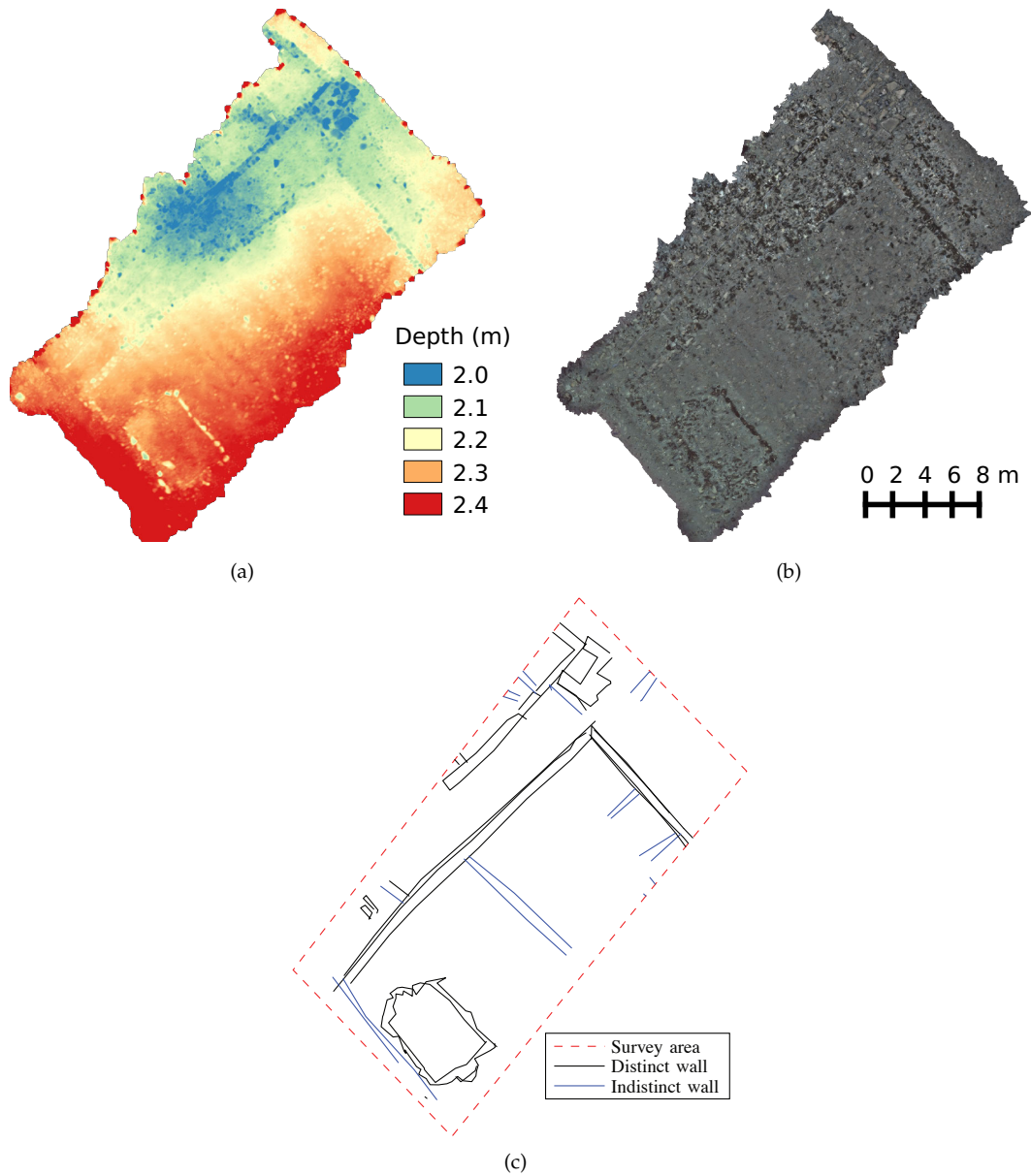
Figure 10: Map of the survey area of from three separate dives using the diver-rig. Remains of walls are clearly visible in both the depth colored view (a) and the texture mapped view (b). The corresponding map produced by the Total Station system (c) shows good agreement in the layout of the features of the site.
