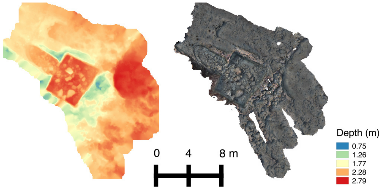
Figure 11: Chamber tomb mesh. The chamber is approximately 4 \times 5 \text{ m}^2 in size, and has been cut to a depth of 3 m from the surrounding rock.
