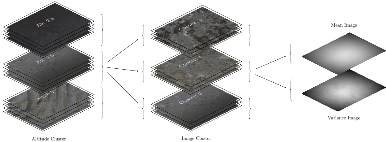
Figure 3: A diagram depicting the two-level clustering process used in image correct, first a division by imaging altitude, then a division by estimated bottom type using a Variational Dirichlet Process (VDP) clustering algorithm (Steinberg et al., 2011, 2013). After the creation of all these subsets the mean and variance for each pixel location in each subset is computed. A gain and offset is then calculated using the standard grey-world algorithm (Buchsbaum, 1980).
