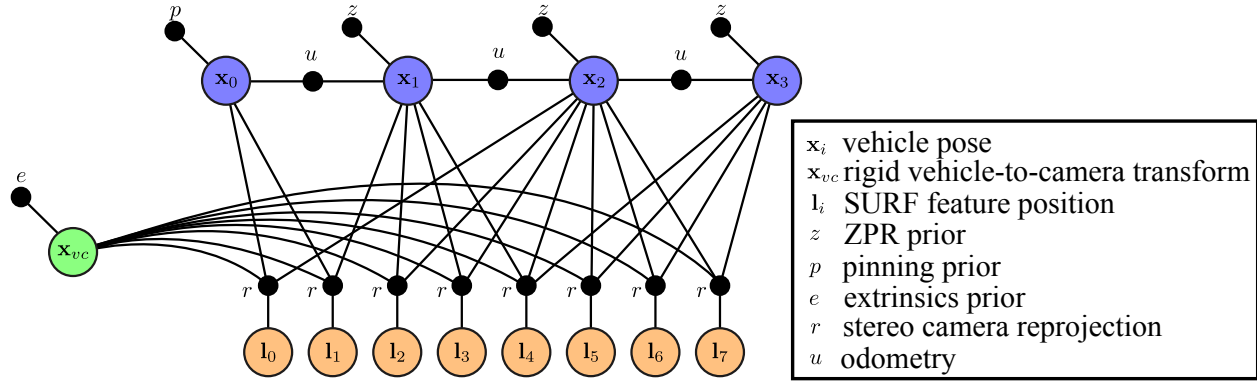
Figure 6: Small example using a factor-graph to graphically represent the estimation of pose (blue nodes) and 3D structure (orange nodes). Besides the usual depth, pitch and roll (ZPR) and odometry measurements, we use ternary factors connected to 3D features, l_0 \dots l_7 , to also constrain the estimate of the vehicle-to-camera rigid body transformation, x_{vc} . The final estimate of the vehicle poses, x_0 \dots x_3 , are fed into a mesh reconstruction and texturing algorithm.
