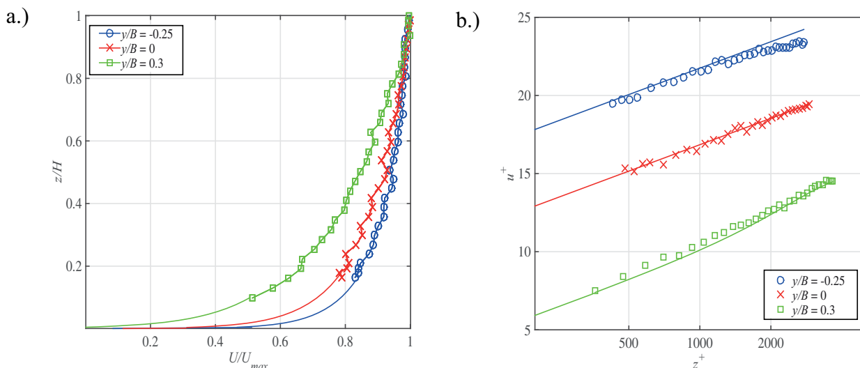
Figure 2. Rough bed case, H = 0.20 m, U_b = 0.22 m/s. (a) Normalized velocity profiles at y/B = -0.25 (over glass bed) with \delta^* = 20.9 mm, y/B = 0 (channel centerline) with \delta^* = 25 mm, and y/B = 0.3 (over rough bed) with \delta^* = 47.8 mm. Markers indicate measured points, and smooth lines below z/H < 0.2 designate the log-law extrapolated results to the bed. (b) Vertical velocity profiles plotted in wall coordinates. Lines indicate log-wake fit.
