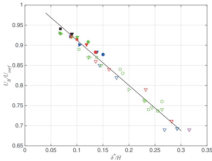
Figure 5. Index velocity versus displacement thickness normalized by the flow depth. Magenta symbols, H = 0.06\text{--}0.08 m; Blue symbols, H = 0.10\text{--}0.11 m; Red symbols, H = 0.15\text{--}0.16 m; Green symbols, H = 0.20\text{--}0.21 m; Black symbols, H = 0.31 m. Circle, U_B = 0.05 m/s; inverted triangle, U_B = 0.09\text{--}0.1 m/s; square, U_B = 0.23\text{--}0.24 m/s; right-facing triangle, U_B = 0.33\text{--}0.35 m/s. Filled-in symbols indicate smooth bed cases and hollow symbols indicate rough bed cases. Solid line: y = -1.12(x) + 1.03 , R^2 = 0.96 .
