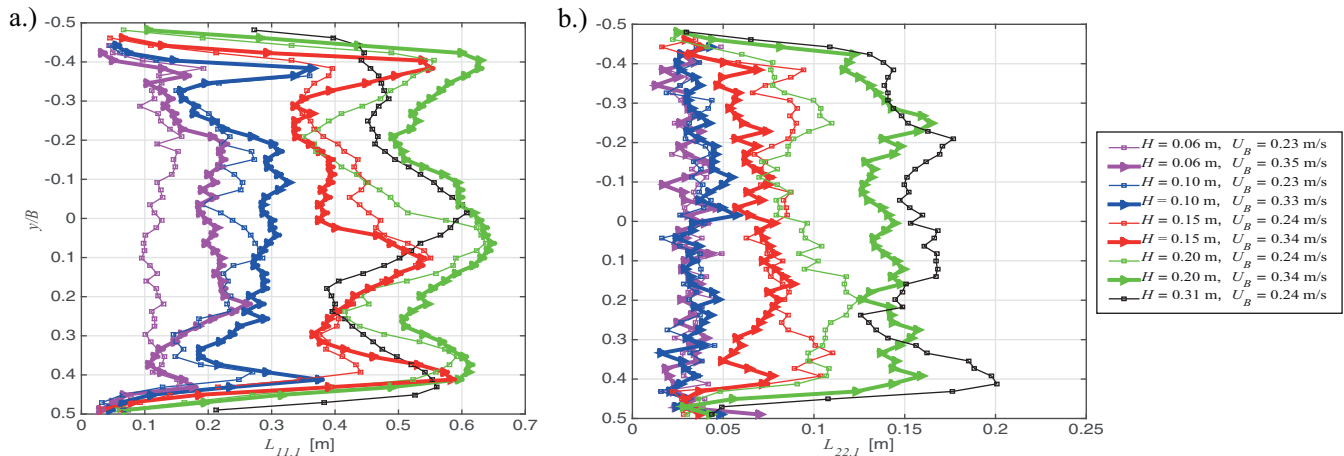
Figure 7. Smooth bed cases. (a) Streamwise integral length scale, L_{11,1} versus nondimensional channel width. (b) Transverse integral length scale, L_{22,1} versus nondimensional channel width.
