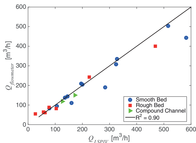
Figure 12. Measured versus predicted volumetric discharge.
