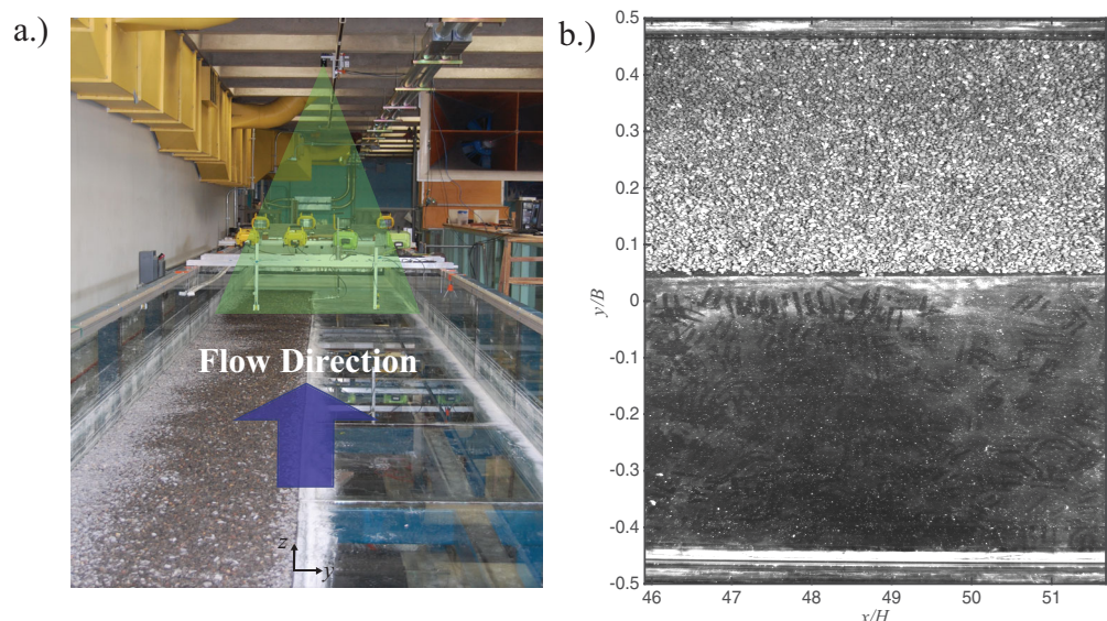
Figure 4. (a) Rough bed experimental setup. (b) Rough bed camera field-of-view.
