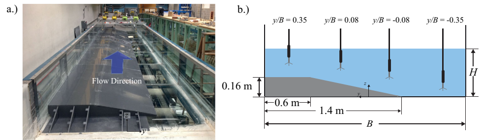
Figure 3. (a) Compound channel experimental setup. Note: front cover of the false-bottom insert has been removed to reveal the cross section. (b) Compound channel schematic with ADV measurement positions indicated.
