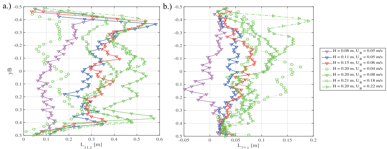
Figure 10. Rough bed cases. (a) Streamwise integral length scale, L_{11,1} versus nondimensional channel width. (b) Transverse integral length scale, L_{22,1} versus nondimensional channel width. U_B values reported in the legend correspond to depth-averaged velocities measured over the rough bed.
