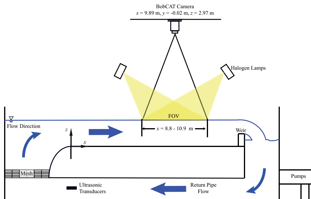
Figure 1. Schematic of recirculating wide-open channel flume.
