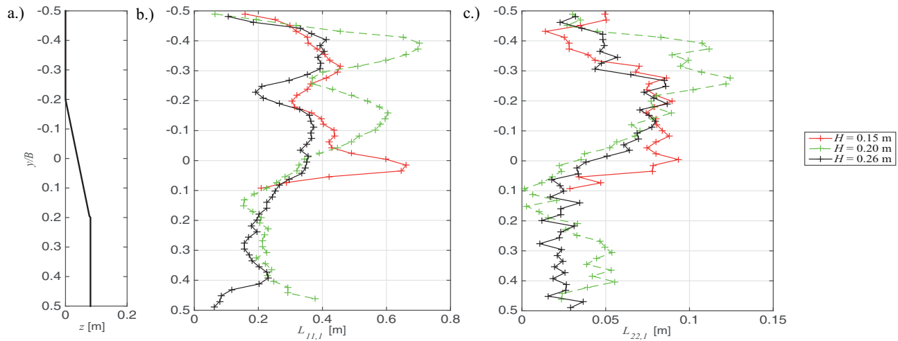
Figure 9. Compound channel cases. (a) Compound channel cross section. (b) Streamwise integral length scale, L_{11,1} versus nondimensional channel width. (c) Transverse integral length scale, L_{22,1} versus nondimensional channel width.
