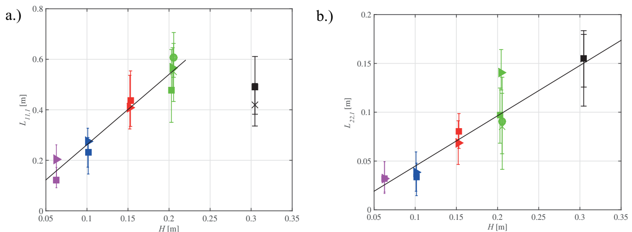
Figure 8. Smooth bed cases. (a) Mean streamwise integral length scale plotted against flow depth. Solid line: y = 2.79(x) - 0.02 , R^2 = 0.95 . (b) Mean transverse integral length scale plotted against flow depth. Solid line: y = 0.52(x) - 0.01 , R^2 = 0.96 . Error bars indicate the range of values across the channel. See caption in Figure 5 for explanation of symbols.
