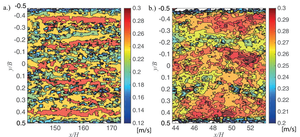
Figure 6. Instantaneous streamwise velocity contours. (a) Smooth bed experimental case H = 0.06 m, U_B = 0.23 m/s. (b) Smooth bed experimental case H = 0.20 m, U_B = 0.24 m/s.
