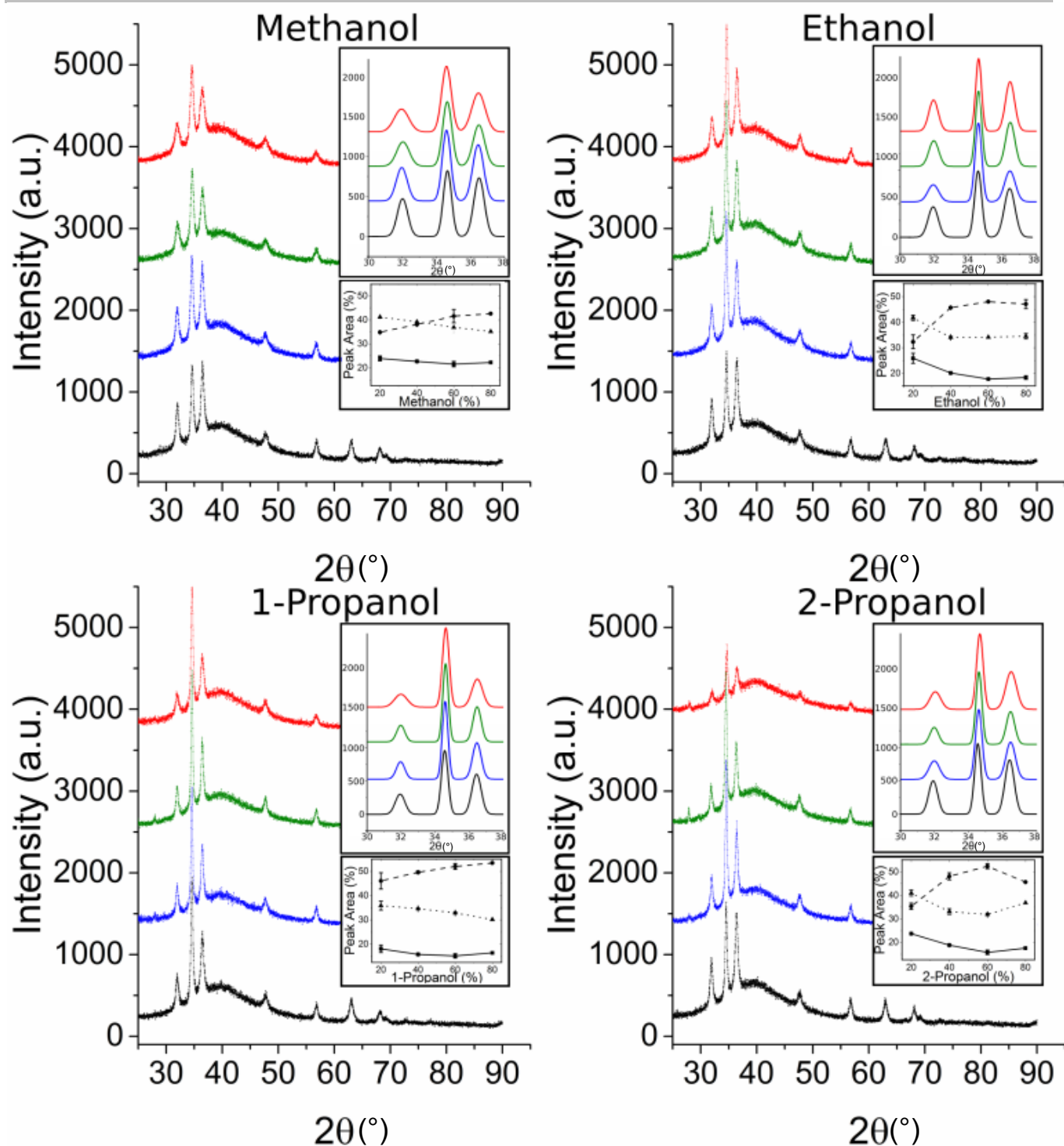
Figure 4. Wide-angle x-ray diffraction for zinc oxide – Nafion composites prepared with different binary solvent mixtures. The percent of alcohol in the binary mixtures are 20% (black), 40% (blue) 60% (green) and 80% (red). Top inset includes the fitted data for the low index planes corresponding to composites prepared at different concentrations of alcohol. Y-axis displays the intensity and is in a.u. The bottom inset plots the evolution of the three primary surface planes as a function of alcohol content. The lines correspond to the following planes: — {100}, - - {002} and ..... {101}.
