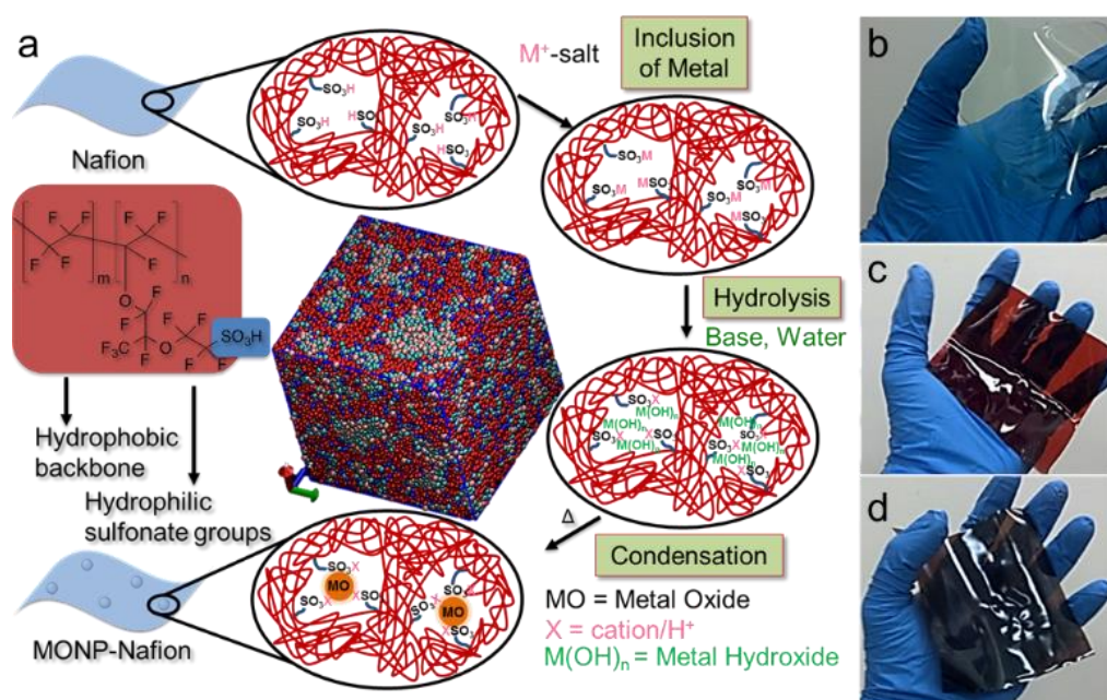
Scheme 1. (a) Schematic depicting the in situ growth of MONP within the polyelectrolyte membranes. Centerpiece is a snapshot of the nanoscale segregated structure in a hydrated Nafion membrane produced by the coarse-grained dissipative particle dynamics simulation (red is fluorinated alkene backbone, dark blue is the hydrophilic sulfonate groups, light blue is water, and pink is the counter cation). (b-d) Large scale MONP-Nafion composite films synthesized with nickel oxide, iron oxide and cobalt oxide, respectively.
