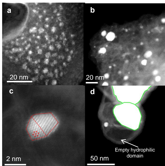
Figure 1. Scanning transmission electron microscopy (STEM) of in situ grown MONP within the polyelectrolyte membrane. (a) Dispersed MONP synthesized with NaOH. (b-d) MONP synthesized using \text{NH}_4\text{OH} . (b) MONP dispersed throughout the Nafion matrix. (c) An individual MONP outlined by a dashed red line with the {002} and {100} exposed crystal facets. The hexagonal packing is highlighted by red circles on the {002} plane. (d) The host hydrophilic growth domains with MONP grown inside, and evidence of twinning of adjacent MONP, outlined by green.
