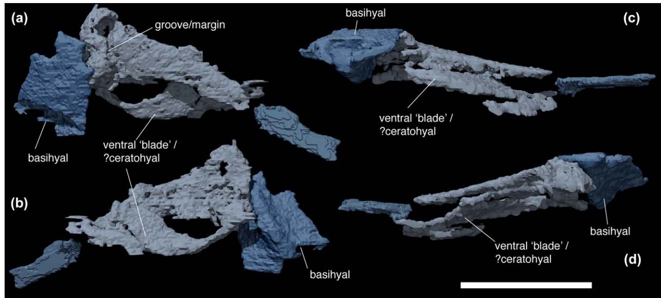
FIGURE 3 Paraplesiobatis , basihyal and first arch elements. Dorsal view (a). Ventral view (b). Posterior view (c). Anterior view (d). Scale bar = 1 cm
