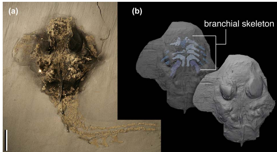
FIGURE 1 Paraplesiobatis specimen KGM 1983/294 (a) and virtual renderings of synchrotron light computed tomography showing solid (lower right) and transparent views (upper left) with branchial arches (b). Scale bar = 1 cm
