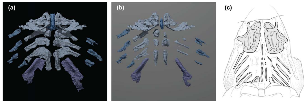
FIGURE 4 Alternative reconstructions of Paraplesiobatis and comparison with Pseudopetalichthys . Partially reconstructed gill skeleton with left and right first arch elements mirrored, and basihyal and posterior elements restored to approximate life condition (a). Reconstruction in panel A partially embedded in a virtual plane resulting in apparent segmented pattern (b). Reconstruction of Pseudopetalichthys (redrawn from Gross, 1962) with pharyngeal arch elements highlighted to show correspondence with Paraplesiobatis suggesting that the segmented appearance may be misleading (c). Not to scale
