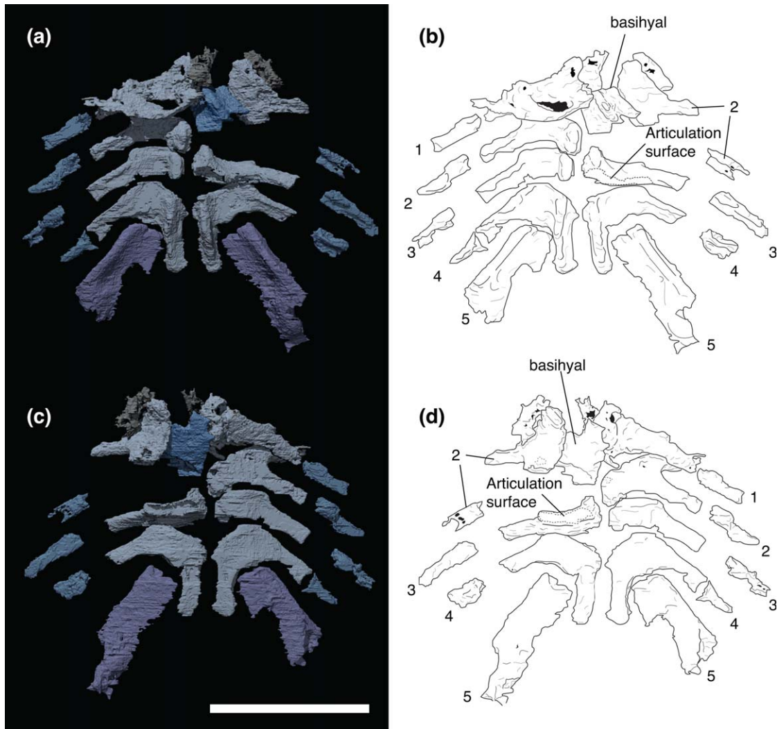
FIGURE 2 Paraplesiobatis , virtual renderings and interpretive illustrations of articulated gill skeleton of KGM 1983/294. Dorsal view (a, b), ventral view (c, d). Numbers indicate individual arch orders referred to in the text, but not necessarily direct homologies to other gnathostomes. Scale bar = 1 cm
