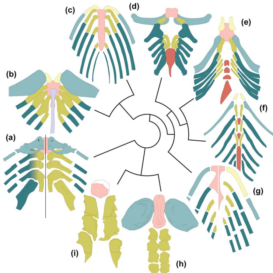
FIGURE 5 Phylogenetic comparison of ventral gill arch patterns in early jawed vertebrates. (a) Two possible interpretations of Paraplesiobatis . (b) Glyptolepis after Jarvik (1972). (c) Mimipiscis after Gardiner (1984). (d) Scapanorhynchus after Garman (1913). (e) Debeerius after Grogan and Lund (2000). (f) Ozarcus after Pradel et al. (2014). (g) Acanthodes after Miles (1973) (left), and Gardiner (1984) (right). (h) Cowralepis after Carr et al. (2009). (i) Tapinosteus after Stensiö (1969). Not to scale
