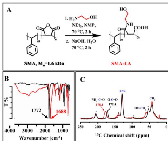
Figure 1. Synthesis and characterization of SMA-EA polymer: A) Reaction scheme for the modification of SMA polymer by an amination reaction. B) FT-IR spectra of SMA (black) and SMA-EA (red; US patent (filed)) polymers showing differences underlying the amination of maleic anhydride. C) ^{13}\text{C} CP-MAS NMR spectra of SMA (black) and SMA-EA (red) obtained under 8 kHz spinning further confirm the transformation of SMA to form the SMA-EA polymer; the spinning side bands are indicated by asterisks.
