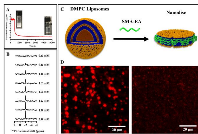
Figure 2. Formation of SMA-EA polymer based nanodiscs: A) Normalized static light scattering of DMPC MLVs upon the addition of SMA-EA polymer. The intense SLS signal observed at time zero ( t=0 ) due to light scattering by the large size MLVs decreases over time after the addition of SMA-EA. B) ^{31}\text{P}
