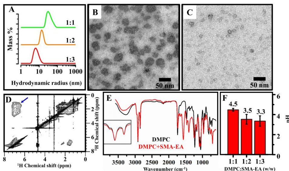
Figure 3. Characterization of SMA-EA polymer based macro and nanodiscs of DMPC bilayers: A) DLS profiles showing the different size nanodiscs obtained by varying the lipid to polymer molar ratio. TEM micrographs highlight the difference in the size of nanodiscs obtained by mixing 1:1 (B) or 1:3 (C) ratio of DMPC:SMA-EA (w/w). D) 2D NOESY spectrum of nanodiscs (~10 nm). Blue arrow shows the cross-peaks between styrene ring protons of the SMA-EA polymer and the CH 2 protons of DMPC acyl chains. E) FT-IR spectra of lyophilized DMPC MLVs (black) and nanodiscs containing a DMPC bilayer (red). F) Highest pH for which precipitation of SMA-EA polymer based DMPC lipid nanodiscs were observed by SLS experiments
