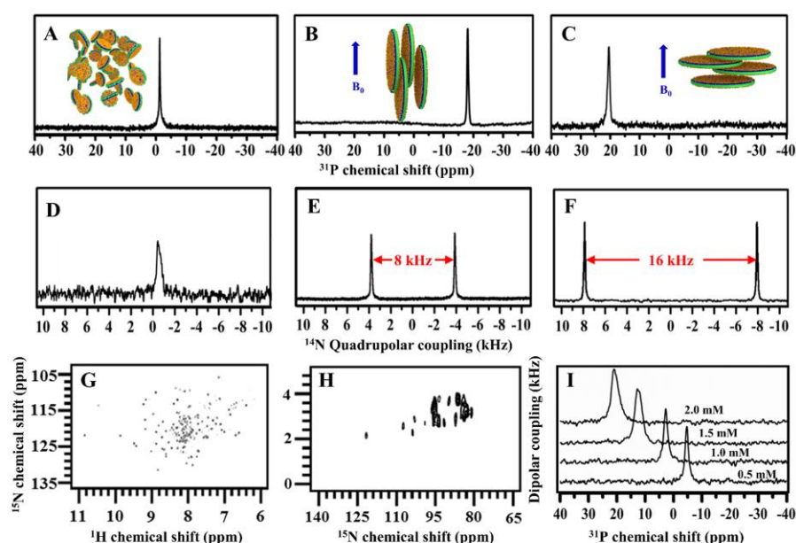
Figure 4. Magnetic-alignment of SMA-EA polymer based macro-nanodiscs: Static ^{31}\text{P} (A, B and C) and ^{14}\text{N} (D, E, and F) NMR spectra demonstrates the presence of isotropic nanodiscs (~10 nm diameter) (A, D), the magnetic-alignment of macro-nanodiscs (~50 nm) with the lipid bilayer perpendicular to the external magnetic field (B, E), and flipped macro-nanodiscs in the presence of \text{Yb}^{3+} ions with the lipid bilayer parallel to the external magnetic field (C, F). G) 2D ^{15}\text{N} - ^1\text{H} TROSY HSQC spectrum of isotropic SMA-EA nanodiscs containing ^{15}\text{N} -cytochrome- b_5 reconstituted in DMPC lipid bilayers. All spectra were recorded at 35 °C, where the DMPC lipids are in a fluid lamellar phase bilayer. H) 2D ^1\text{H} - ^{15}\text{N} PISEMA spectrum of SMA-EA macro-nanodiscs containing ^{15}\text{N} -cytochrome- b_5 reconstituted in DMPC lipid bilayers with the bilayer normal perpendicular to the external magnetic field. I) ^{31}\text{P} static NMR spectra of macro-nanodiscs with varying concentration of \text{YbCl}_3 .
