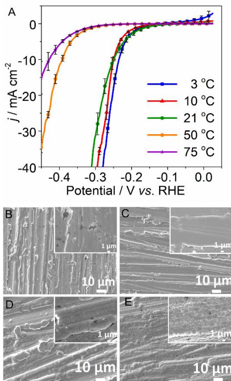
Figure 7. (A) Polarization data in 0.5 M H 2 SO 4 for Ni-P (Brenner) films electrodeposited at different temperatures of 3 °C (blue), 10 °C (red), 21 °C (green), 50 °C (orange) and 75 °C (purple); scan rate is 5 mV s -1 . The values represent the mean ± SD based on 3 independent experiments. (B-E) SEM images of Ni-P (Brenner) films electrodeposited at varied temperatures of (B) 3 °C, (C) 10 °C, (D) 50 °C, (E) 75 °C. The insets are further zoomed in SEM images.
