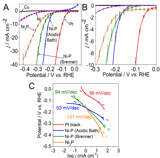
Figure 2. (A) Polarization data and (B) an inset of the polarization curves for electrodeposited Pt black (red), Ni-P (Acidic Bath) (blue), Ni-P (Brenner) (green), commercial Ni 2 P (orange) Ni (Watts) (purple) films and blank copper foil (black) in 0.5 \text{ M H}_2\text{SO}_4 ; scan rate is 5 \text{ mV s}^{-1} . The inset shows the polarization data at the initial stage (from 0 \text{ V} to -0.3 \text{ V} vs. RHE) of the electrolysis. The values represent the mean \pm standard deviation (SD) based on 3 independent experiments. (C) Corresponding Tafel plots (with linearly fitted dashed lines) derived from the polarization curves.
