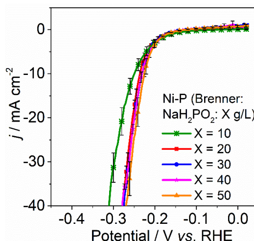
Figure 8. Polarization data in 0.5 M H 2 SO 4 for Ni-P (Brenner) films electrodeposited with varied concentration of NaH 2 PO 2 in the plating bath. Ni-P (Brenner: X g/L): (X=10 (green), 20 (red), 30 (blue), 40 (pink) and 50 (orange)); scan rate is 5 mV s -1 . The values represent the mean ± SD based on 3 independent experiments.
