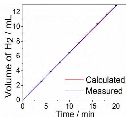
Figure 3. Volume of \text{H}_2 generated on Ni-P (Brenner) films when a current of 85.4 \text{ mA} is passed over 20 minutes in 0.5 \text{ M H}_2\text{SO}_4 versus calculated quantities assuming 100% Faradaic efficiency for the HER. The values represent the mean \pm SD based on 3 independent experiments.
