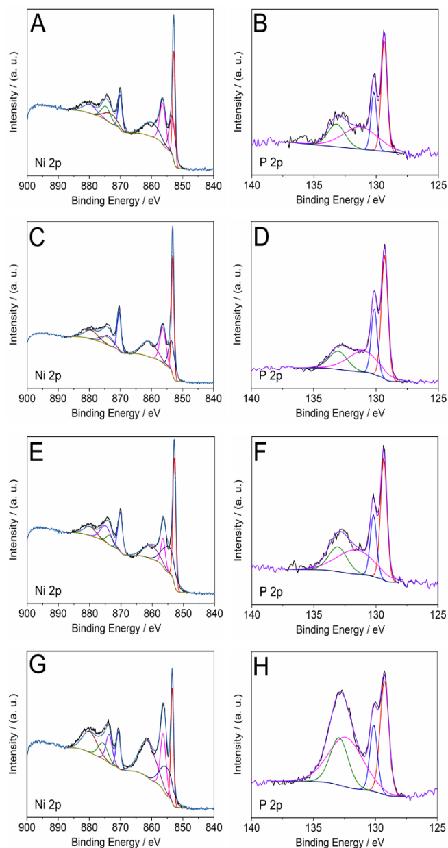
Figure 5. XPS spectra of the Ni 2p and P 2p regions for (A and B) as-deposited Ni-P (Brenner), (C and D), Ni-P (Brenner) after 5000 cyclic voltammetric sweeps in 0.5 M H 2 SO 4 , (E and F) as-deposited Ni-P (Acidic Bath), (G and H), Ni-P (Acidic Bath) after 5000 cyclic voltammetric sweeps in 0.5 M H 2 SO 4 .
