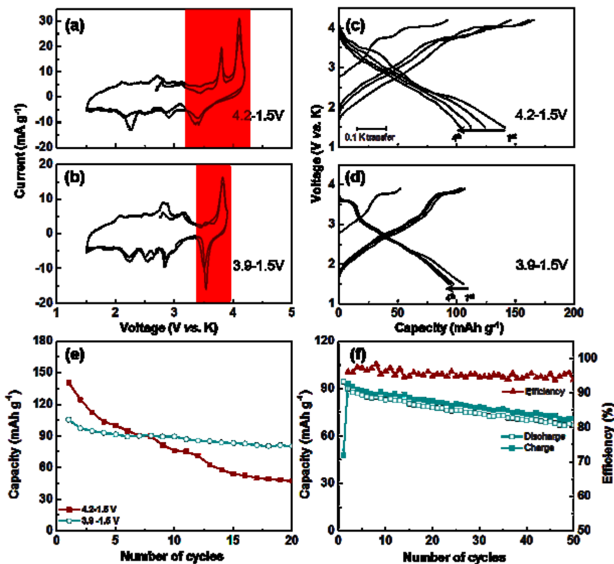
Figure 2. K-storage properties of P3- \text{K}_{0.5}\text{MnO}_2 . (a–b) Cyclic voltammograms at a scan rate of 0.03 \text{ mV sec}^{-1} and (c–d) galvanostatic voltage–capacity profiles of P3-type \text{K}_{0.5}\text{MnO}_2 with two different voltage cutoffs. (e) Discharge capacity of P3-type \text{K}_{0.5}\text{MnO}_2 over 20 cycles with the two different voltage cutoffs at a current rate of 5 \text{ mA g}^{-1} . (f) Cycle stability and coulombic efficiency (of the 1 st discharge) of P3-type \text{K}_{0.5}\text{MnO}_2 at a current rate of 20 \text{ mA g}^{-1} in the range of 3.9–1.5 V (vs. \text{K}/\text{K}^+ ).
