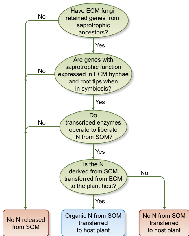
Fig. 1 Set of minimum conditions necessary for the liberation of organic nitrogen (N) from soil organic matter (SOM) by ectomycorrhizal fungi (ECM). See full text for explanation.
