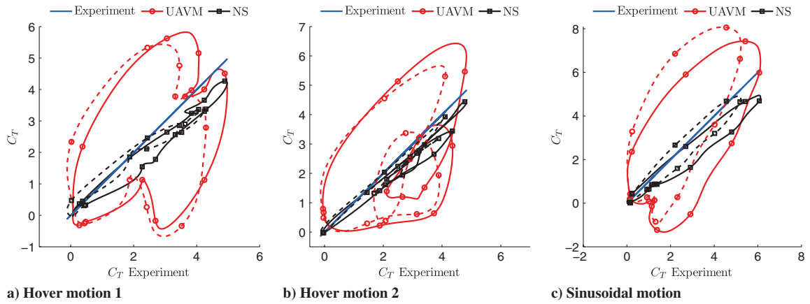
Fig. 8 Correlation plot of the force coefficients of all three motions. The solid lines and dashed lines represent the up and down-stroke respectively.
