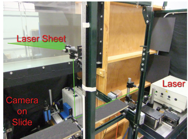
Fig. 3 Representation of the PIV setup parallel to the water surface.
