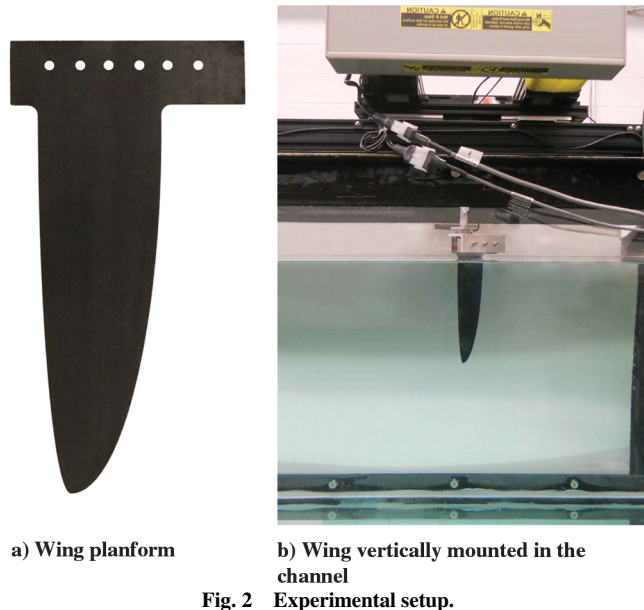
Fig. 2 Experimental setup.
