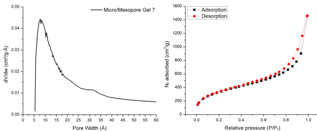
Figure 4. a. Micro/mesoporosimetry BJH/Horvath-Kawazoe differential pore volume plot for gel 7 at 0 \leq p/p_0 \leq 0.1 showing peak pore size of \sim 1.0 nm, b. BET mesopore analysis of gel 7 showing N_2 adsorption up to 1500 cm^3/g with a type II shape and H3 hysteresis loop with slit-like pores. 40
