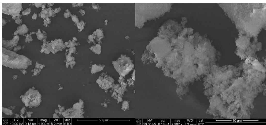
Figure 3. SEM images of gel 7 at 2x and 8x magnification.
