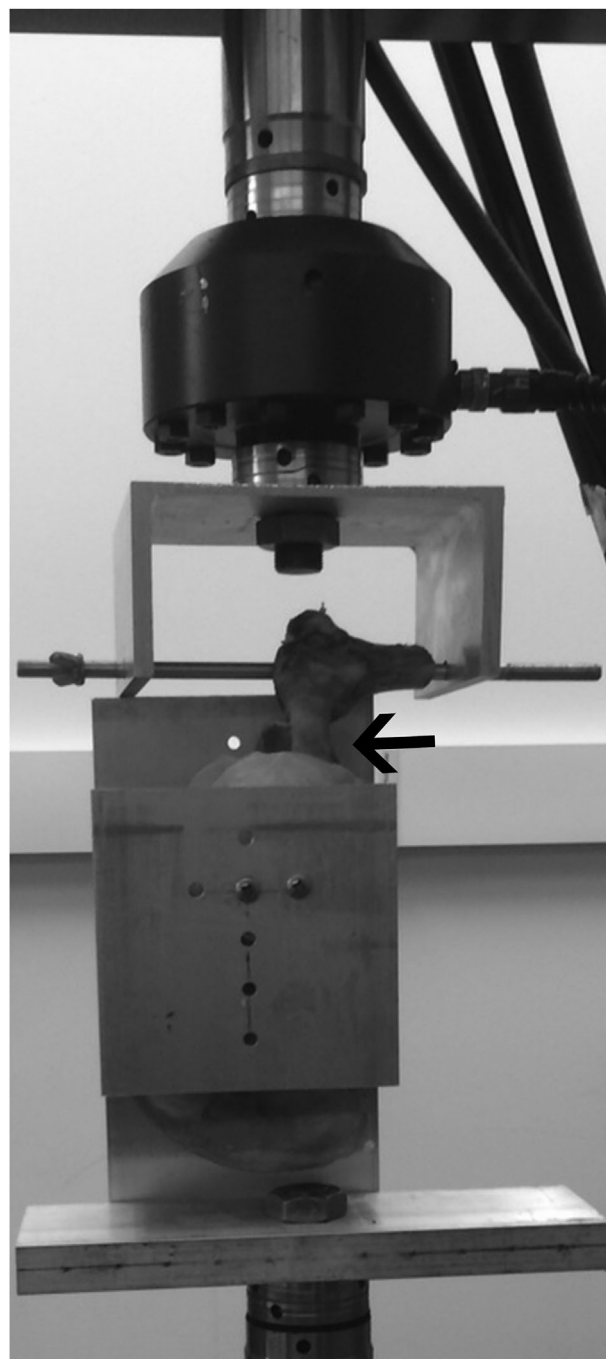
Figure 3. Custom-made grip design with humerus and scapula mounted uniaxially to the MTS. Arrow points to infraspinatus tendon.
