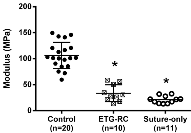
Figure 6. Rotator Cuff Stiffness. (*) Denotes significance p \leq 0.05 compared to control shoulder. Error bars represent \pm SD.
