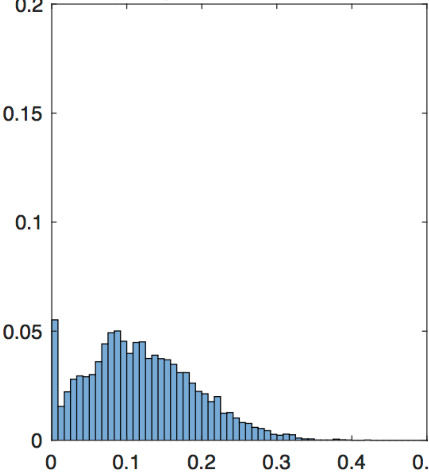
Perfectly Negatively Correlated, rho=-1
