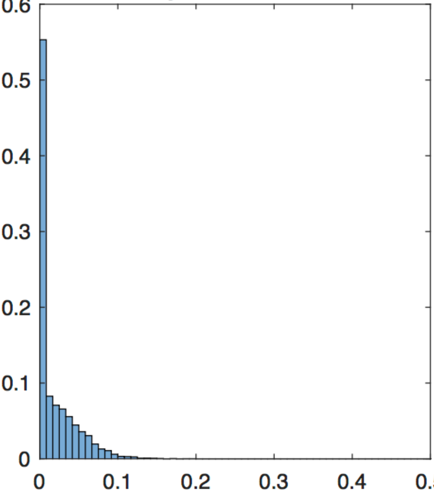
Positively Correlated, rho=0.5
