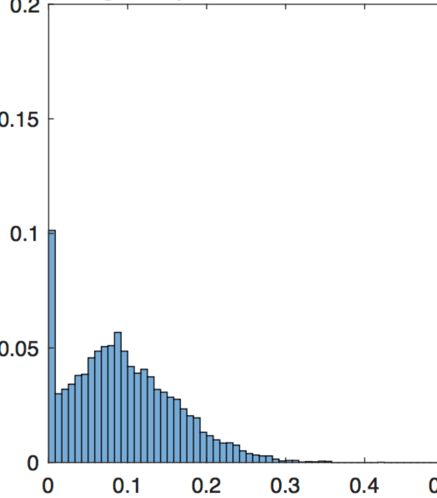
Negatively Correlated, rho=-0.5
