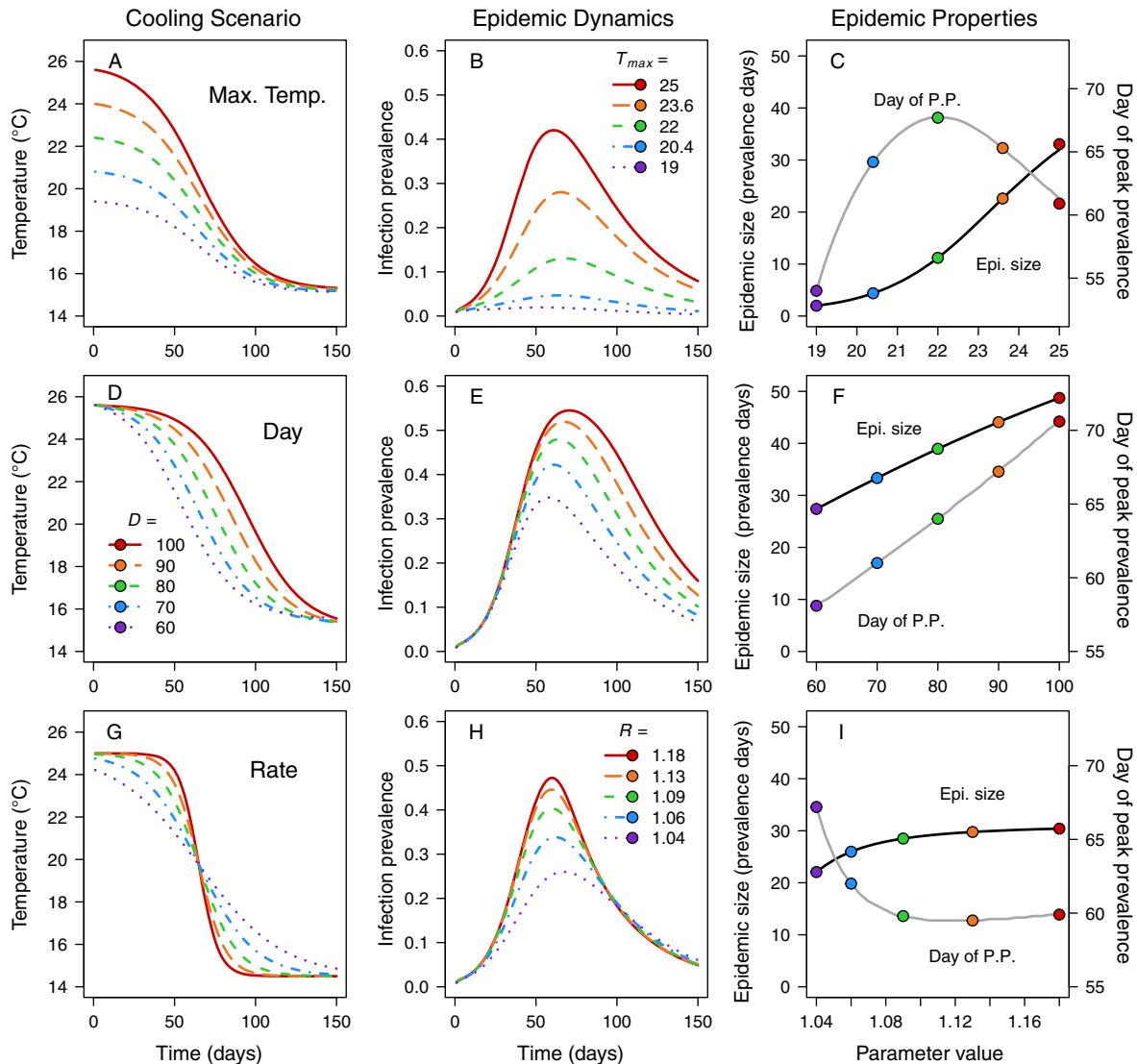
FIG. 5. Simulated epidemics with multiple scenarios of seasonal cooling and all traits as temperature-dependent functions. Top row varies starting temperature ( T_{max} ), middle row varies start date of cooling ( D ), and bottom row varies cooling rate ( R ). Left column shows five cooling scenarios, middle column shows corresponding epidemic dynamics, and right column shows how two epidemic properties (size and date of peak prevalence) vary with each parameter. Points in the right column correspond to the five examples in the first two columns. Parameters values decrease as lines become less solid and colors become more cool (i.e., red > orange > green > blue > purple). (A, B, C) Starting temperature, T_{max} : epidemics are larger with hotter starting temperatures. Epidemics reach peak prevalence later at intermediate starting temperatures. (D, E, F) Start date of cooling: epidemics are larger and peak later as start date of cooling moves later in the season. (G, H, I) Cooling rate, R : epidemic properties are relatively stable with varying cooling rates. Base cooling parameters: T_{max} = 25^{\circ}\text{C} , D = 70 , R = 1.06 , and T_{min} = 15^{\circ}\text{C} .
