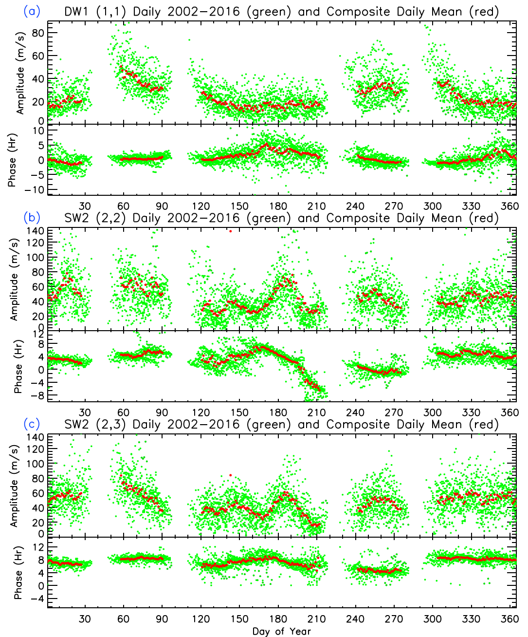
Figure 3. Thermosphere-Ionosphere-Mesosphere Energetic and Dynamics Doppler Interferometer DW1 (1,1)(a), SW2 (2,2) (b), and SW2 (2,3) (c) daily and composite mean amplitudes and phases from 2002 to 2016. Note that SW2 (2,2) and (2,3) mode phases are wrapped to avoid unwanted discontinuities.
