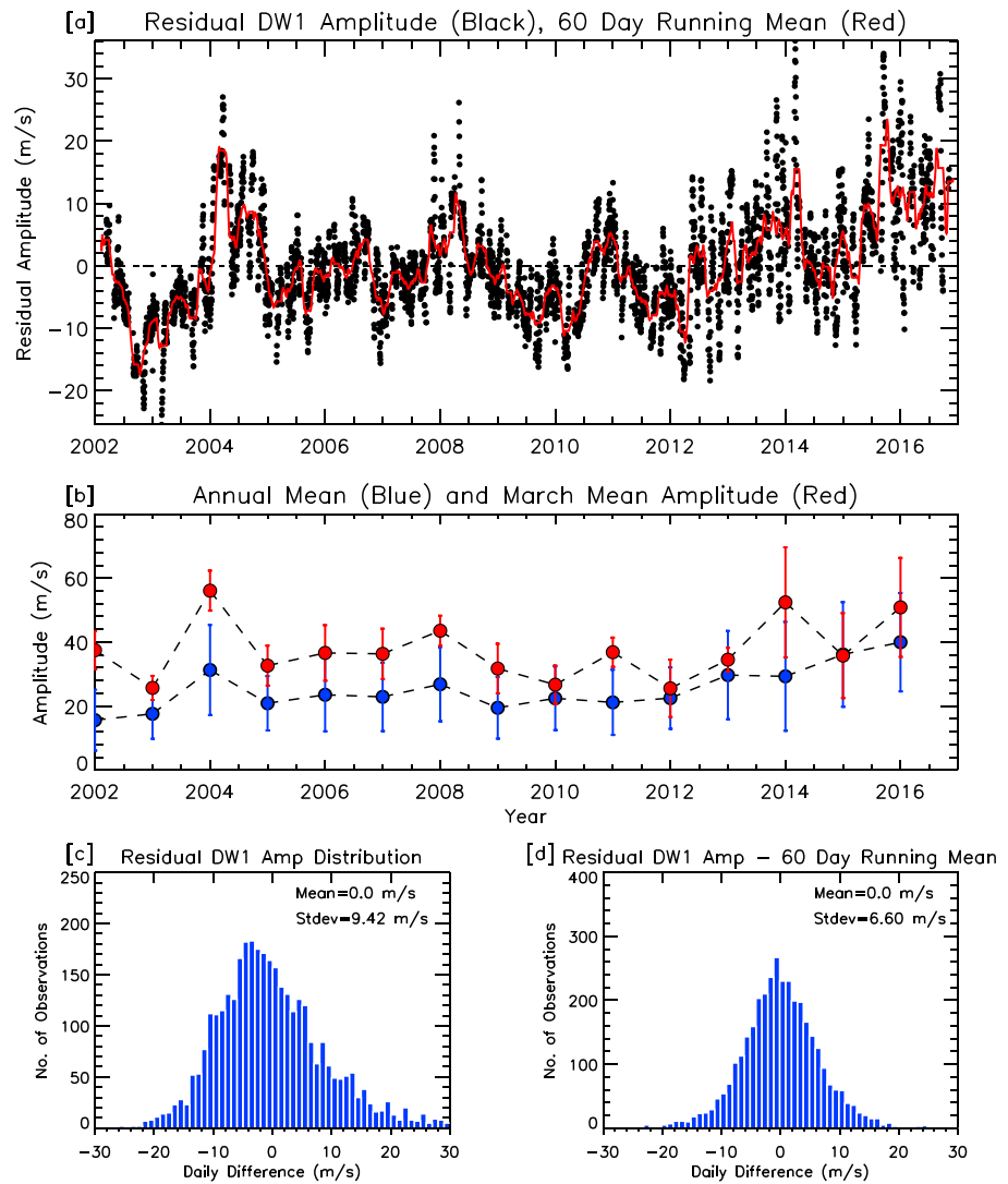
Figure 6. (a) TIDI DW1 (1,1) mode residual amplitude and 60-day running mean time series from 2002 to 2016, (b) TIDI DW1 annual and March mean amplitude. The error bars denote the standard deviation of the estimated tidal amplitudes, (c) histogram of residual amplitude shown in (a), and (d) residual amplitude after removing 60-day running mean (shown in a).
