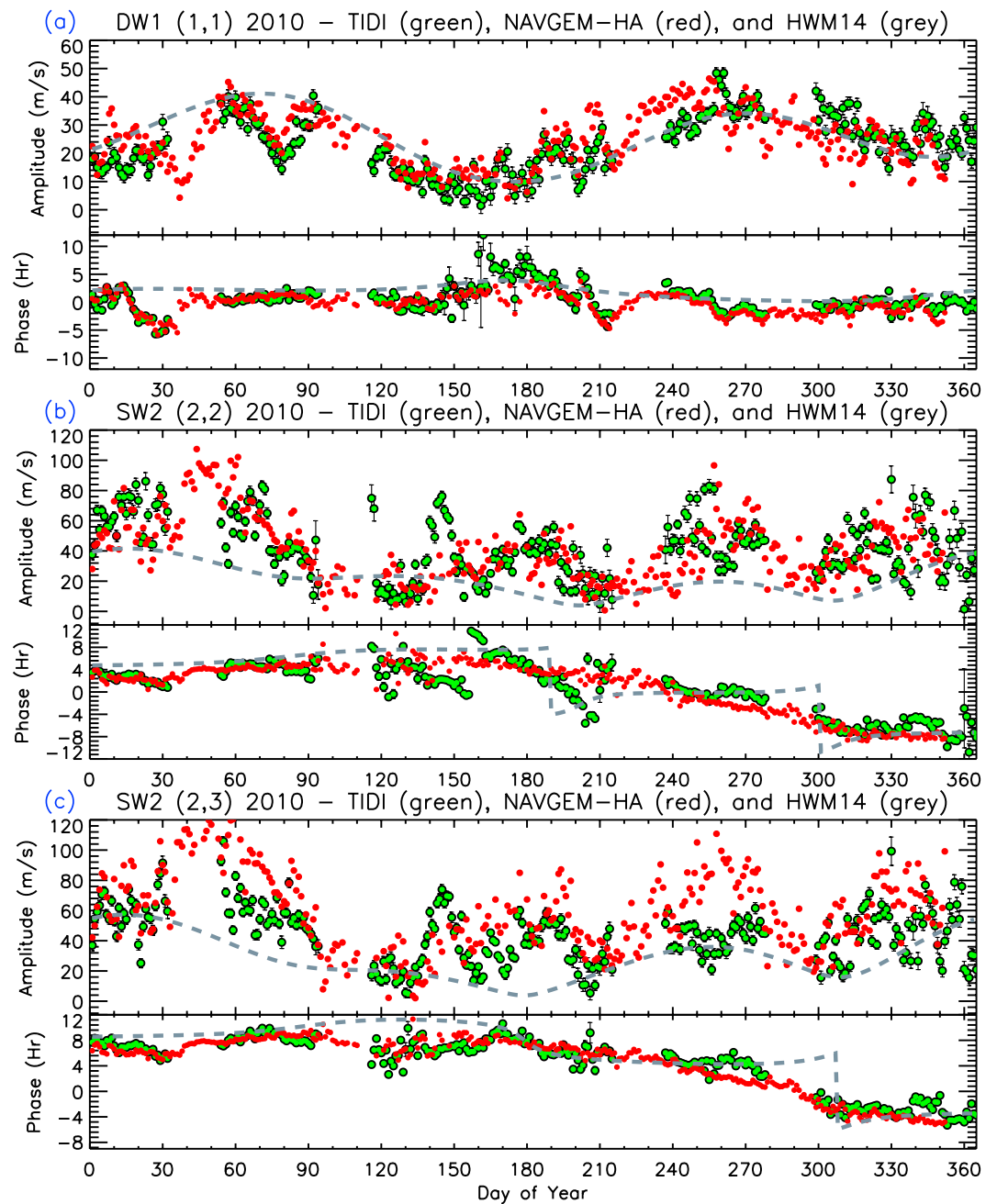
Figure 2. DW1 (1,1)(a), SW2 (2,2) (b), and SW2 (2,3) (c) tidal mode amplitudes and phases estimated from TIDI (green), NAVGEM-HA (red), and HWM14 (gray) meridional winds during 2010. Amplitude refers to maximum value, while phase refers to the local solar time of the maximum value. Error bars denote the \pm 1\sigma uncertainty estimate. Note that SW2 (2,2) and (2,3) mode phases are wrapped to avoid unwanted discontinuities. TIDI = TIMED Doppler Interferometer; NAVGEM-HA = Navy Global Environmental Model-High Altitude version; HWM14 = Horizontal Wind Model.
