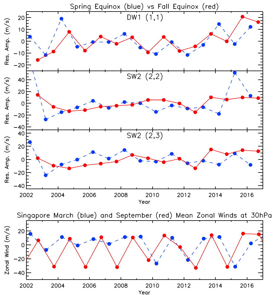
Figure 5. (top) Comparison of TIDI DW1 (1,1), SW2 (2,2), and SW2 (2,3) mode amplitude residuals for spring equinox (day number 60–100, blue) and fall equinox (day number 230–290, red). (bottom) March (blue) and September (red) monthly mean stratospheric zonal winds at 30 hPa from Singapore.
