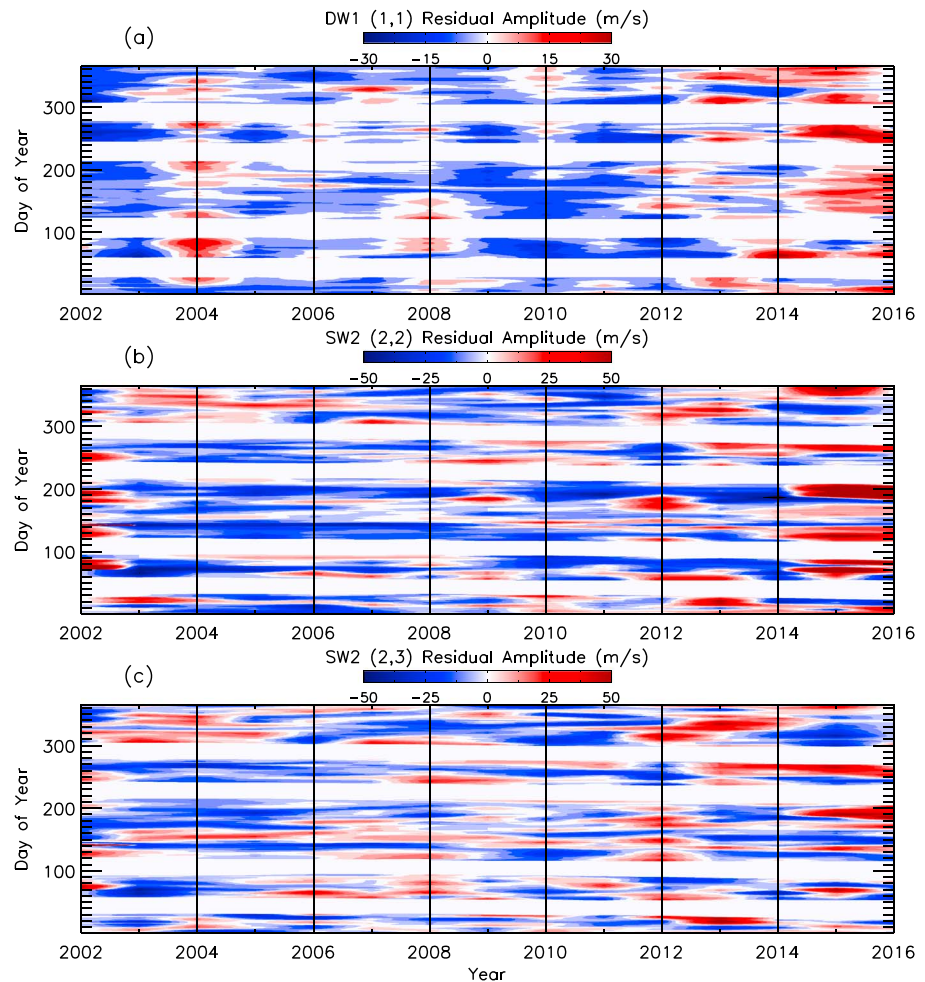
Figure 4. TIDI DW1 (1,1)(a), SW2 (2,2) (b), and SW2 (2,3) (c) residual amplitude (= daily amplitude minus composite daily mean amplitude) contours as a function of year and day of year. Note that x axis represent interannual variability and y axis present intra-annual variability.
