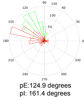
D Phase means by cell class: 50-200Hz Broadband gamma
