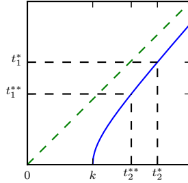
Figure 3: Schematic sketch of t_1^* as a function of t_2^*
