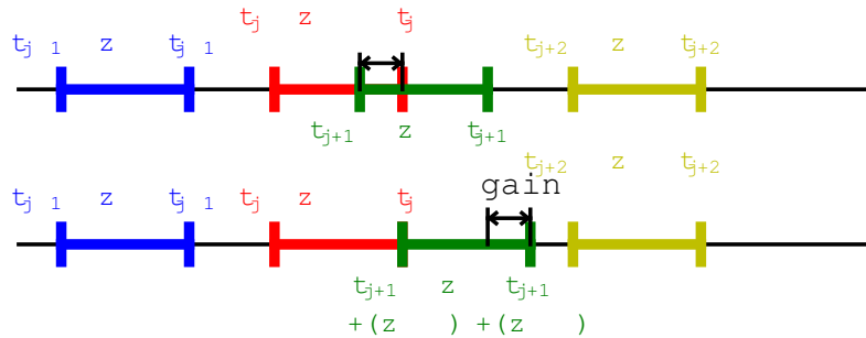
Figure 2: Schematic sketch for Eq. 12
