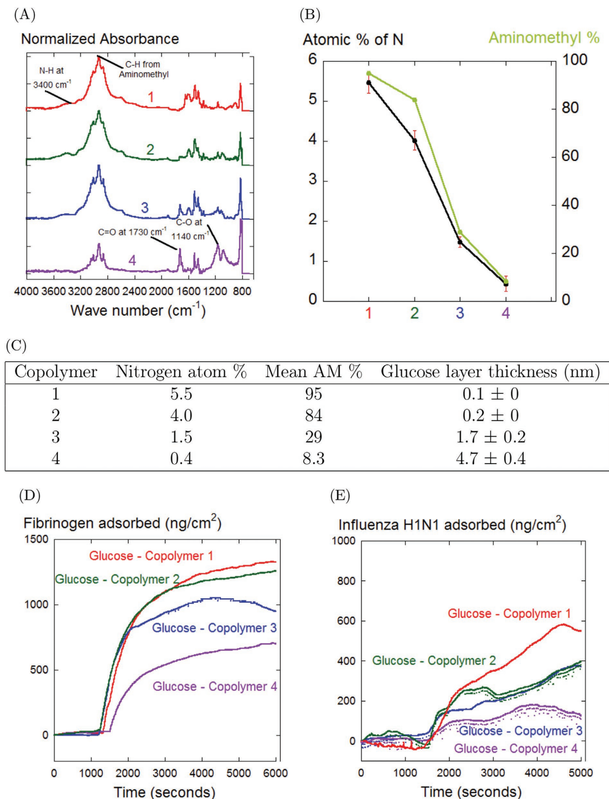
Figure 3. Four sets of copolymers (1-red, 2-green, 3-blue, 4-purple) with different concentrations of aminomethyl (AM) and ester bromide (EB) groups were prepared. A) FTIR and B) XPS measurements together verified that the AM concentration decreased progressively from copolymer 1 to 4. Conversely, the EB content increased as shown by the growing intensity of the carbonyl band. C) Ellipsometric thicknesses of glucose polymers grafted from the copolymer coatings. QCM traces of D) fibrinogen and E) influenza indicate that the adsorption levels of both the protein and the virus particles are correlated with the AM density.
