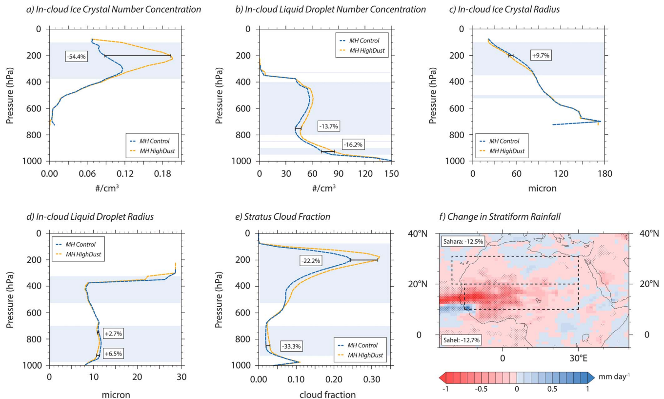
Figure 2. June, July, August, September Saharan-average atmospheric profiles for (a) in-cloud ice crystal number concentration, (b) in-cloud liquid droplet number concentration, (c) in-cloud ice crystal radius, (d) in-cloud liquid droplet radius, (e) stratus cloud fraction, and (f) spatial map of stratiform rainfall difference between MH Control and MH HighDust . Atmospheric profile and spatial map description same as Figure 1. “In-cloud” variables are calculated by dividing the specified cloud variable (e.g., ice crystal number concentration) by its fractional occurrence. Calculated differences for profile levels are shown as follows: (a) 200, (b) 750 and 925, (c) 200, (d) 750 and 925, and (e) 200 and 850 hPa.
