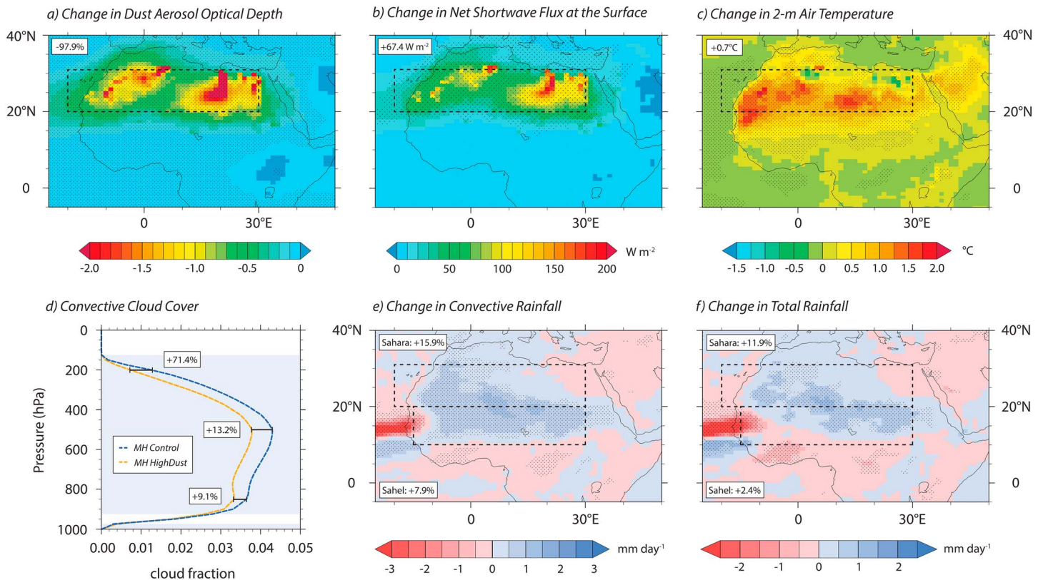
Figure 1. June, July, August, September differences between MH Control and MH HighDust in (a) dust aerosol optical depth, (b) net surface shortwave radiation flux diagnosed from offline radiation calculations, (c) 2-m air temperature, (d) profile of convective cloud cover averaged over the Sahara, (e) convective rainfall, and (f) total rainfall. In spatial maps, dashed boxes signify Saharan (upper) and Sahel (lower in (e)–(f)) extent used to calculate percent changes noted in left corner(s) of each panel. Numbers in atmospheric profile represent the percent change in cloud fraction at specific atmospheric levels (850, 500, and 200 hPa). Stippling in spatial maps and shading in the atmospheric profile indicate statistically significant differences at the 95% confidence level.
