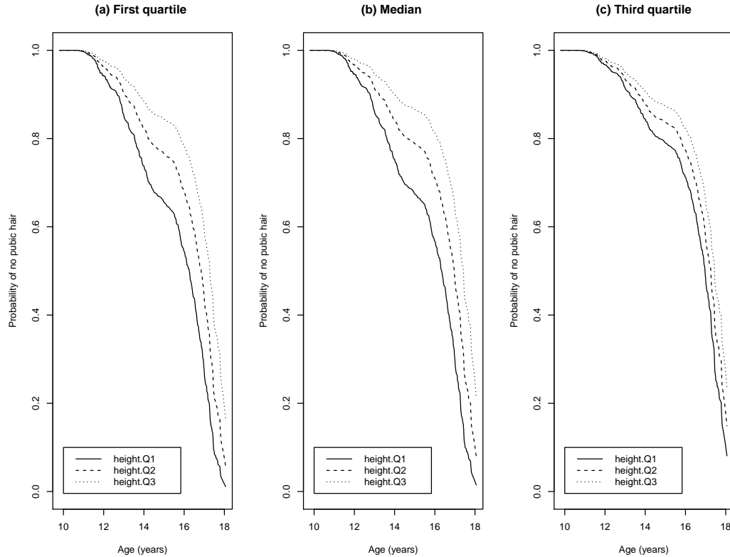
FIGURE 2: Analyzing the pubertal development study. Estimated survival functions for the three height groups with a fixed exposure to mixtures of phthalates m_k , k = 1, 2, 3 at the first quartile, median, and third quartiles of mixture m = \alpha_{31}X_1 + \alpha_{32}X_2 + \alpha_{33}X_3 . The height groups correspond to girls with a height equal to the first quartile (solid line), median (dashed line), or third quartile (dotted line), and an average value for maternal parity.
