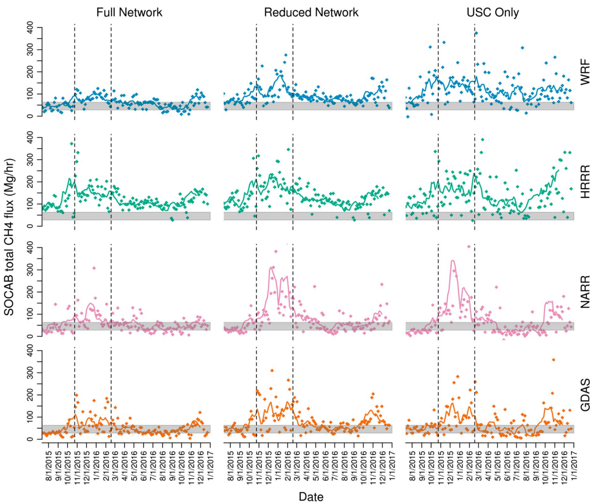
Figure 2. (points) Estimated total CH 4 flux time series for the SoCAB, at 4-day time intervals, according to inversions using transport driven by each of four meteorological models and using the full observing network (nine sites), a reduced network (three sites), or a single observing site. (curves) The 28-day running means of each time series for visual reference (not used in the analysis). The shaded band indicates the typical range of estimates in past studies. The dashed vertical lines indicate the start and end dates of the Aliso Canyon natural gas leak. SoCAB = South Coast Air Basin; WRF = Weather Research and Forecasting; HRRR = High-Resolution Rapid Refresh; NARR = North American Regional Reanalysis; GDAS = Global Data Assimilation System.
